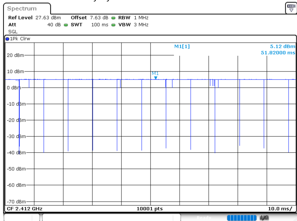
Duty Cycle NVHT 802.11b 2412MHz
