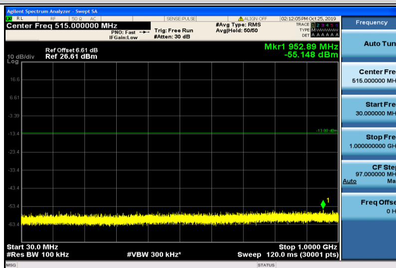
Band4-15MHz-16QAM-20025-1RB#0-30~1000MHz
