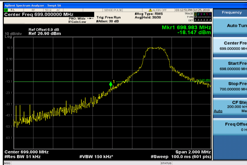
Band12-5MHz-QPSK-23035-1RB#0
