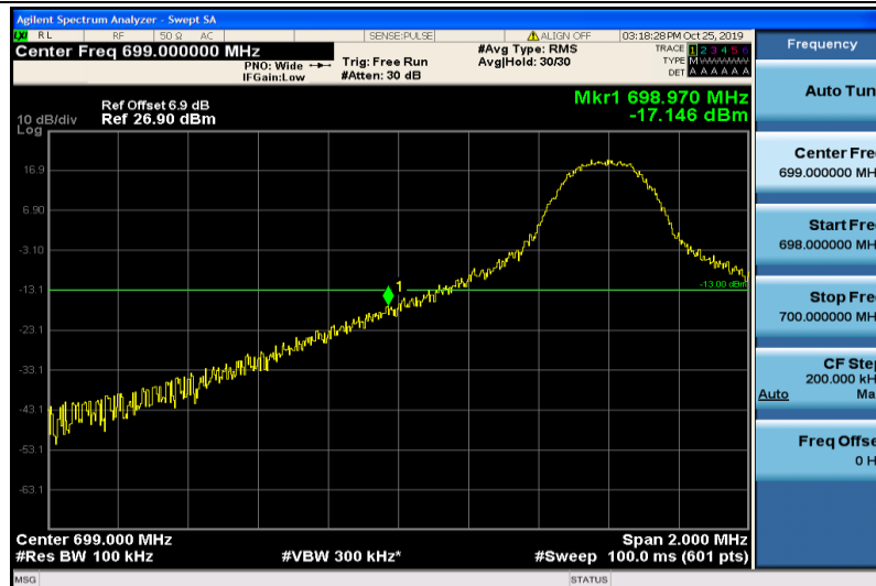
Band12-10MHz-16QAM-23060-1RB#0
