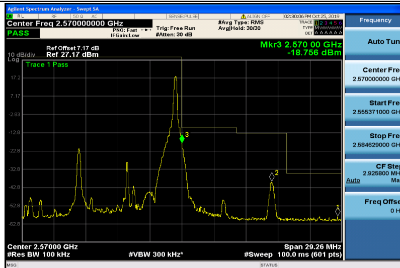
Band7-10MHz-16QAM-21400-1RB#49
