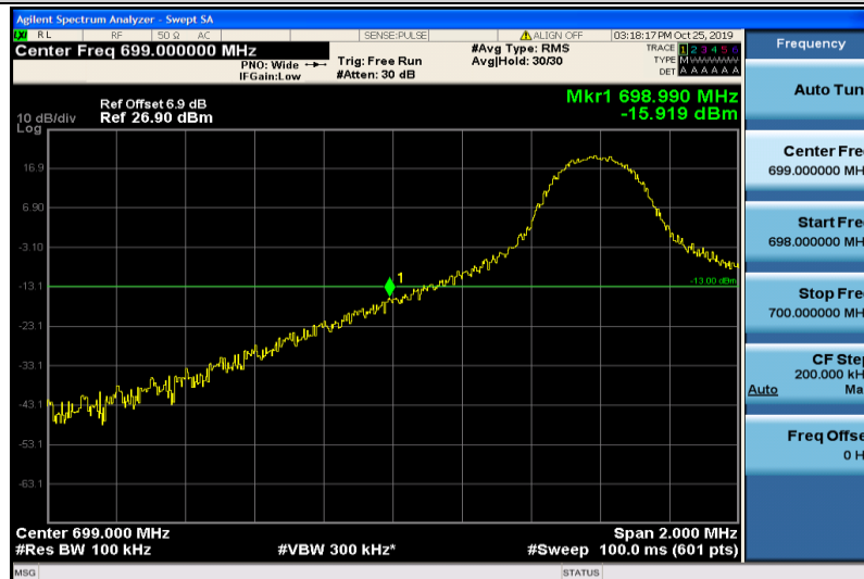
Band12-10MHz-QPSK-23060-1RB#0
