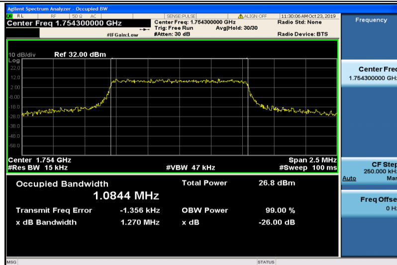
Band4-1.4MHz-16QAM-20393-6RB#0-1.0844
