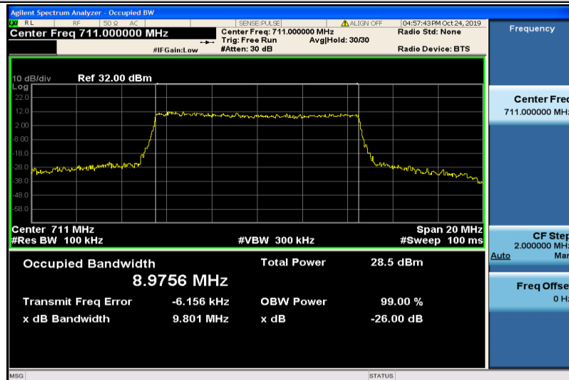
Band12-10MHz-16QAM-23130-50RB#0-8.9756
