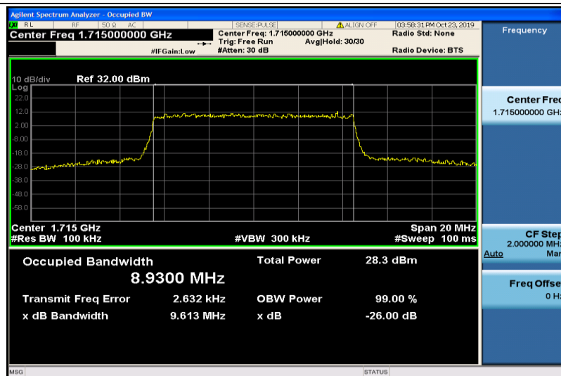
Band4-10MHz-16QAM-20000-50RB#0-8.9300
