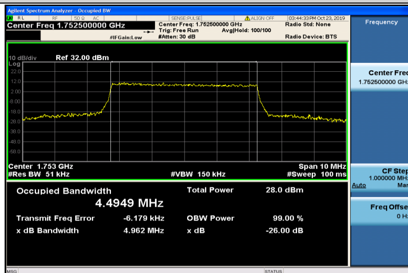
Band4-5MHz-16QAM-20375-25RB#0-4.4949
