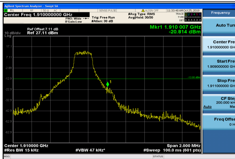
Band2-1.4MHz-16QAM-19193-1RB#5
