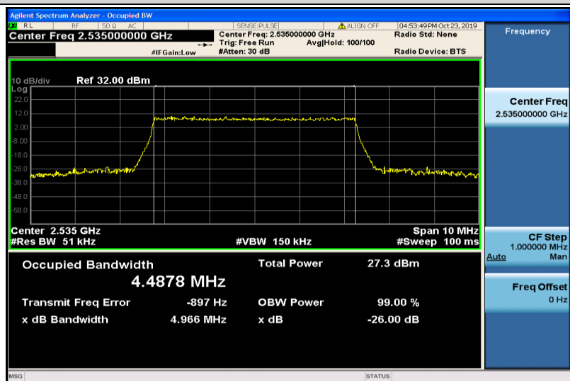
Band7-5MHz-16QAM-21100-25RB#0-4.4878
