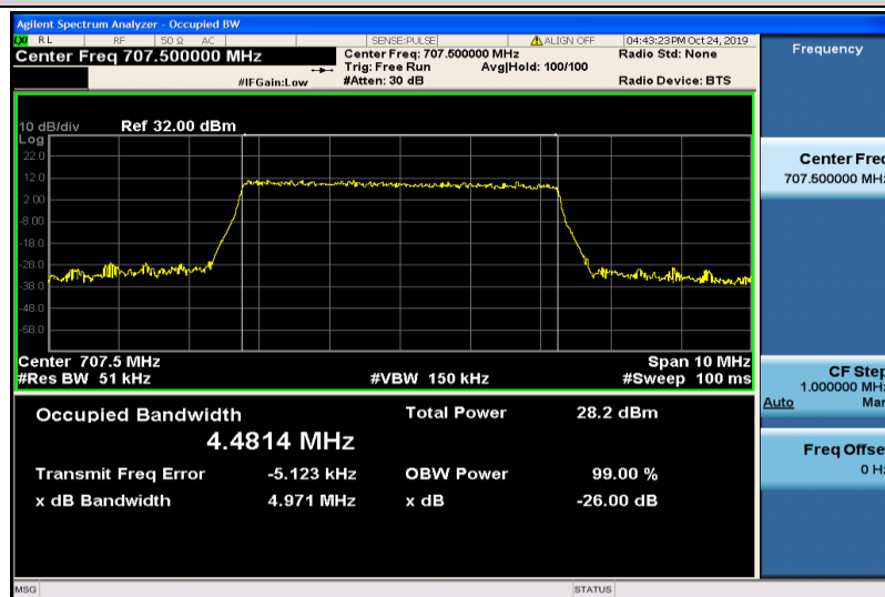
Band12-5MHz-16QAM-23095-25RB#0-4.4814
