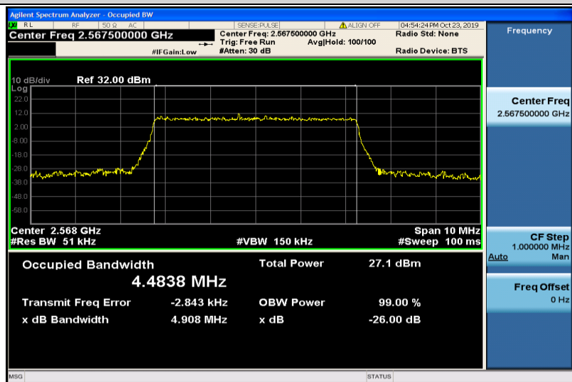
Band7-5MHz-16QAM-21425-25RB#0-4.4838
