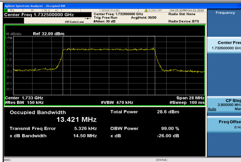
Band4-15MHz-16QAM-20175-75RB#0-13.421
