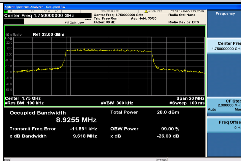
Band4-10MHz-16QAM-20350-50RB#0-8.9255
