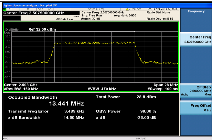
Band7-15MHz-QPSK-20825-75RB#0-13.441
