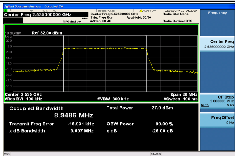
Band7-10MHz-16QAM-21100-50RB#0-8.9486
