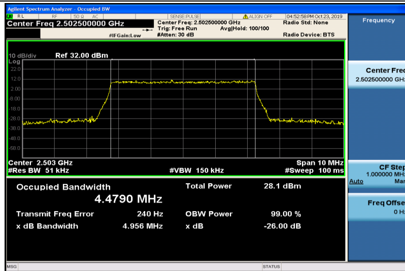
Band7-5MHz-QPSK-20775-25RB#0-4.4790
