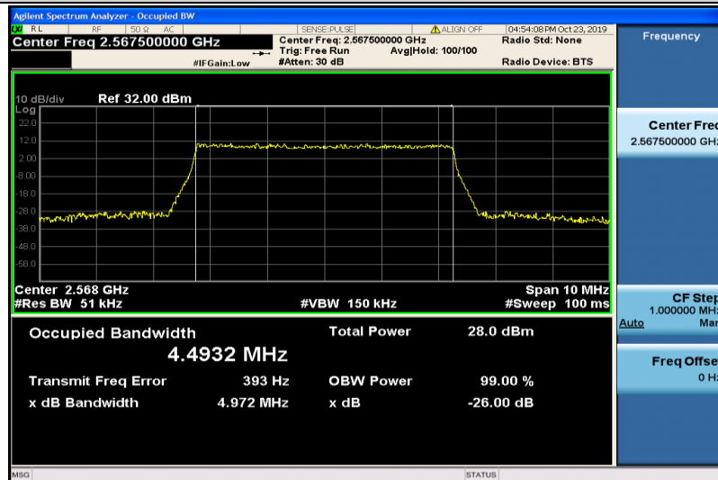
Band7-5MHz-QPSK-21425-25RB#0-4.4932
