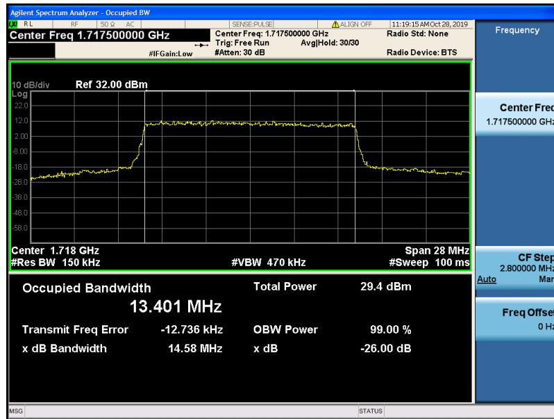
Band4-15MHz-QPSK-20025-75RB#0-13.401
