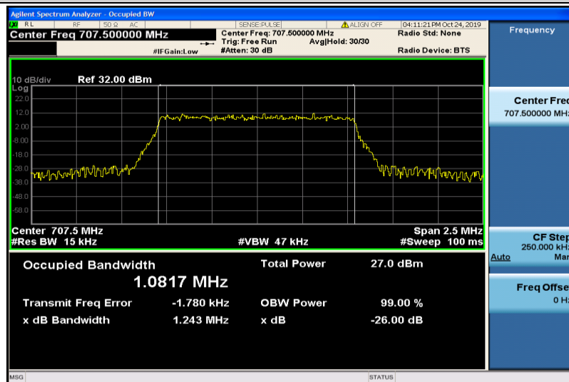
Band12-1.4MHz-16QAM-23095-6RB#0-1.0817
