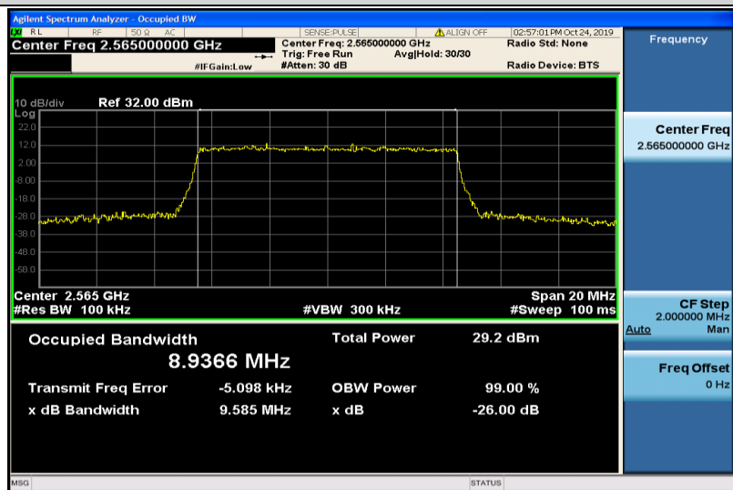
Band7-10MHz-QPSK-21400-50RB#0-8.9366
