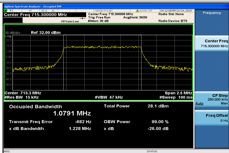
Band12-1.4MHz-QPSK-23173-6RB#0-1.0791
