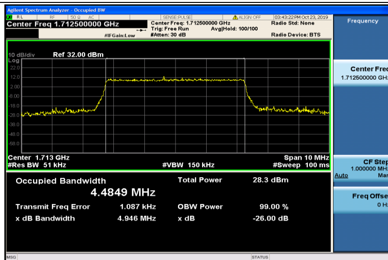
Band4-5MHz-16QAM-19975-25RB#0-4.4849
