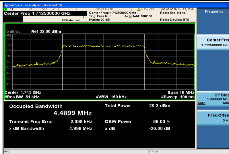
Band4-5MHz-QPSK-19975-25RB#0-4.4899
