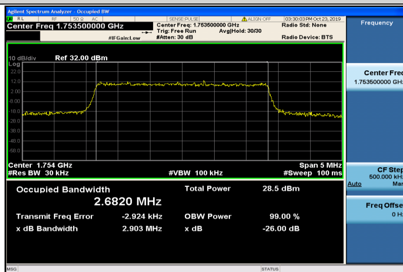
Band4-3MHz-QPSK-20385-15RB#0-2.6820
