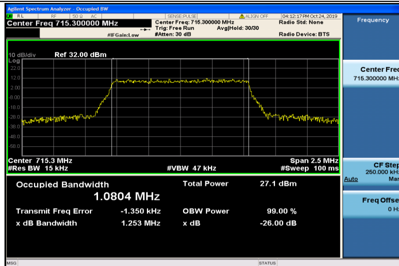
Band12-1.4MHz-16QAM-23173-6RB#0-1.0804
