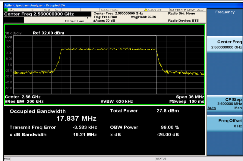
Band7-20MHz-16QAM-21350-100RB#0-17.837
