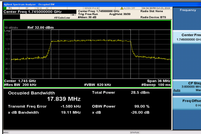
Band4-20MHz-16QAM-20300-100RB#0-17.839
