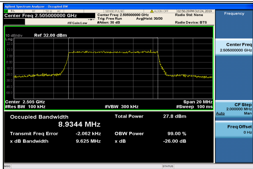
Band7-10MHz-16QAM-20800-50RB#0-8.9344
