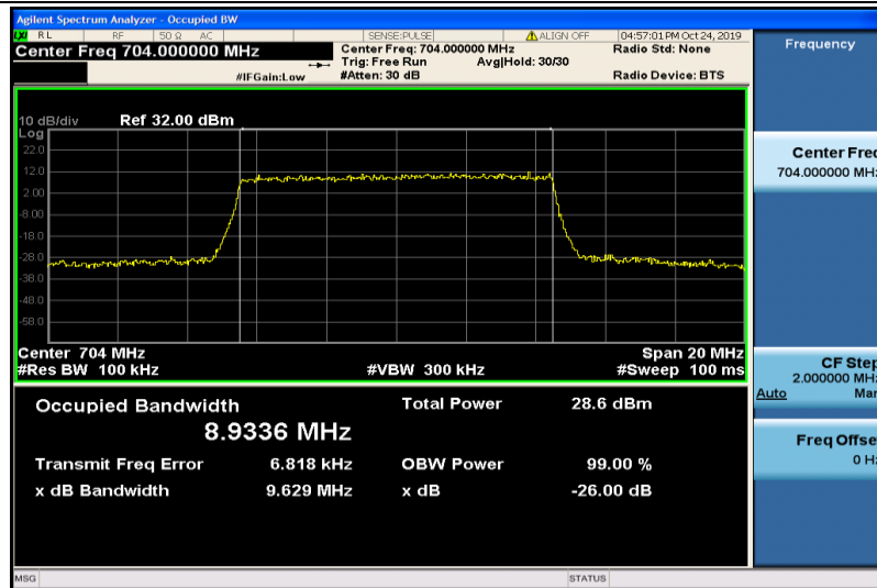
Band12-10MHz-16QAM-23060-50RB#0-8.9336
