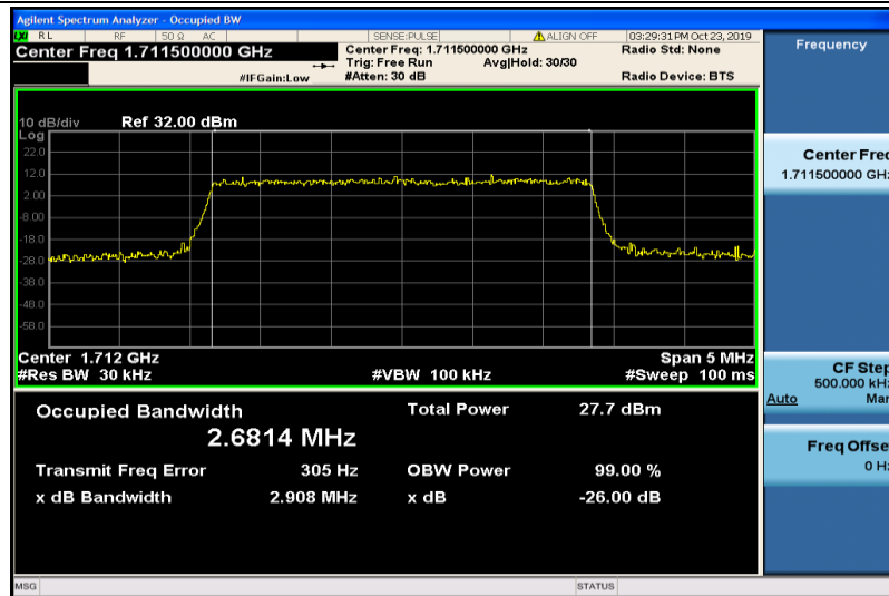
Band4-3MHz-16QAM-19965-15RB#0-2.6814
