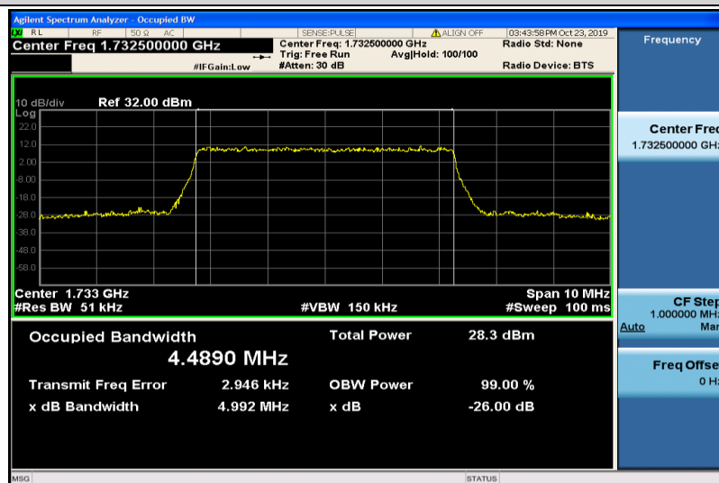
Band4-5MHz-16QAM-20175-25RB#0-4.4890
