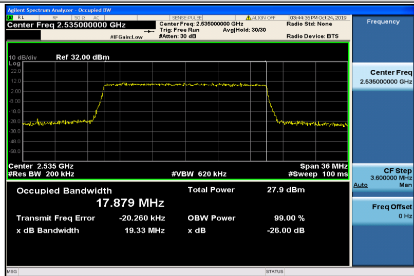
Band7-20MHz-16QAM-21100-100RB#0-17.879
