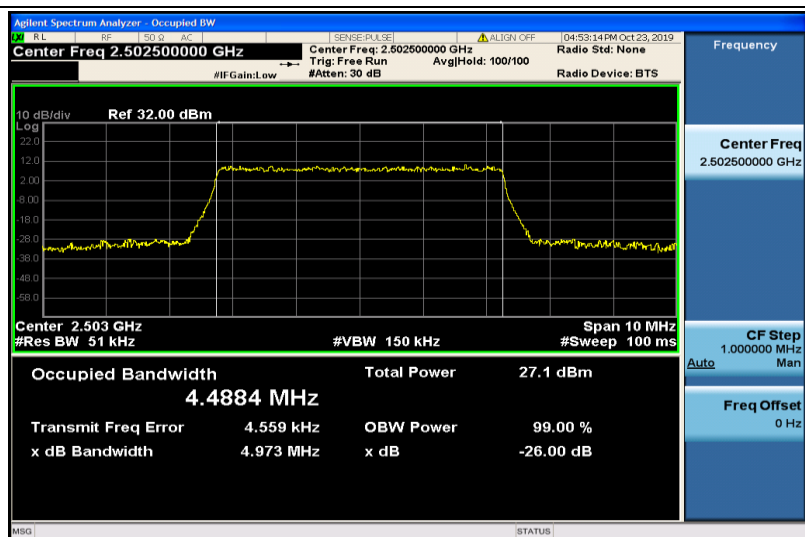
Band7-5MHz-16QAM-20775-25RB#0-4.4884
