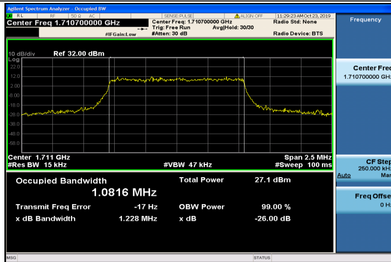
Band4-1.4MHz-16QAM-19957-6RB#0-1.0816
