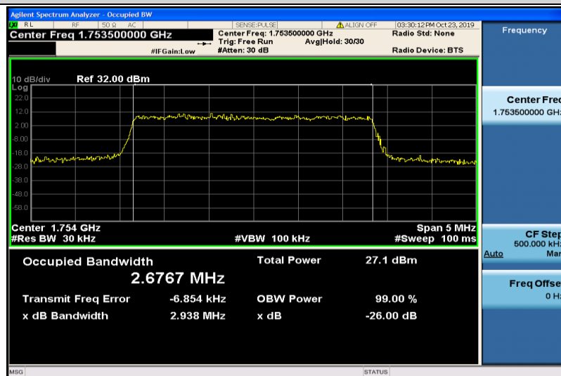
Band4-3MHz-16QAM-20385-15RB#0-2.6767
