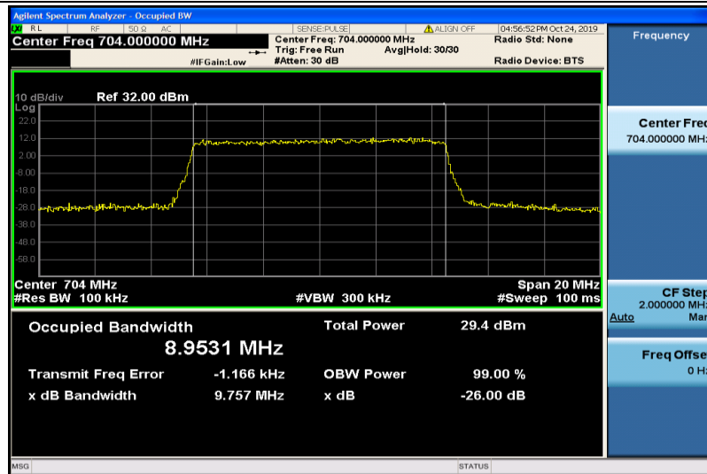
Band12-10MHz-QPSK-23060-50RB#0-8.9531
