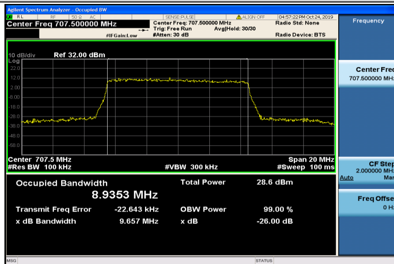
Band12-10MHz-16QAM-23095-50RB#0-8.9353
