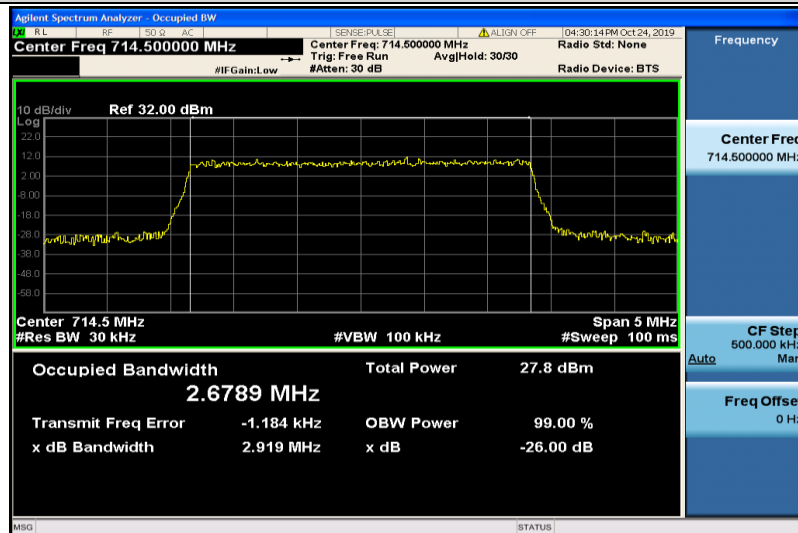
Band12-3MHz-16QAM-23165-15RB#0-2.6789
