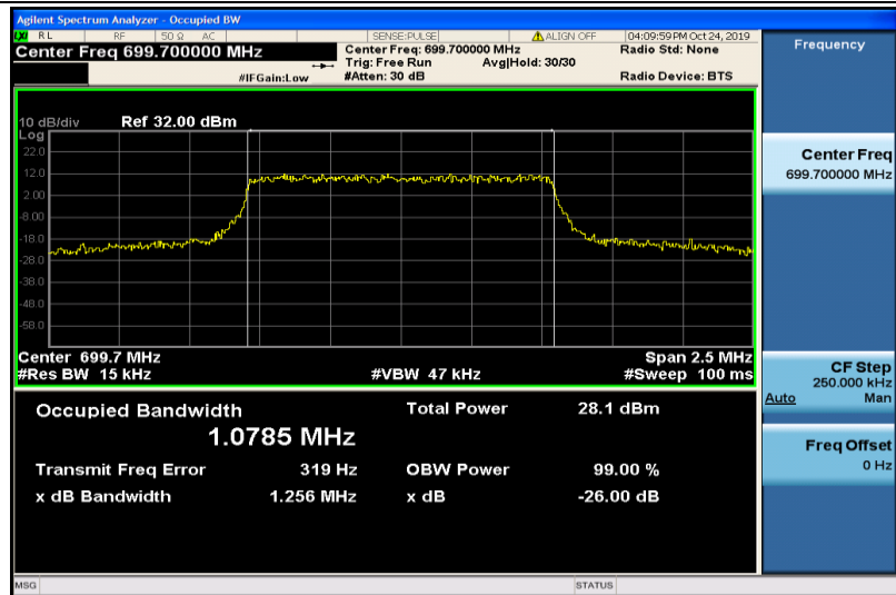
Band12-1.4MHz-QPSK-23017-6RB#0-1.0785
