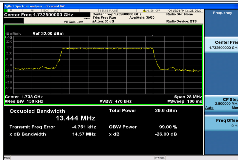
Band4-15MHz-QPSK-20175-75RB#0-13.444
