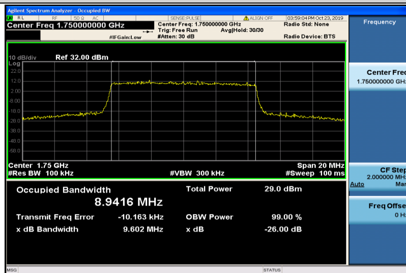
Band4-10MHz-QPSK-20350-50RB#0-8.9416
