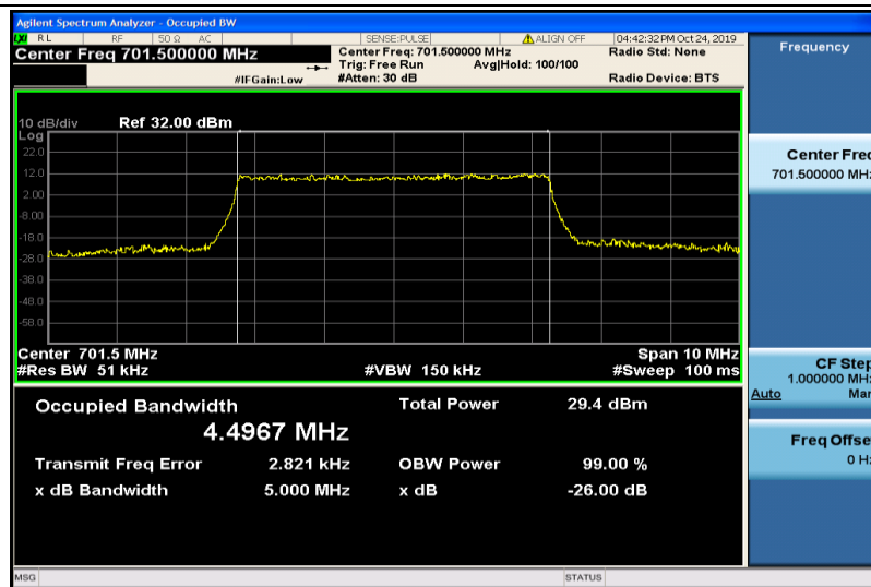
Band12-5MHz-QPSK-23035-25RB#0-4.4967
