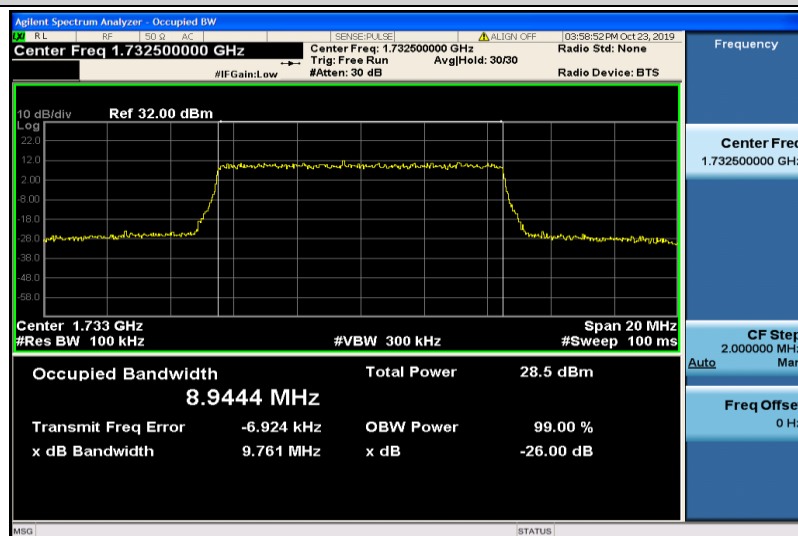
Band4-10MHz-16QAM-20175-50RB#0-8.9444
