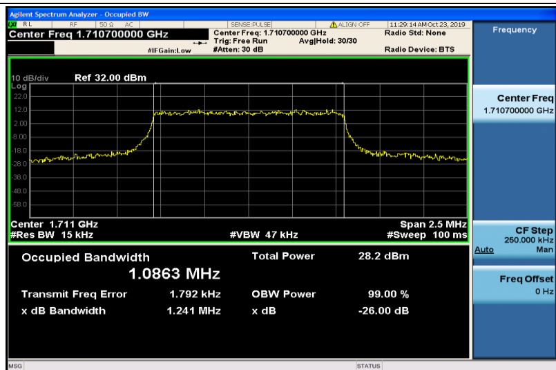
Band4-1.4MHz-QPSK-19957-6RB#0-1.0863
