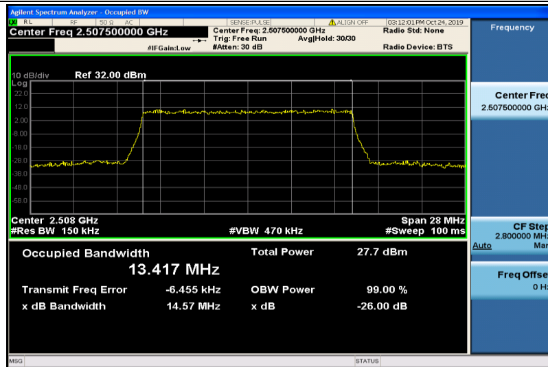
Band7-15MHz-16QAM-20825-75RB#0-13.417
