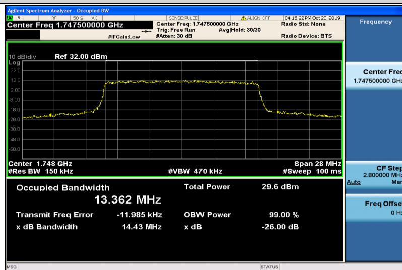
Band4-15MHz-QPSK-20325-75RB#0-13.362
