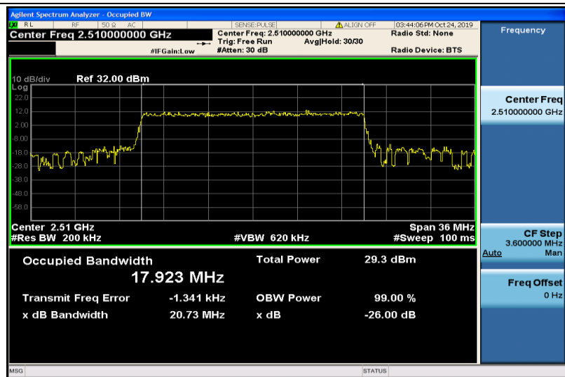
Band7-20MHz-QPSK-20850-100RB#0-17.923
