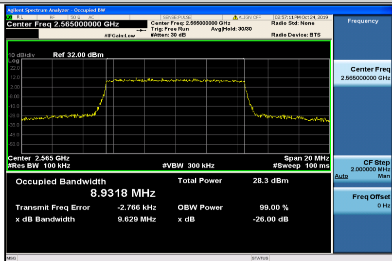
Band7-10MHz-16QAM-21400-50RB#0-8.9318
