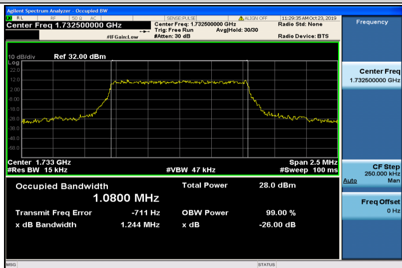
Band4-1.4MHz-QPSK-20175-6RB#0-1.0800
