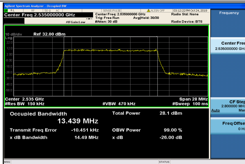
Band7-15MHz-16QAM-21100-75RB#0-13.439
