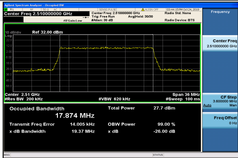
Band7-20MHz-16QAM-20850-100RB#0-17.874
