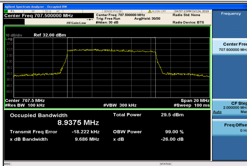
Band12-10MHz-QPSK-23095-50RB#0-8.9375
