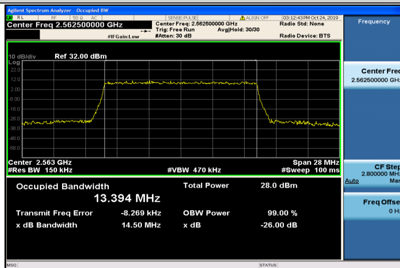
Band7-15MHz-16QAM-21375-75RB#0-13.394
