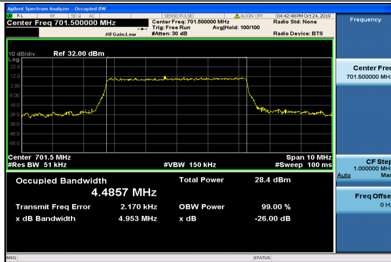
Band12-5MHz-16QAM-23035-25RB#0-4.4857
