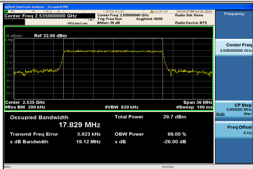
Band7-20MHz-QPSK-21100-100RB#0-17.829
