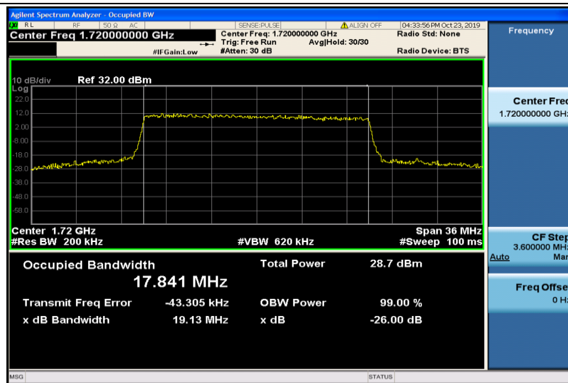
Band4-20MHz-16QAM-20050-100RB#0-17.841
