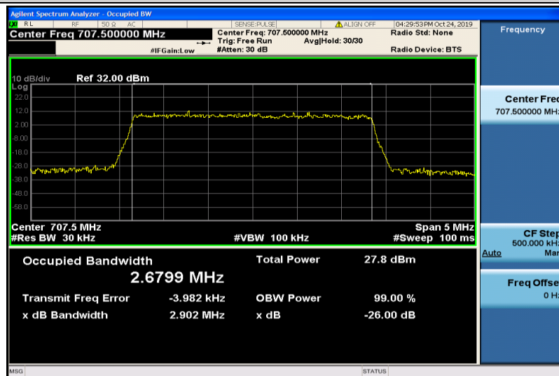
Band12-3MHz-16QAM-23095-15RB#0-2.6799
