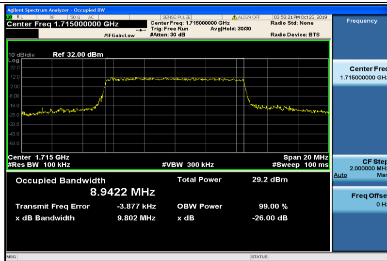
Band4-10MHz-QPSK-20000-50RB#0-8.9422
