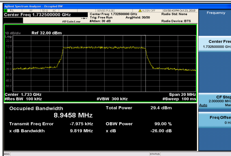
Band4-10MHz-QPSK-20175-50RB#0-8.9458
