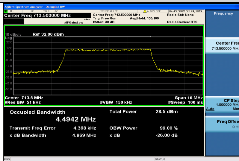
Band12-5MHz-16QAM-23155-25RB#0-4.4942
