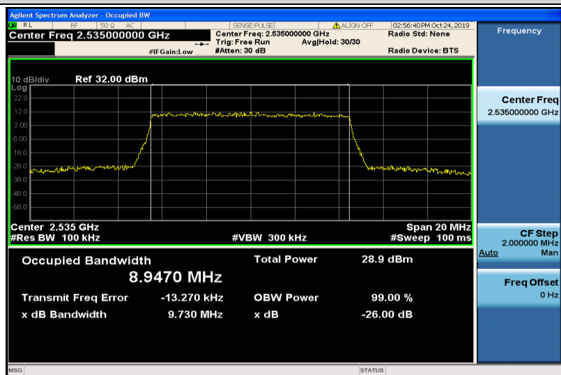
Band7-10MHz-QPSK-21100-50RB#0-8.9470
