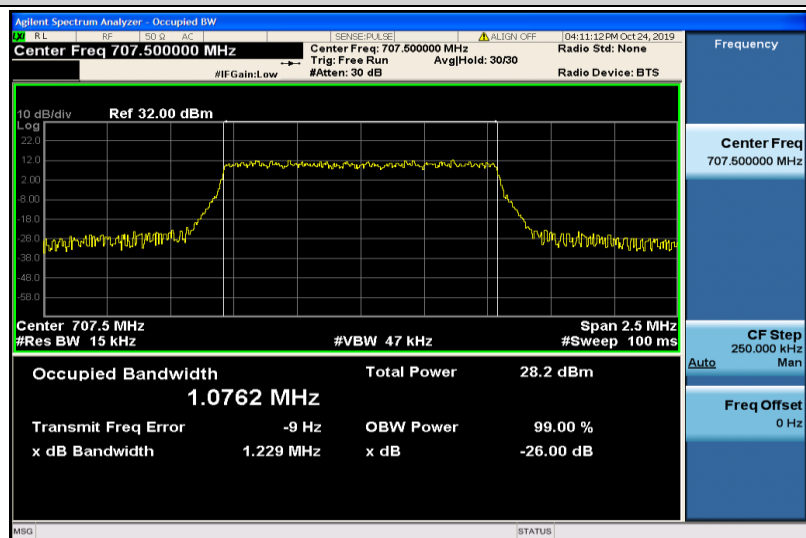
Band12-1.4MHz-QPSK-23095-6RB#0-1.0762
