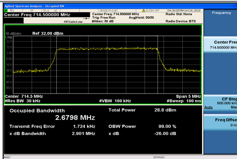
Band12-3MHz-QPSK-23165-15RB#0-2.6798
