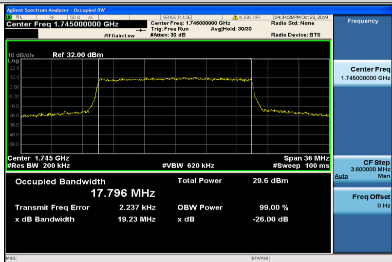
Band4-20MHz-QPSK-20300-100RB#0-17.796
