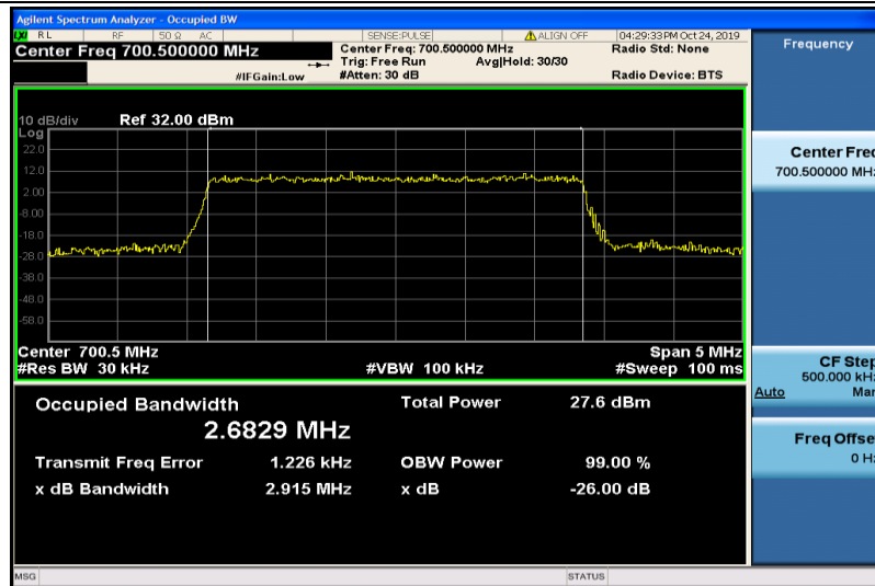
Band12-3MHz-16QAM-23025-15RB#0-2.6829
