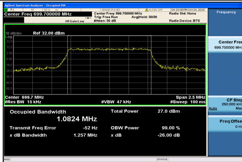
Band12-1.4MHz-16QAM-23017-6RB#0-1.0824
