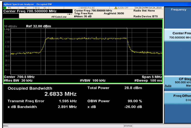
Band12-3MHz-QPSK-23025-15RB#0-2.6833
