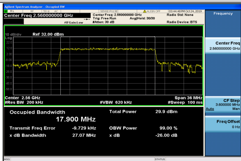
Band7-20MHz-QPSK-21350-100RB#0-17.900
