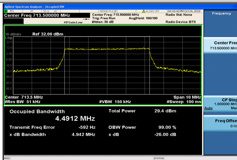
Band12-5MHz-QPSK-23155-25RB#0-4.4912
