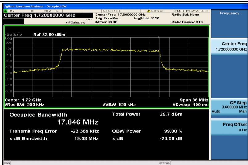
Band4-20MHz-QPSK-20050-100RB#0-17.846
