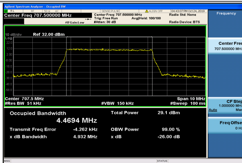
Band12-5MHz-QPSK-23095-25RB#0-4.4694
