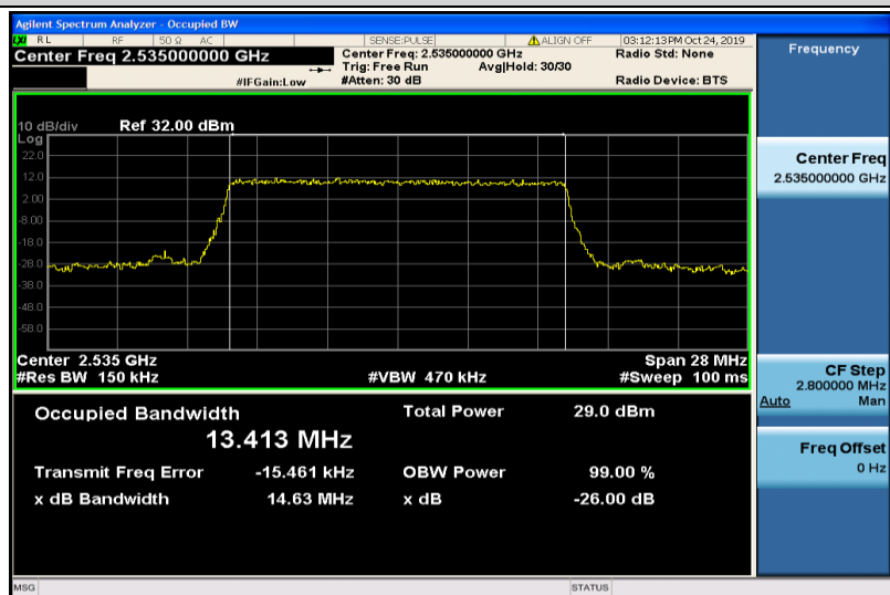
Band7-15MHz-QPSK-21100-75RB#0-13.413
