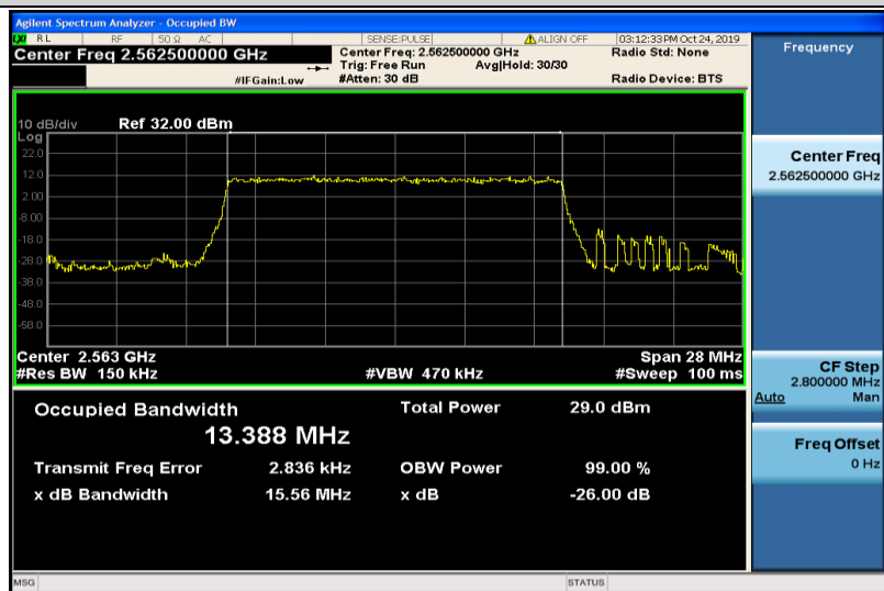
Band7-15MHz-QPSK-21375-75RB#0-13.388
