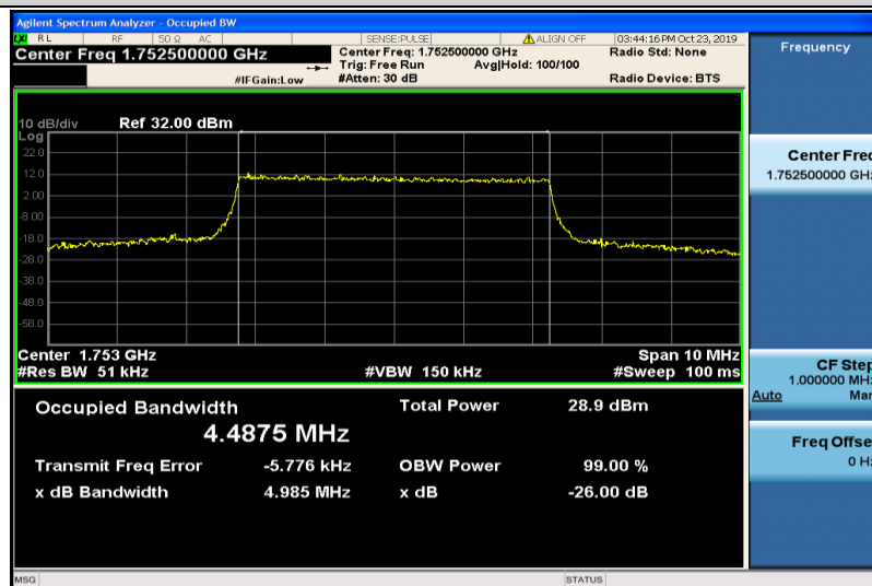
Band4-5MHz-QPSK-20375-25RB#0-4.4875
