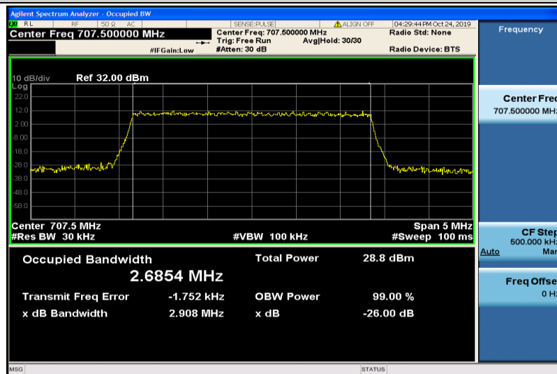
Band12-3MHz-QPSK-23095-15RB#0-2.6854
