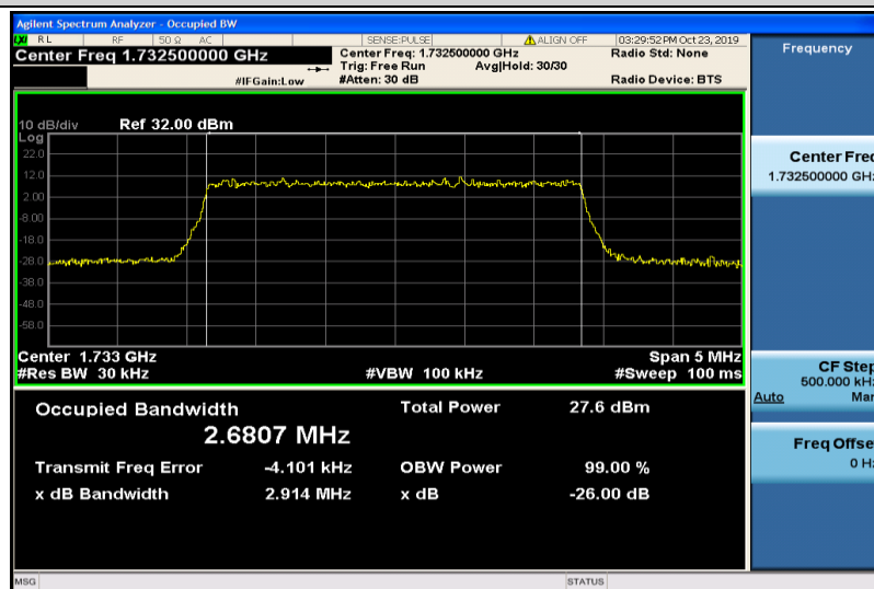
Band4-3MHz-16QAM-20175-15RB#0-2.6807
