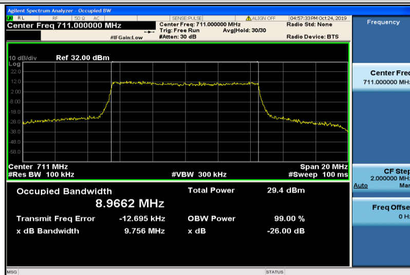
Band12-10MHz-QPSK-23130-50RB#0-8.9662
