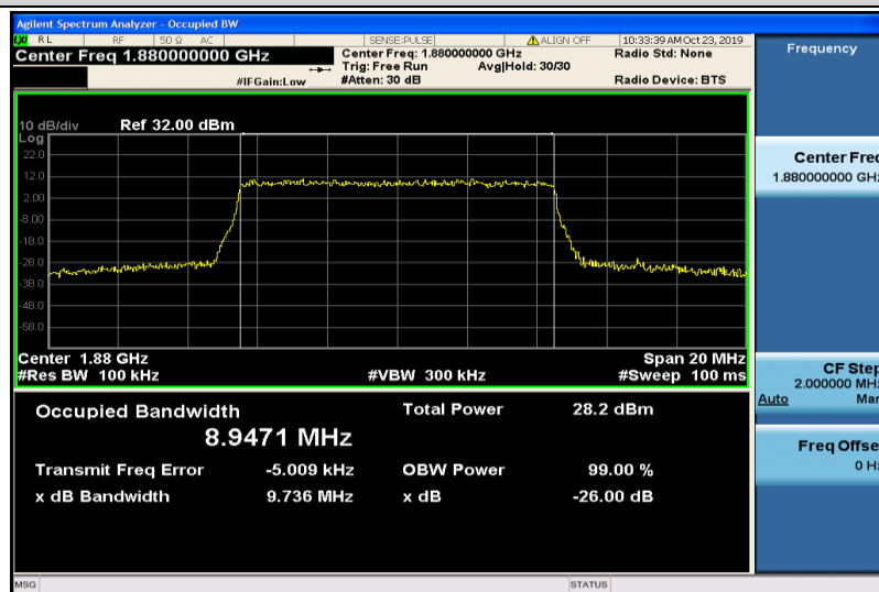
Band2-10MHz-16QAM-18900-50RB#0-8.9471
