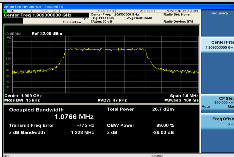
Band2-1.4MHz-QPSK-19193-6RB#0-1.0766
