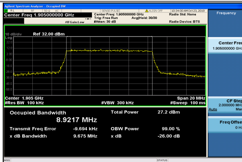
Band2-10MHz-16QAM-19150-50RB#0-8.9217
