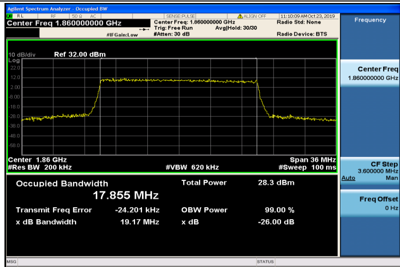
Band2-20MHz-16QAM-18700-100RB#0-17.855
