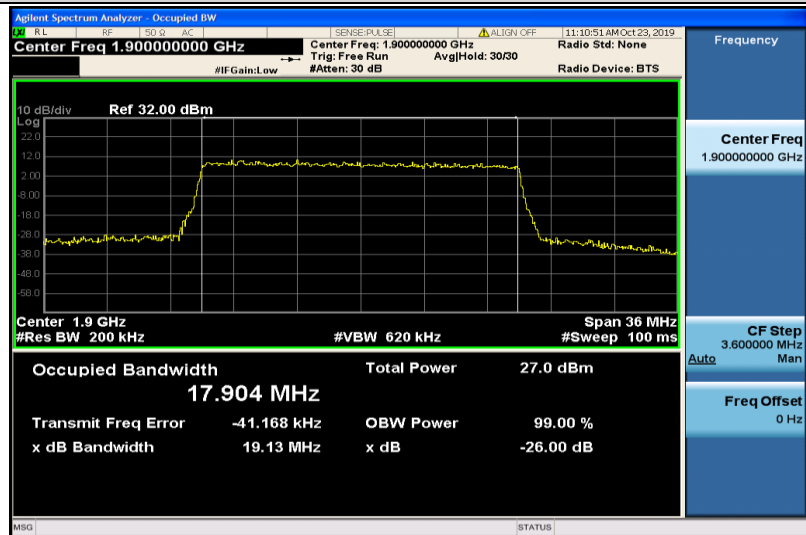
Band2-20MHz-16QAM-19100-100RB#0-17.904
