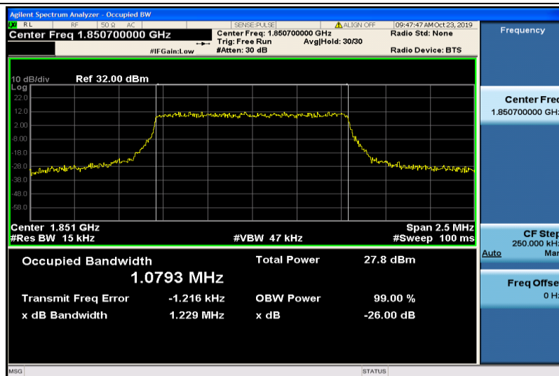
Band2-1.4MHz-QPSK-18607-6RB#0-1.0793
