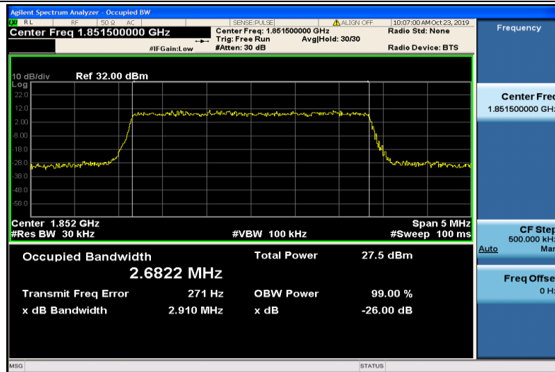
Band2-3MHz-16QAM-18615-15RB#0-2.6822
