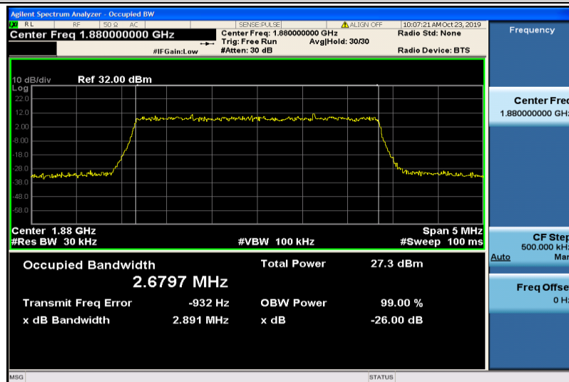
Band2-3MHz-16QAM-18900-15RB#0-2.6797
