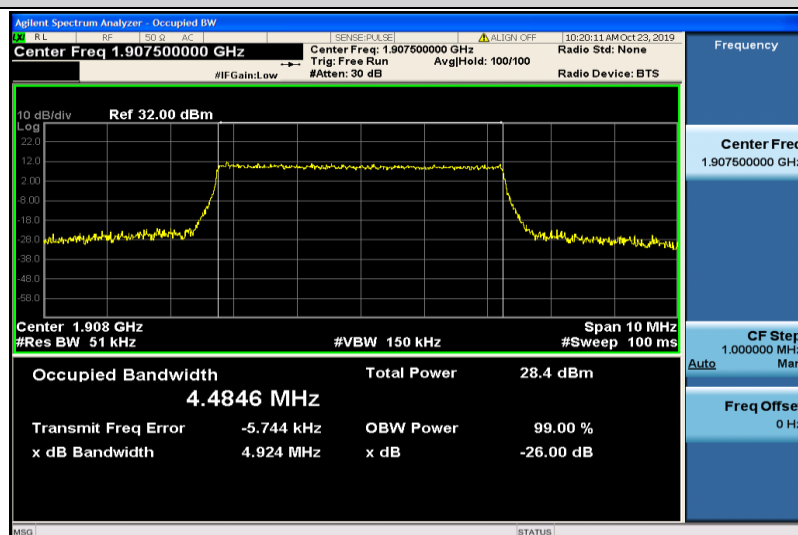
Band2-5MHz-QPSK-19175-25RB#0-4.4846
