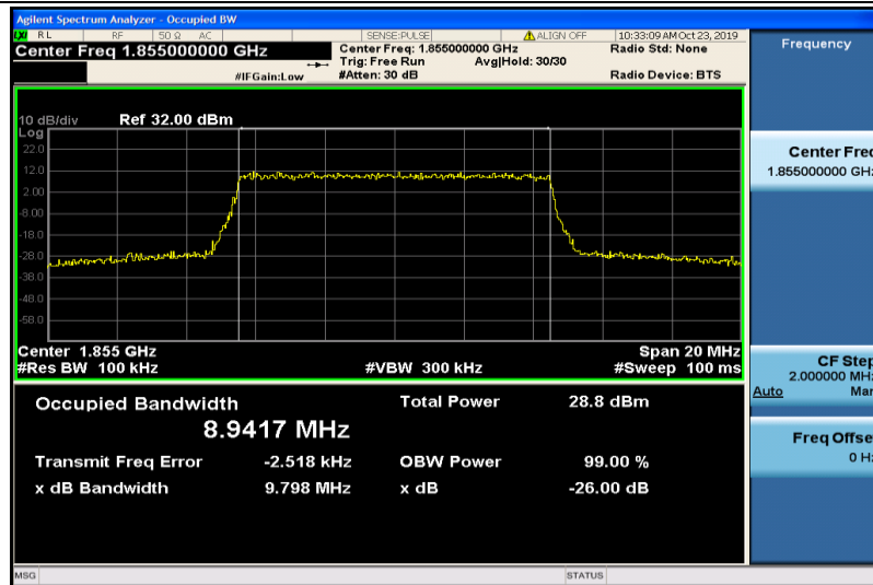
Band2-10MHz-QPSK-18650-50RB#0-8.9417
