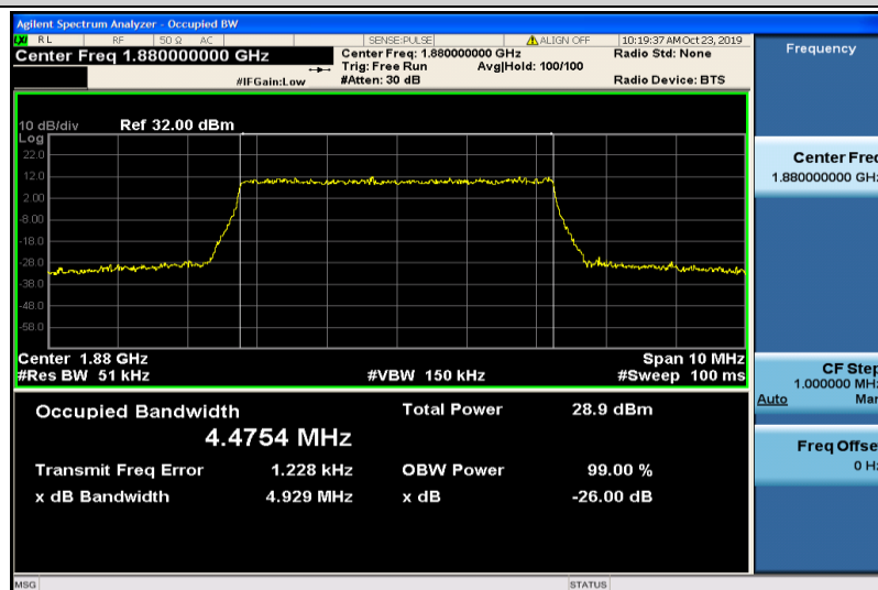
Band2-5MHz-QPSK-18900-25RB#0-4.4754
