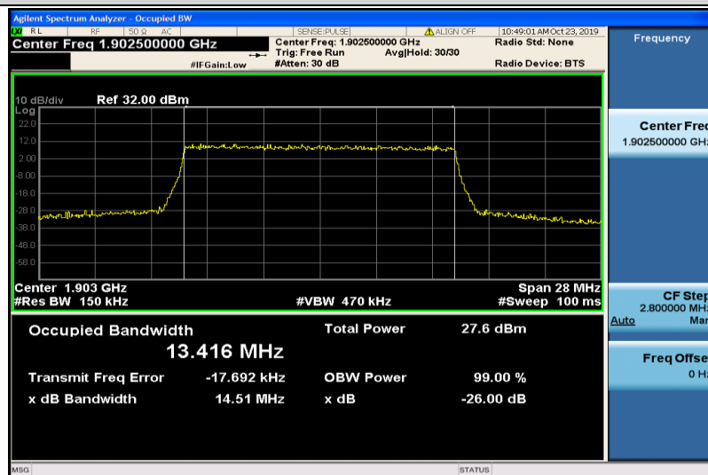
Band2-15MHz-16QAM-19125-75RB#0-13.416
