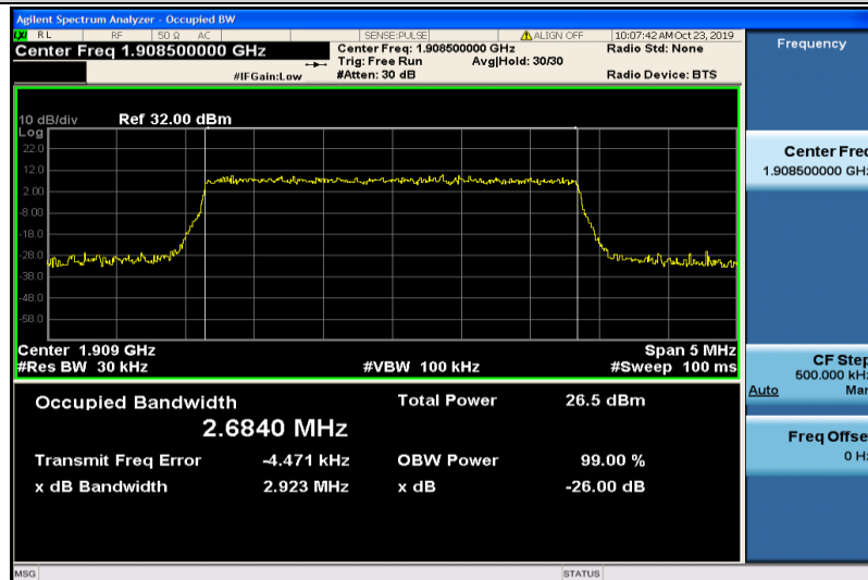
Band2-3MHz-16QAM-19185-15RB#0-2.6840
