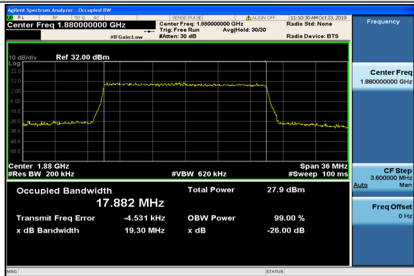
Band2-20MHz-16QAM-18900-100RB#0-17.882
