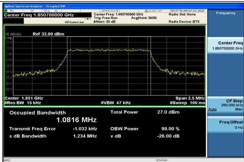
Band2-1.4MHz-16QAM-18607-6RB#0-1.0816
