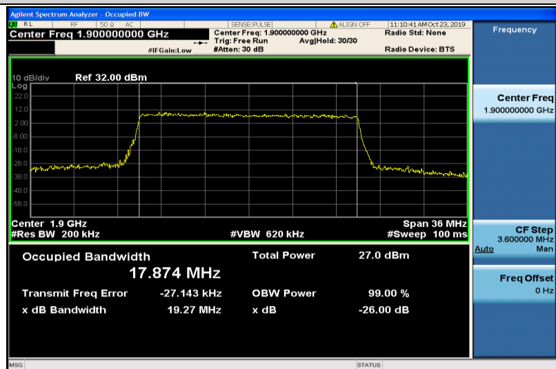
Band2-20MHz-QPSK-19100-100RB#0-17.874
