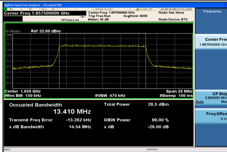
Band2-15MHz-16QAM-18675-75RB#0-13.410
