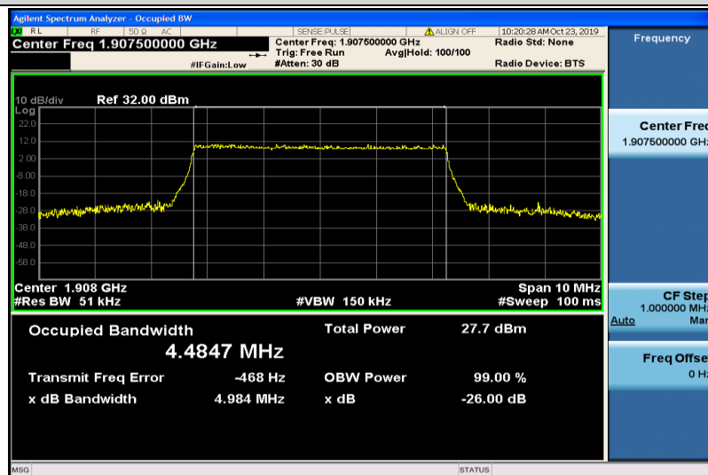
Band2-5MHz-16QAM-19175-25RB#0-4.4847
