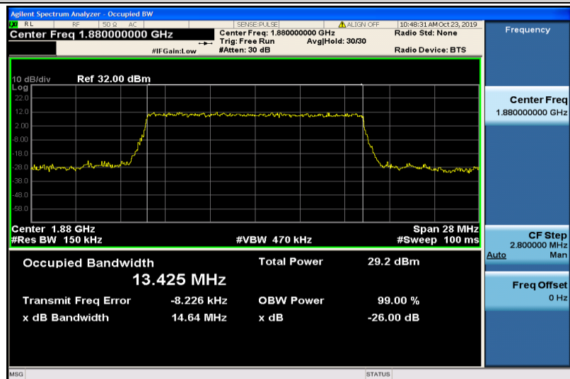
Band2-15MHz-QPSK-18900-75RB#0-13.425
