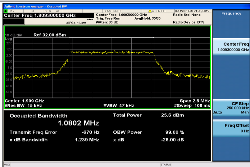
Band2-1.4MHz-16QAM-19193-6RB#0-1.0802
