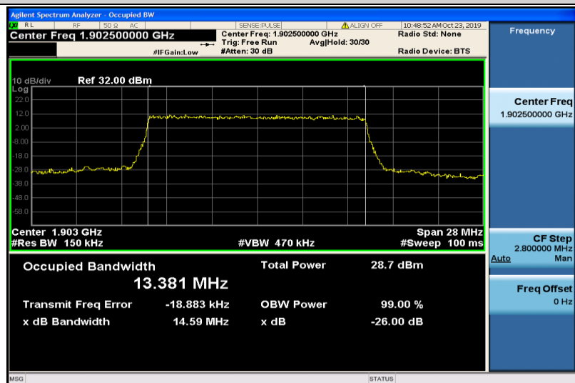
Band2-15MHz-QPSK-19125-75RB#0-13.381
