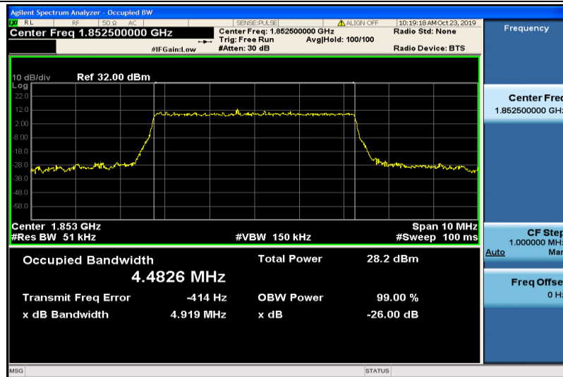
Band2-5MHz-16QAM-18625-25RB#0-4.4826
