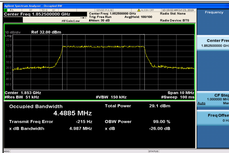
Band2-5MHz-QPSK-18625-25RB#0-4.4885
