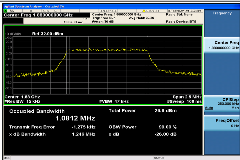
Band2-1.4MHz-16QAM-18900-6RB#0-1.0812
