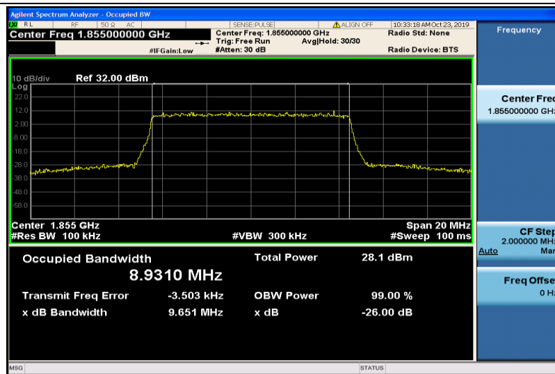
Band2-10MHz-16QAM-18650-50RB#0-8.9310
