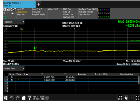
N2(15M)_DFT-s- OFDM_QPSK_Edge_1RB_Left_High_CH
