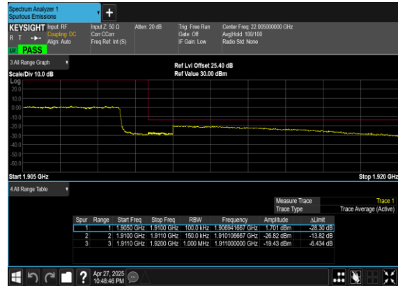
N2(15M)_DFT-s- OFDM_QPSK_Outer_Full_High_CH
