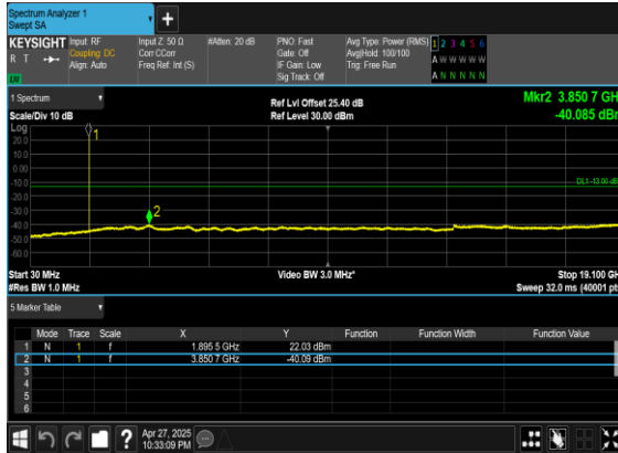
N2(15M)_DFT-s- OFDM_BPSK_Edge_1RB_Left_High_CH
