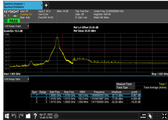
N2(15M)_DFT-s- OFDM_QPSK_Edge_1RB_Right_High_CH
