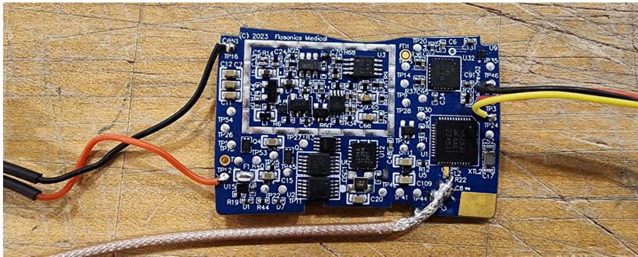
Figure 2 – Front (Shield Removed)
