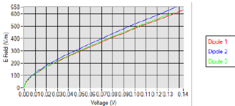
Calibration curves
