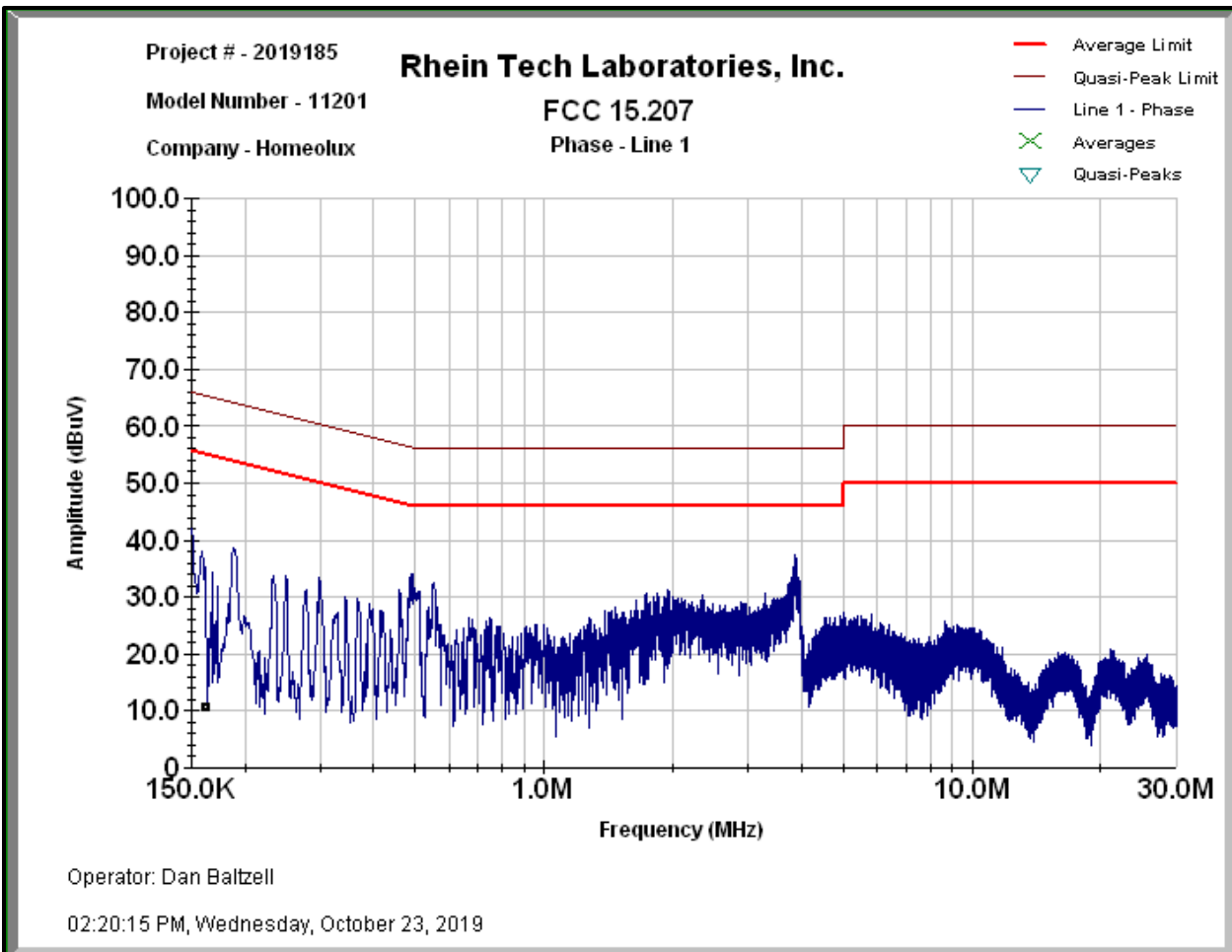
Plot 4-1: Conducted AC Emissions – Phase
