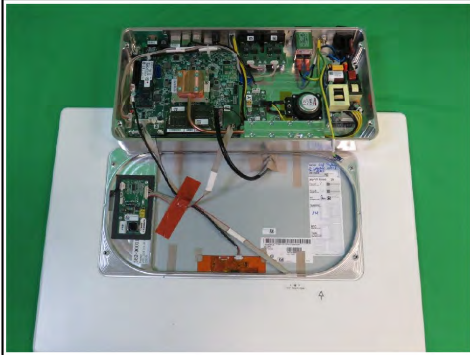
OR-PC® 24 Intern Architecture View 1
