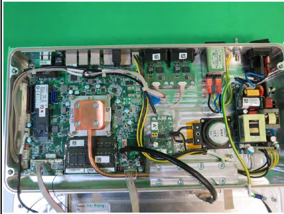
OR-PC® 21 Intern Architecture View 7
