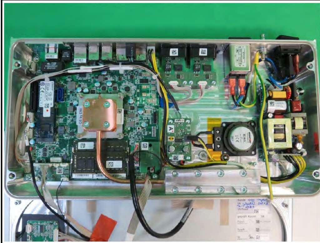
OR-PC® 24 Intern Architecture View 7
