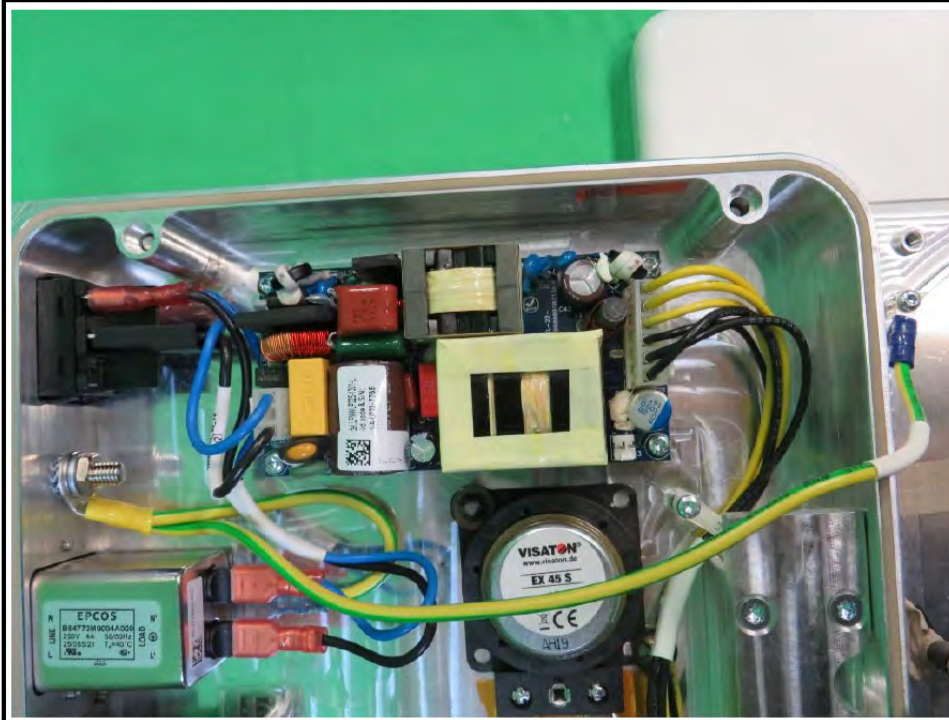
OR-PC® 21 Intern Architecture View 10
