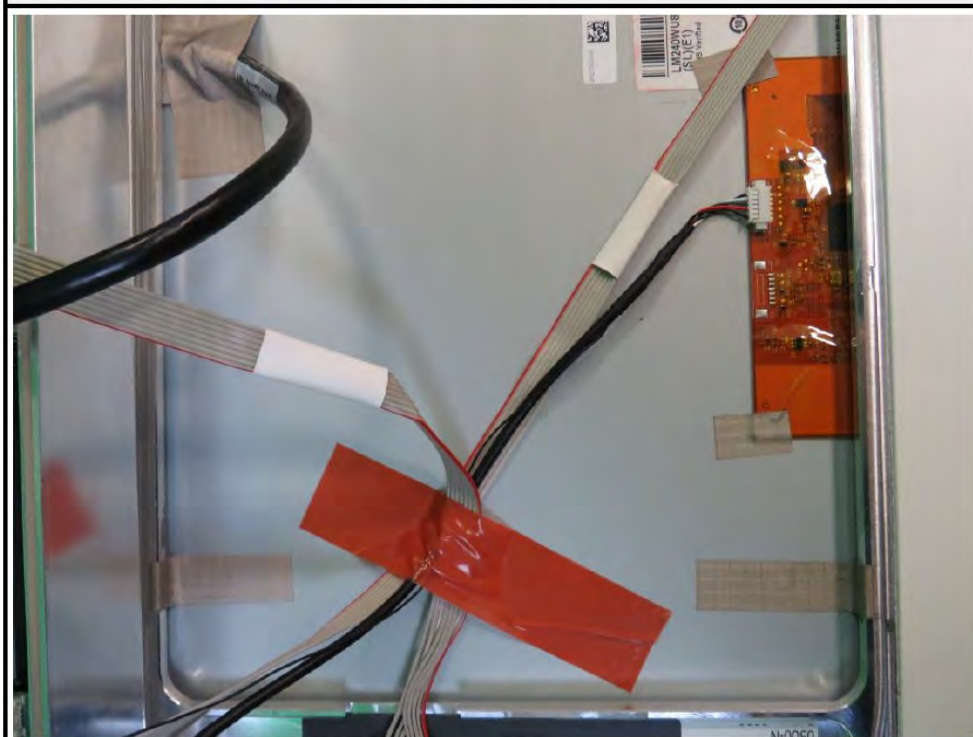
OR-PC® 24 Intern Architecture View 4
