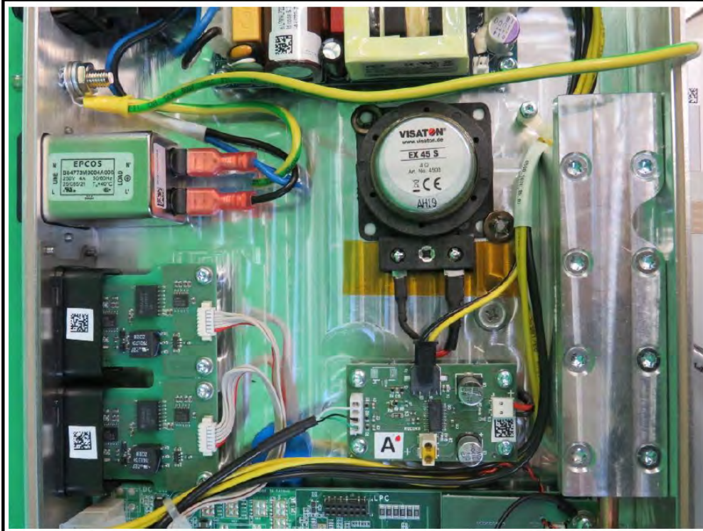
OR-PC® 24 Intern Architecture View 9
