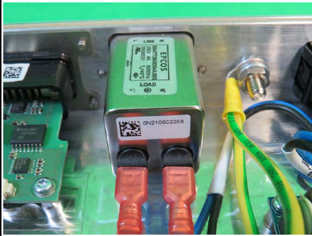
OR-PC® 24 Intern Architecture View 11
