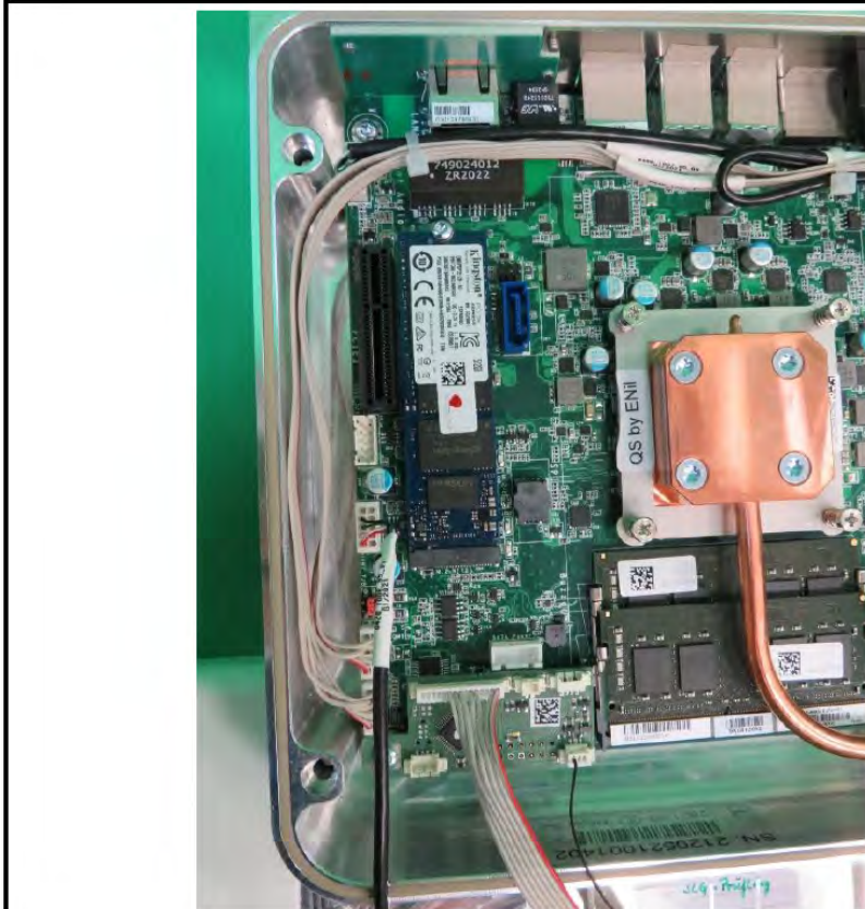
OR-PC® 21 Intern Architecture View 8
