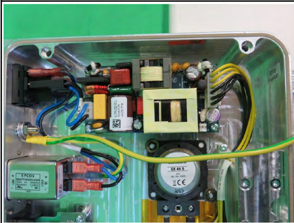
OR-PC® 24 Intern Architecture View 10
