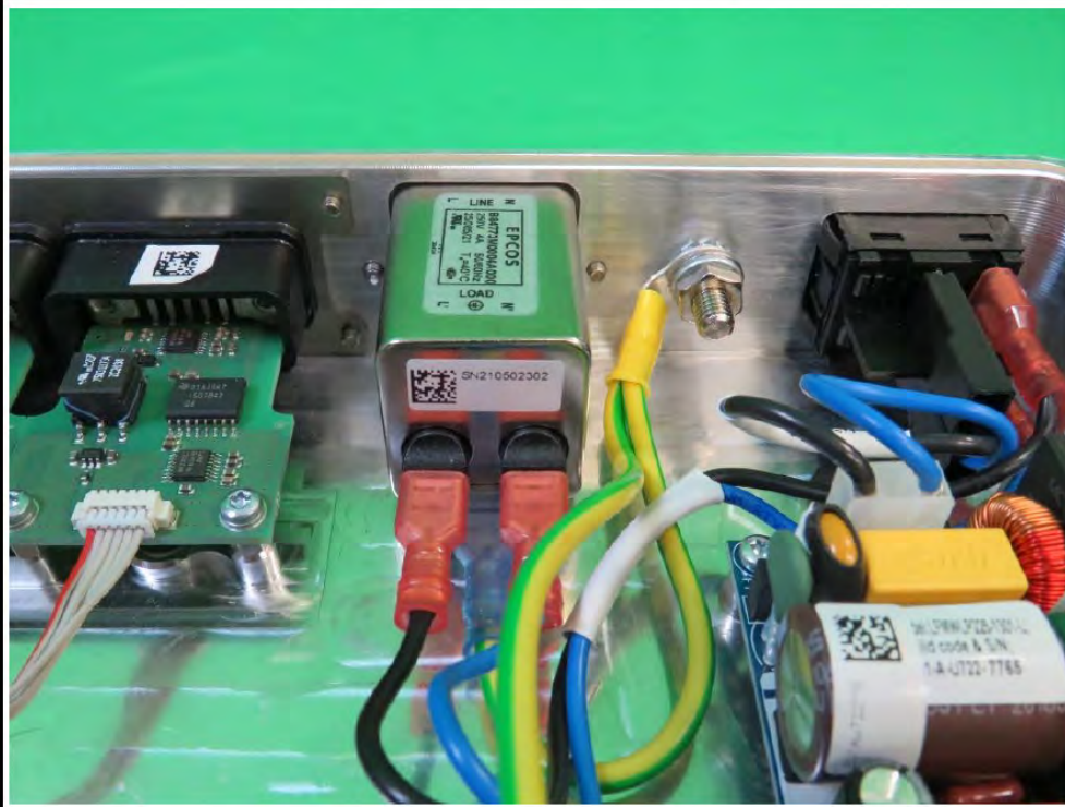
OR-PC® 21 Intern Architecture View 11
