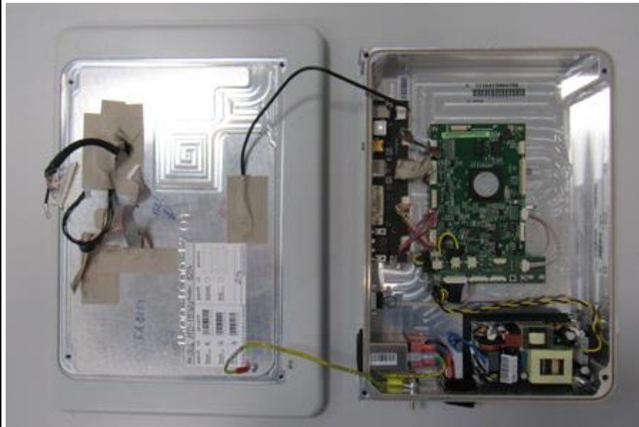
EUT TOP AND BOTTOM SIDE
