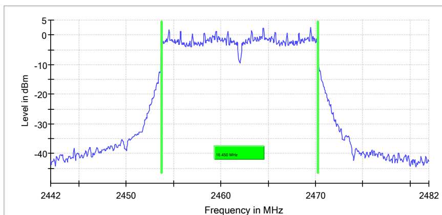
6 dB Bandwidth
