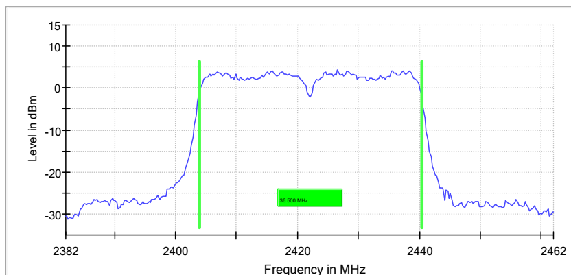
99 % Bandwidth
