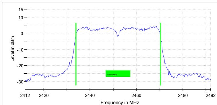
99 % Bandwidth
