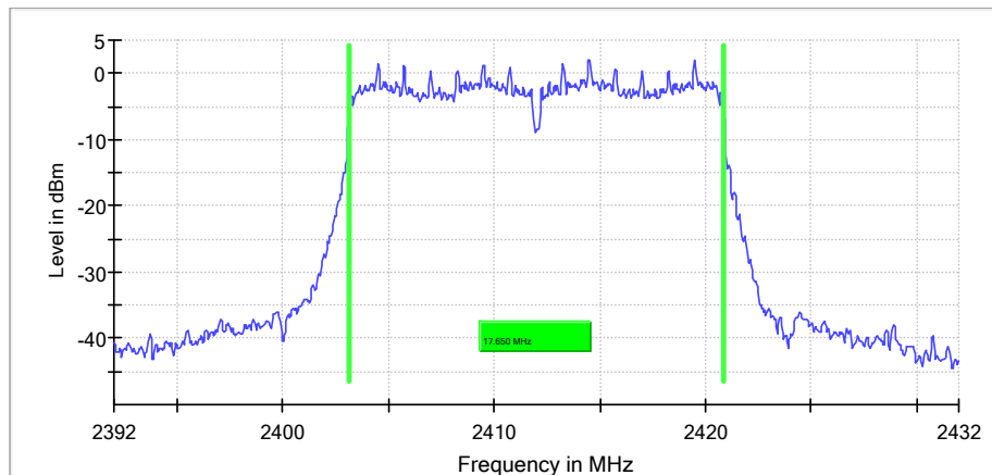
6 dB Bandwidth
