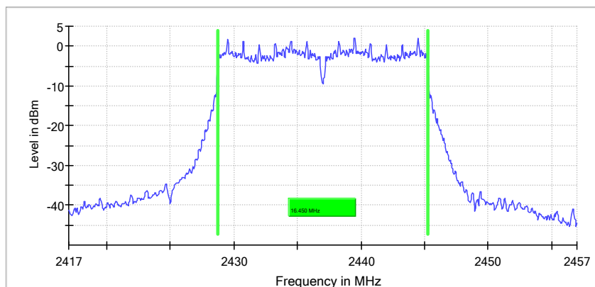
6 dB Bandwidth
