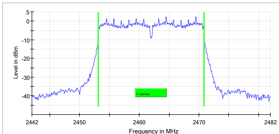
6 dB Bandwidth
