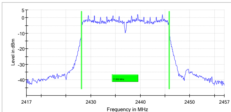
6 dB Bandwidth
