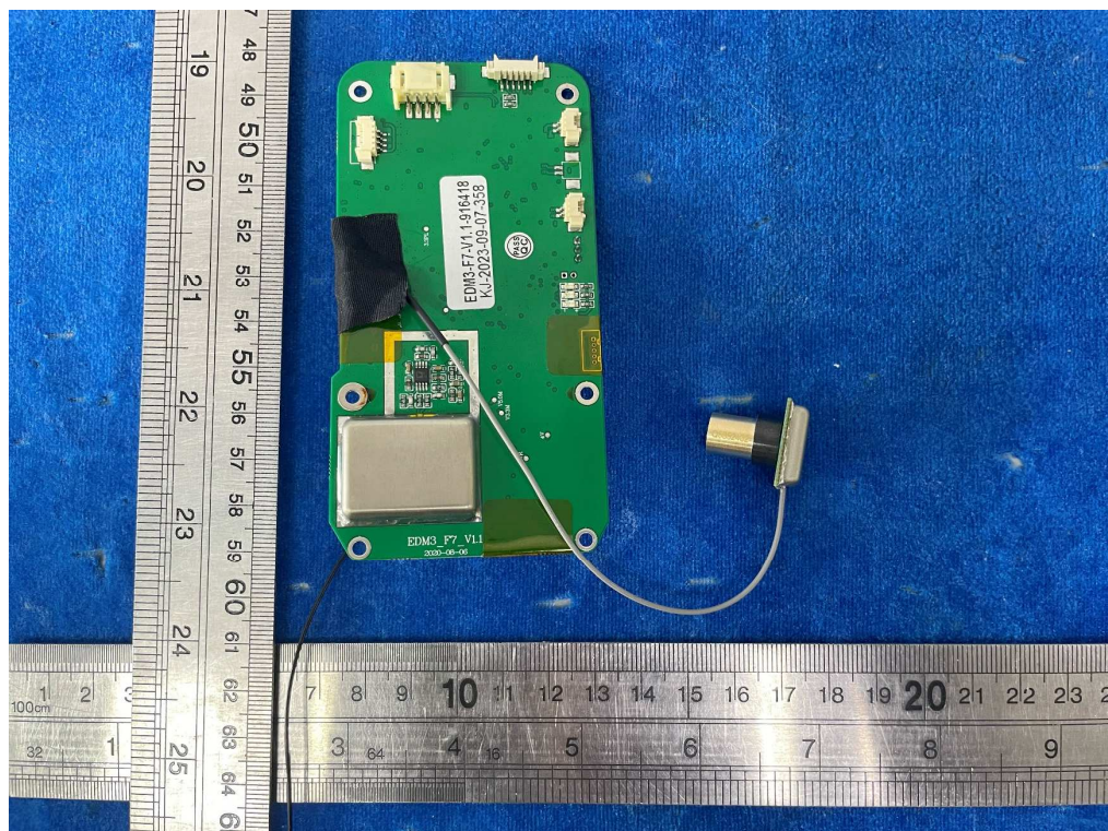
Picture 36: View of the EDM PCBA module
