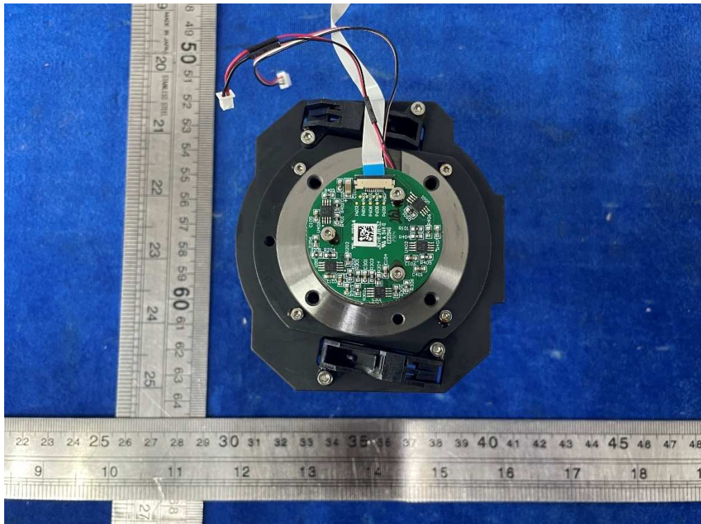
Picture 46: View of the Hz array board
