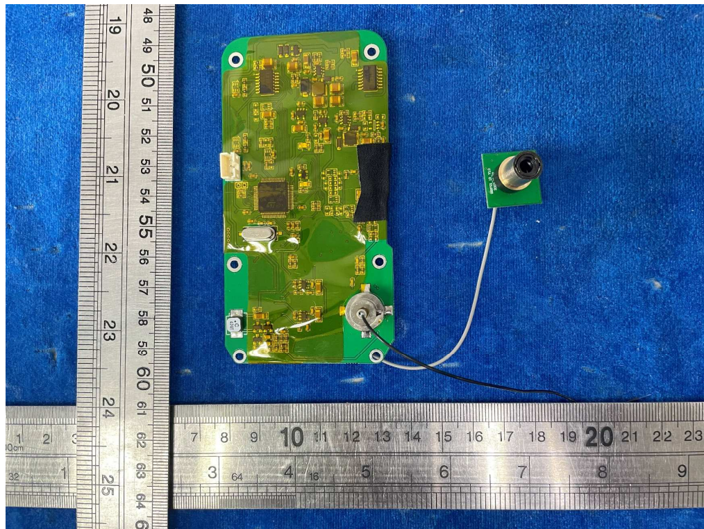
Picture 35: View of the EDM PCBA module
