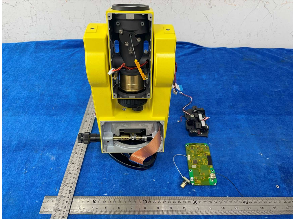
Picture 34: Internal view
