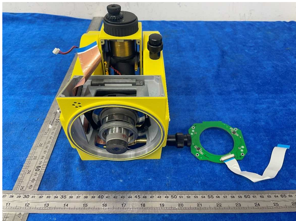
Picture 44: Internal view
