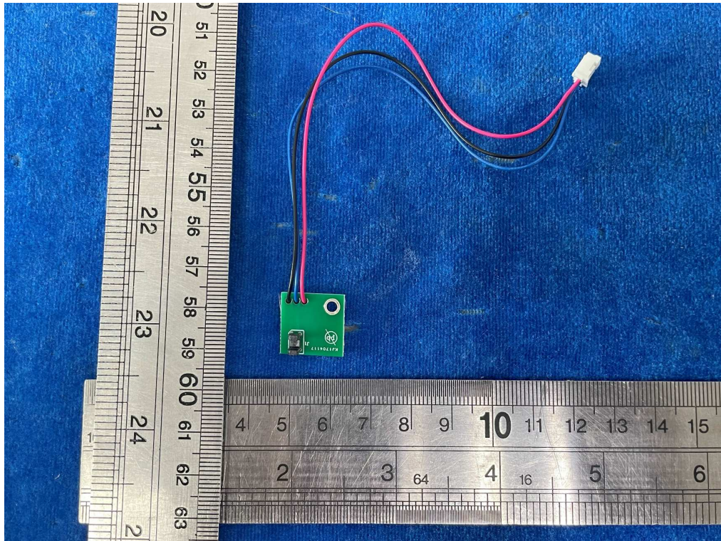
Picture 39: View of the initial position PCB
