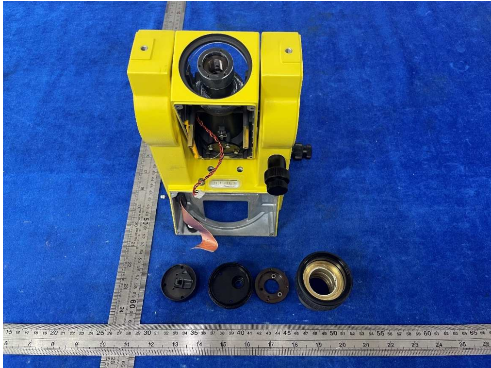
Picture 41: Internal view of focusing telescope and eyepiece
