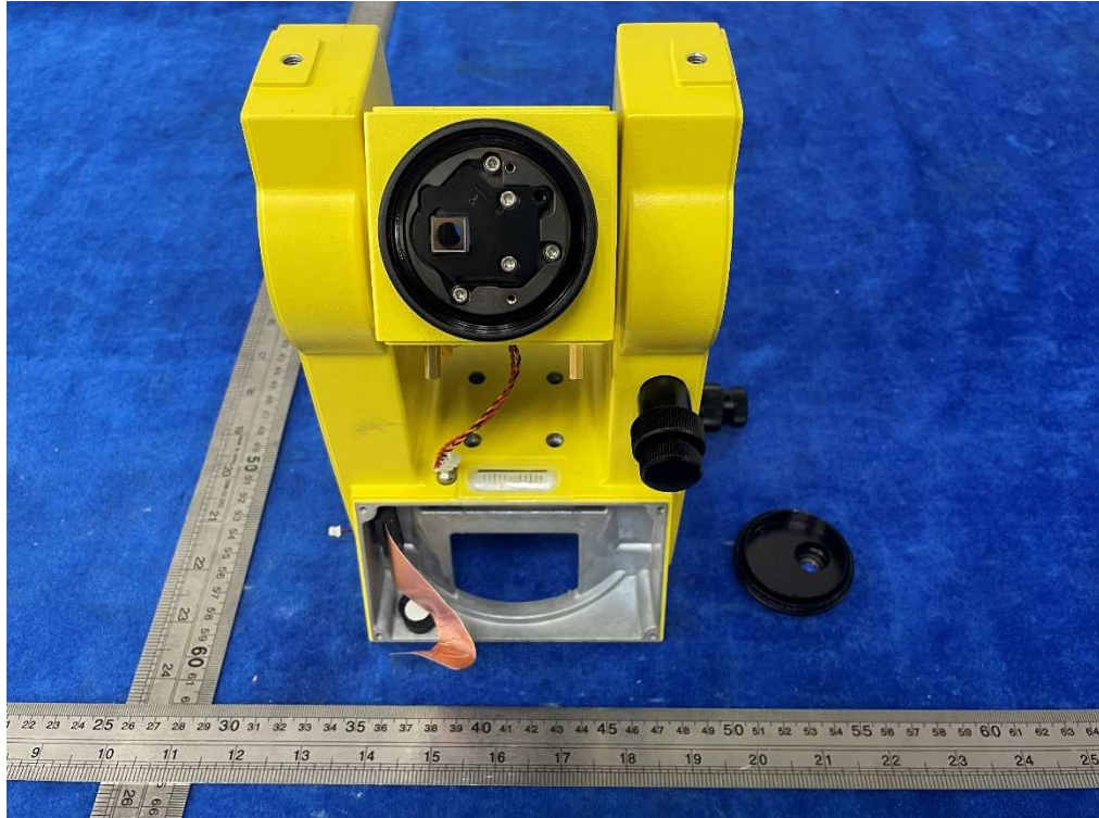
Picture 40: Internal view of focusing telescope and eyepiece
