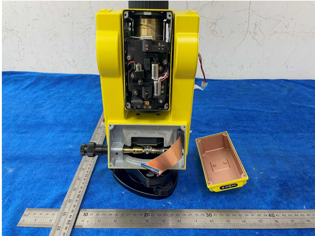
Picture 33: Internal view
