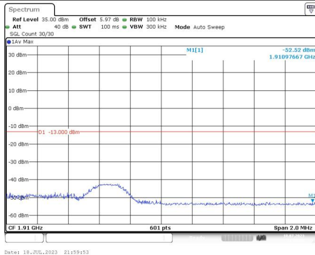
Band2-5MHz-16QAM-19175-1RB#24
