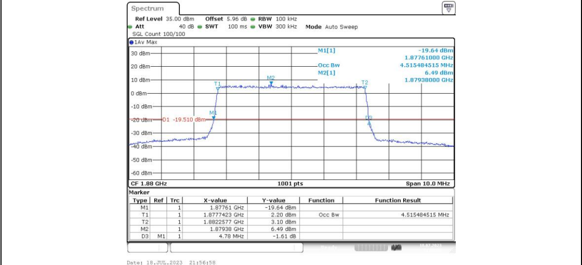
Band2-5MHz-16QAM-19175-25RB#0
