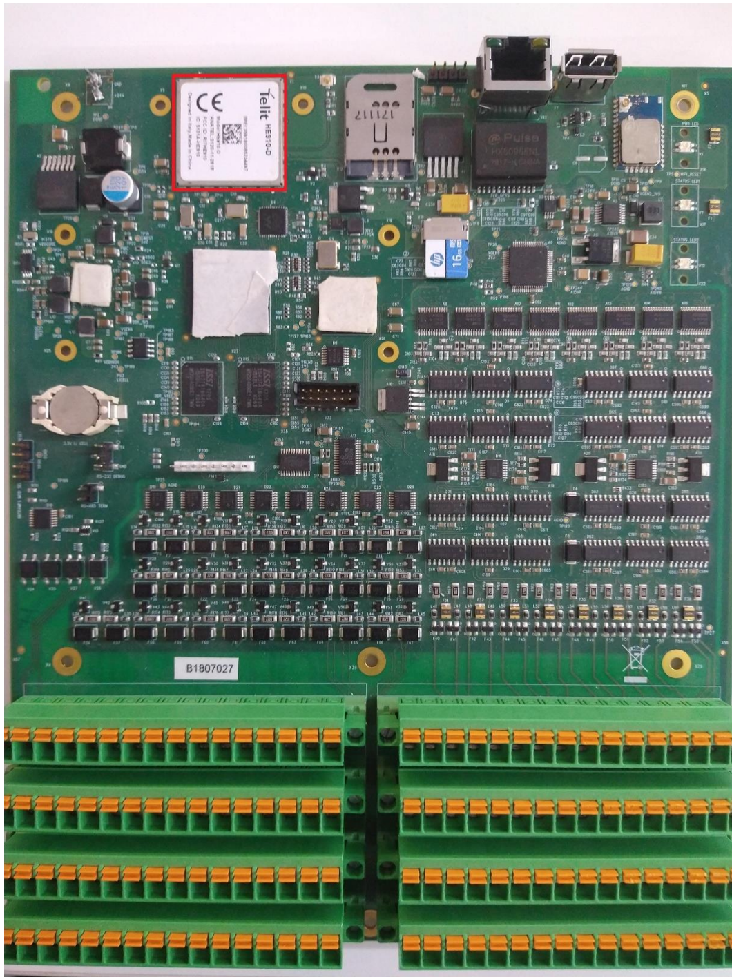
Photo 7: PCB front view showing Telit RF module
