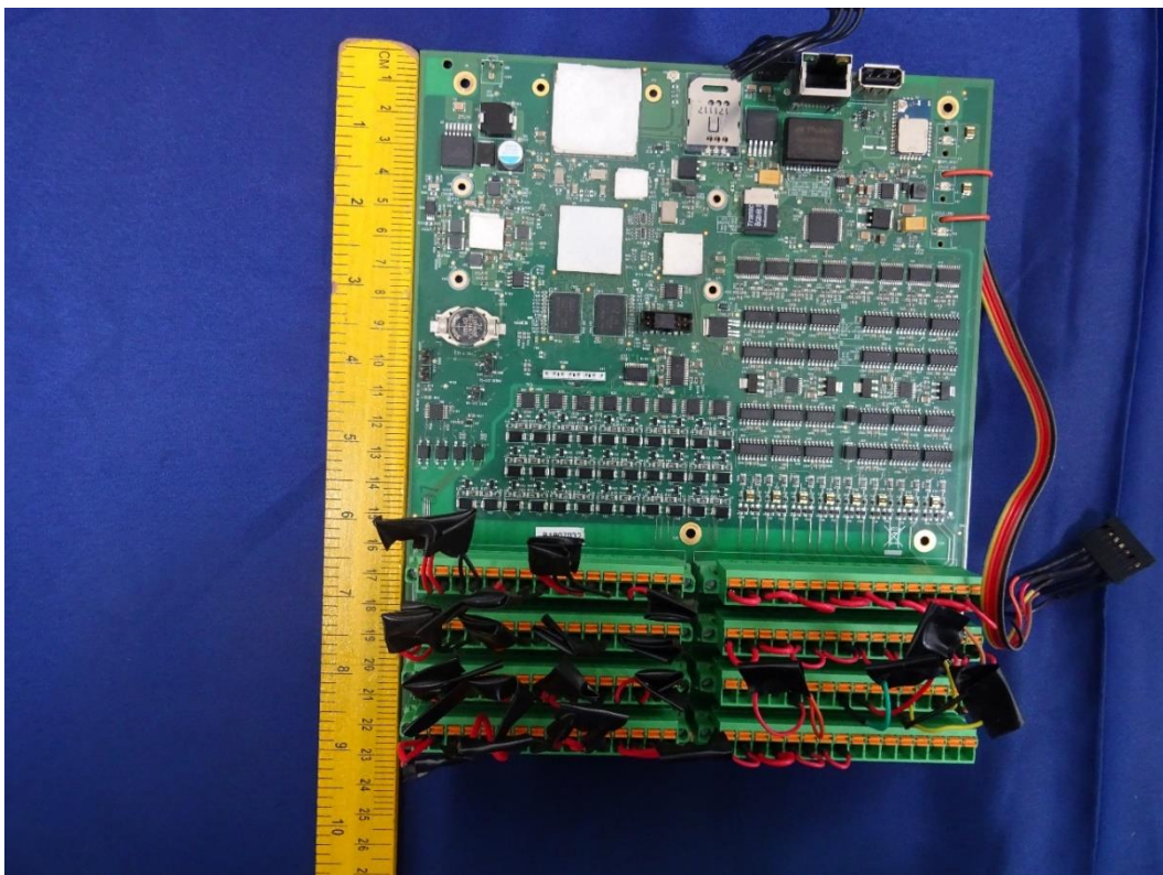
Photo 4: Dimensional view of internal PCB (Length)
