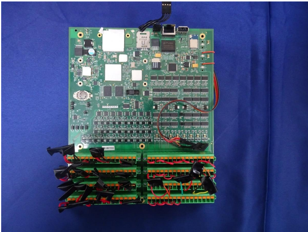
Photo 2: PCB front view
