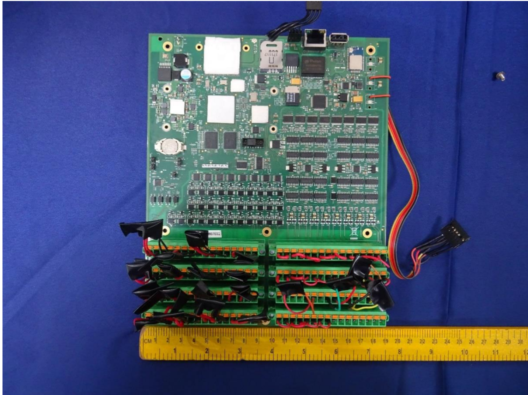
Photo 5: Dimensional view of internal PCB (width)
