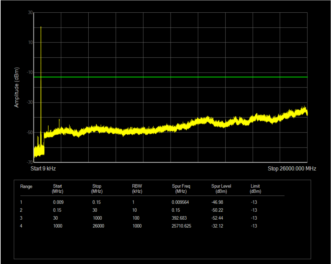
Band12 QAM16 BW=10MHz Channel=23060 RB Size=1 Position=#0 NB Index=0
