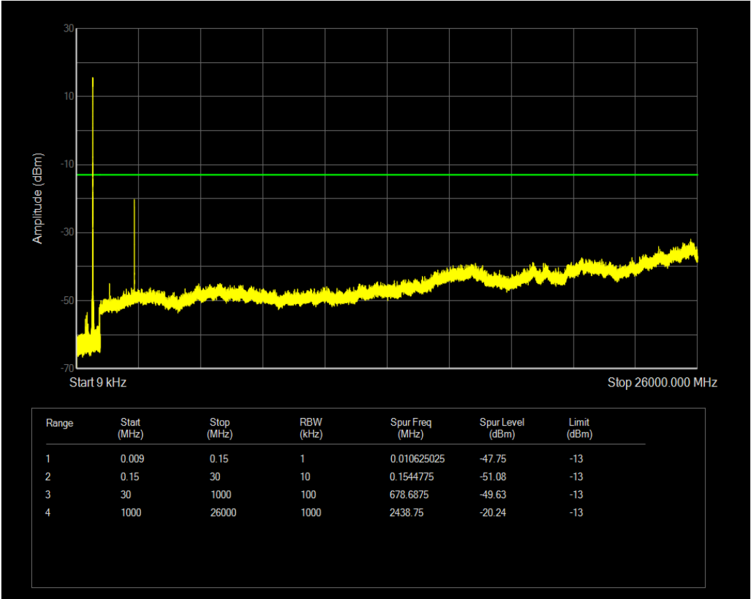
Band12 QAM16 BW=5MHz Channel=23035 RB Size=1 Position=#0 NB Index=0
