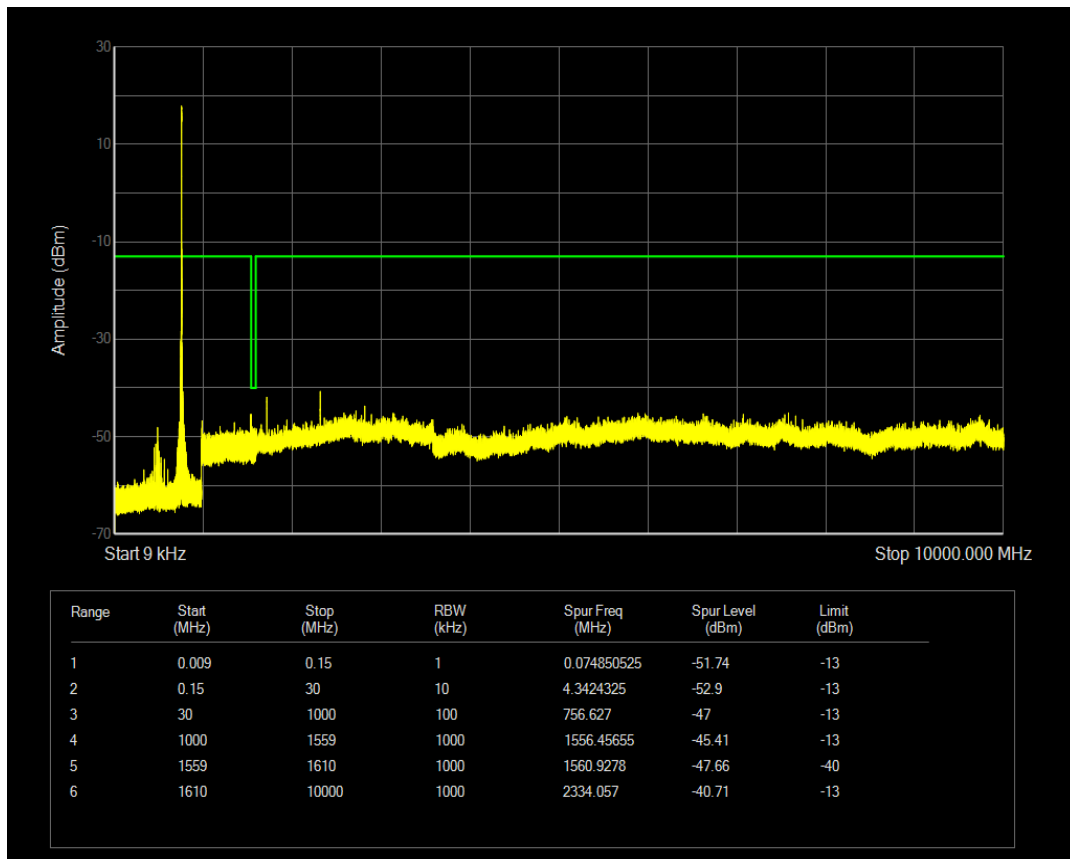
Band13 QPSK BW=5MHz Channel=23255 RB Size=1 Position=#0 NB Index=0
