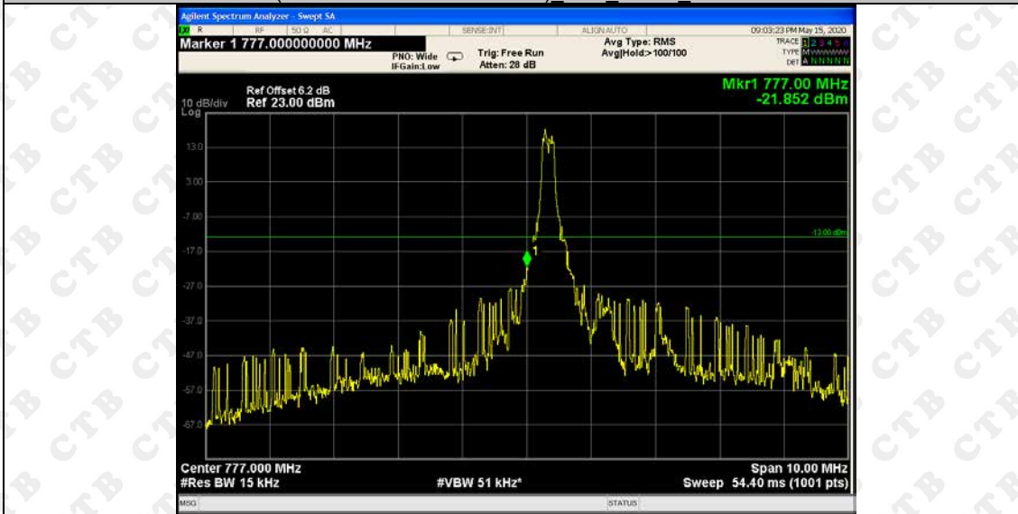
(Channel Bandwidth: 5 MHz) LCH QPSK_6RB#0
