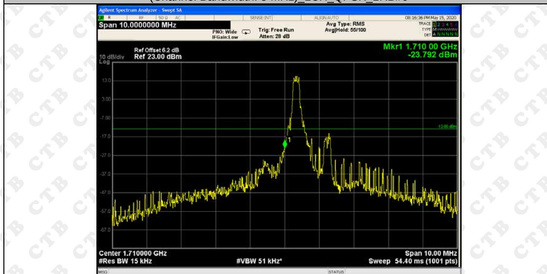
(Channel Bandwidth: 5 MHz)_LCH_QPSK_1RB#0
