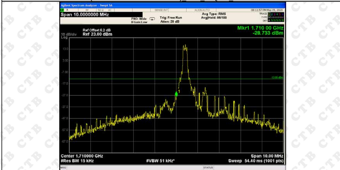
(Channel Bandwidth: 3 MHz) LCH 16QAM 5RB#0
