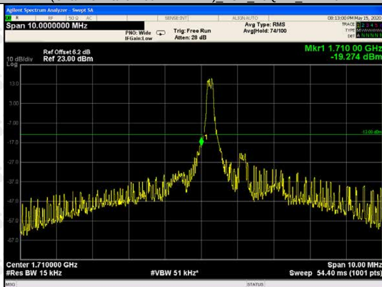
(Channel Bandwidth: 1.4 MHz) _LCH_16QAM_1RB#0
