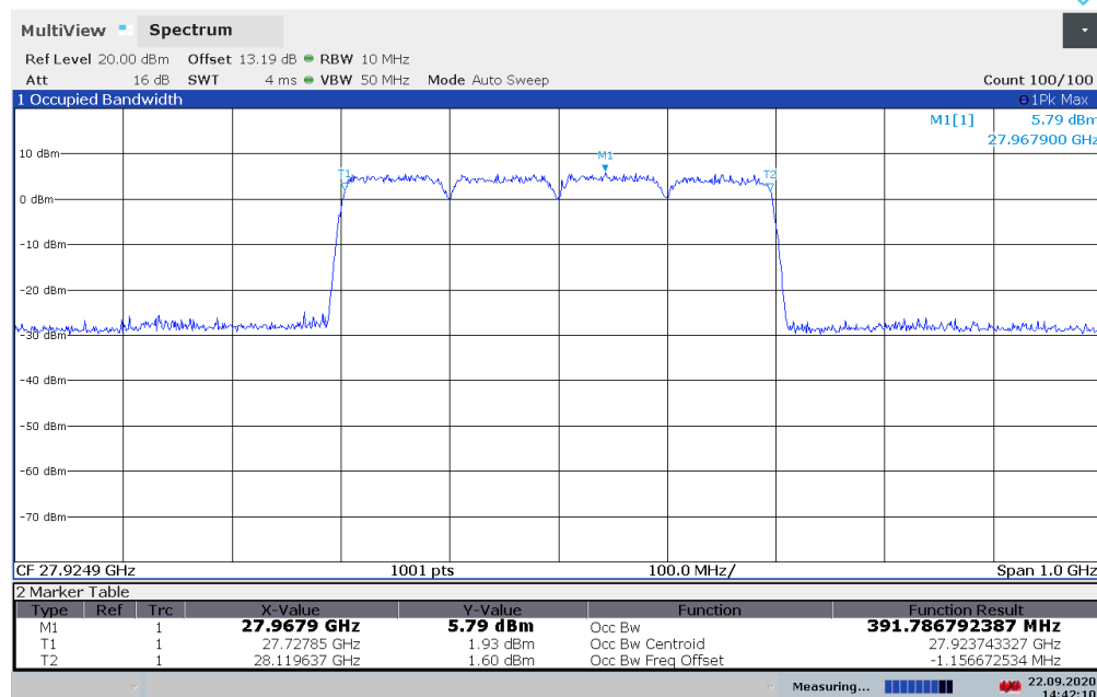
Plot 7-8. Occupied Bandwidth Plot - HBF Antenna (400MHz 4CC- 16QAM - Mid Channel) – V
