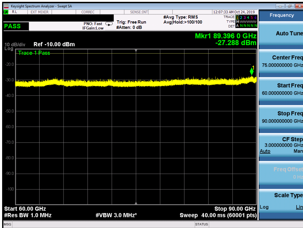
Plot 7-44. HBF Antenna Radiated Spurious Plot 60-90 GHz (1CC QPSK Mid Channel H Beam)
