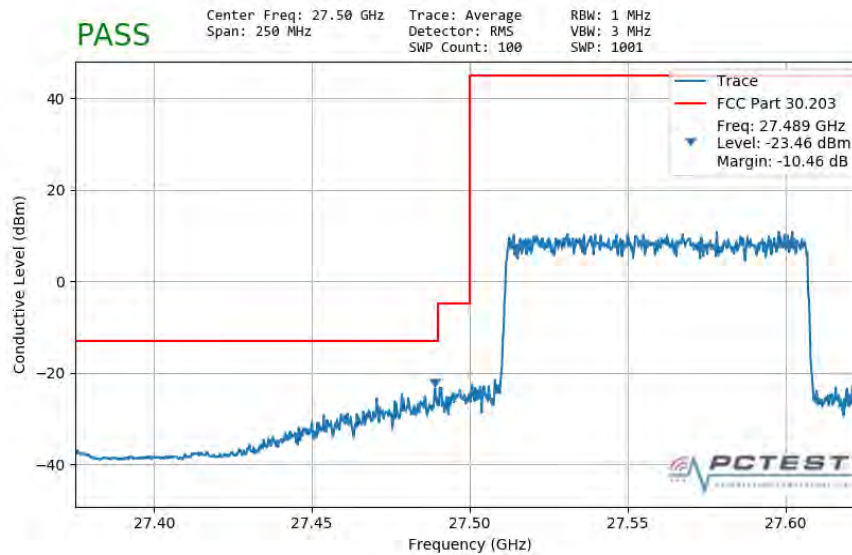
Plot 7-93. Lower Band Edge Plot (100MHz QPSK Full RB)
