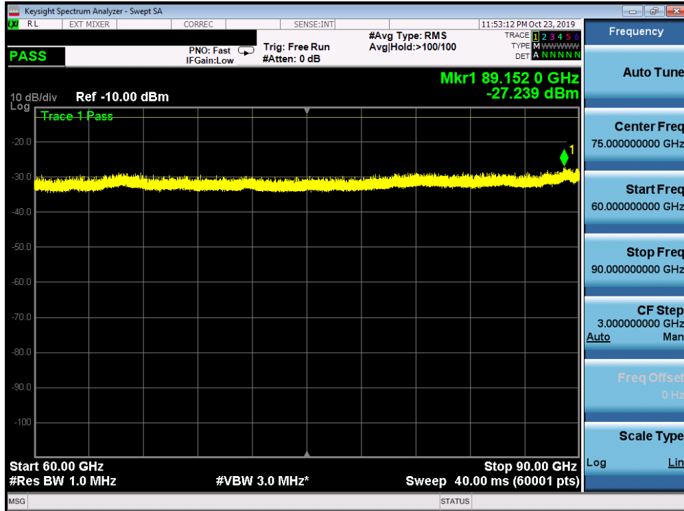
Plot 7-43. HBF Antenna Radiated Spurious Plot 60-90 GHz (1CC QPSK Low Channel H Beam)
