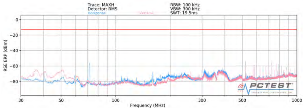
Plot 7-56. Patch Antenna Radiated Spurious Plot 30 MHz - 1 GHz (1CC QPSK Mid Channel V Beam)
