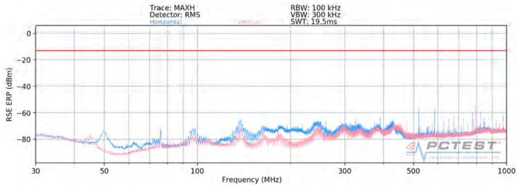
Plot 7-22. HBF Antenna Radiated Spurious Plot 30 MHz - 1 GHz (1CC QPSK Mid Channel V Beam)
