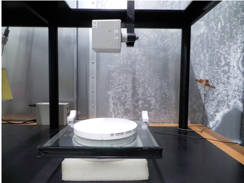
Figure 1. MPE Measurement Setup – Front IDU Face
