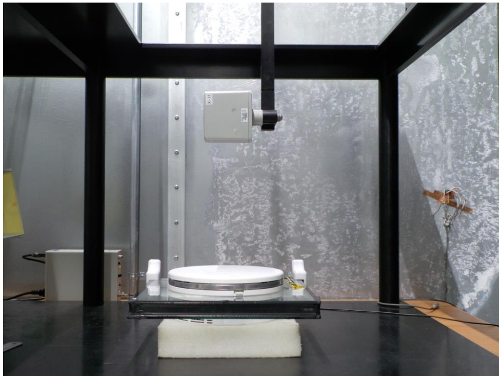
Figure 2. MPE Measurement Setup – Rear IDU Face
