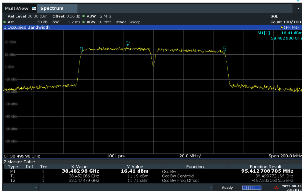
Plot 7-28. Occupied Bandwidth Plot – DFT-s – H-DL Polarization (50MHz-2CC – 16QAM – Mid Channel)
