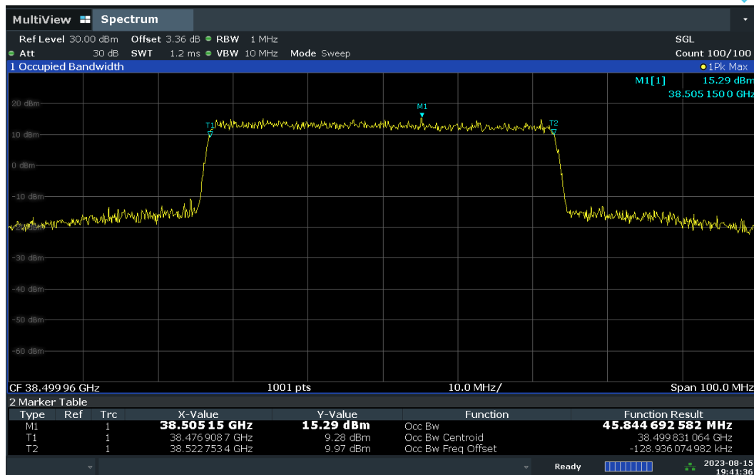
Plot 7-16. Occupied Bandwidth Output at 3dB above AGC Threshold – CP – H-DL Polarization.
