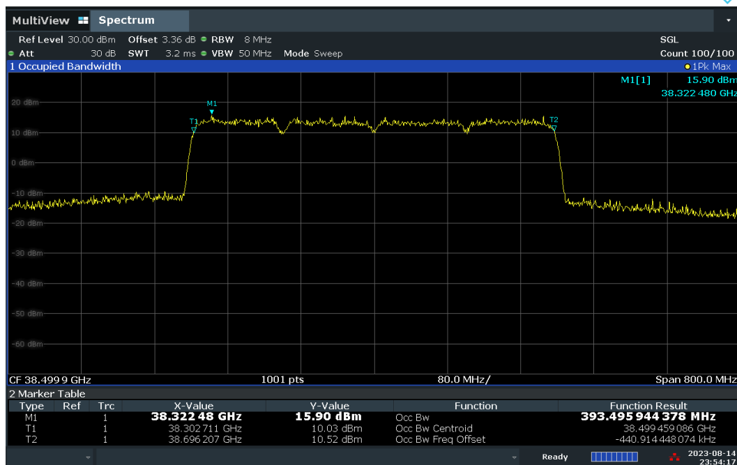
Plot 7-36. Occupied Bandwidth Plot – CP – V-DL Polarization (100MHz-4CC – 16QAM – Mid Channel)
