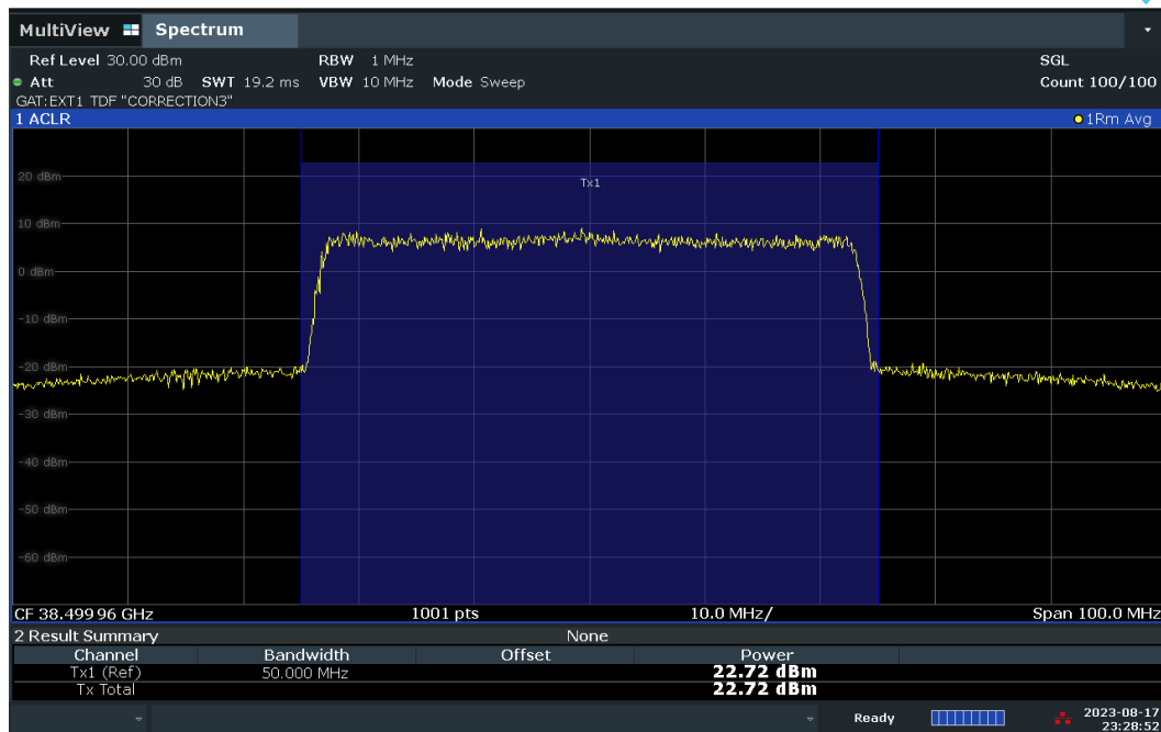
Plot 7-49. Conducted Power Plot – DFT-S – V-DL Polarization (50MHz-1CC – 16QAM – Mid Ch. – Full RB)
