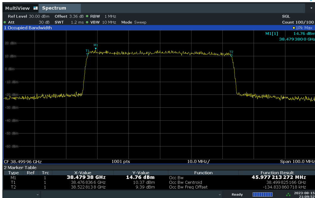
Plot 7-2. Occupied Bandwidth Output at 0.5dB below AGC Threshold – DFT-s – V-DL Polarization.
