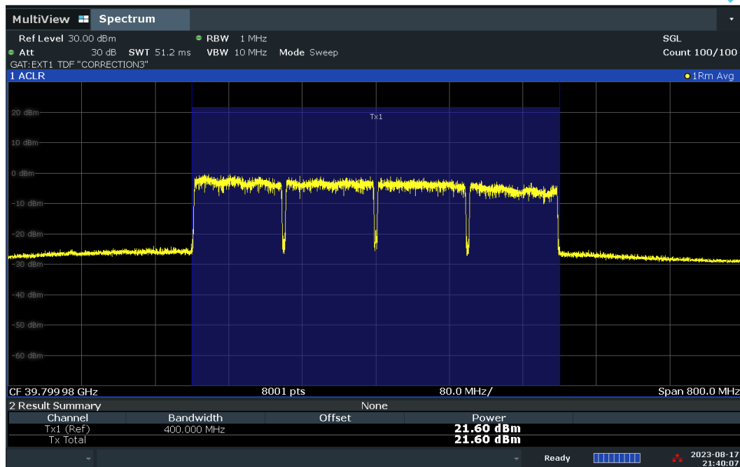
Plot 7-103. Conducted Power Plot – CP – V-DL Polarization (100MHz-4CC – QPSK – High Ch. – Full RB)
