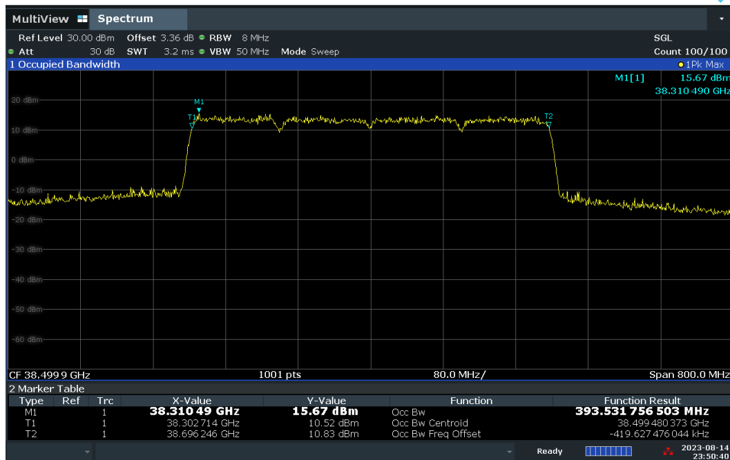
Plot 7-35. Occupied Bandwidth Plot – CP – V-DL Polarization (100MHz-4CC – QPSK – Mid Channel)
