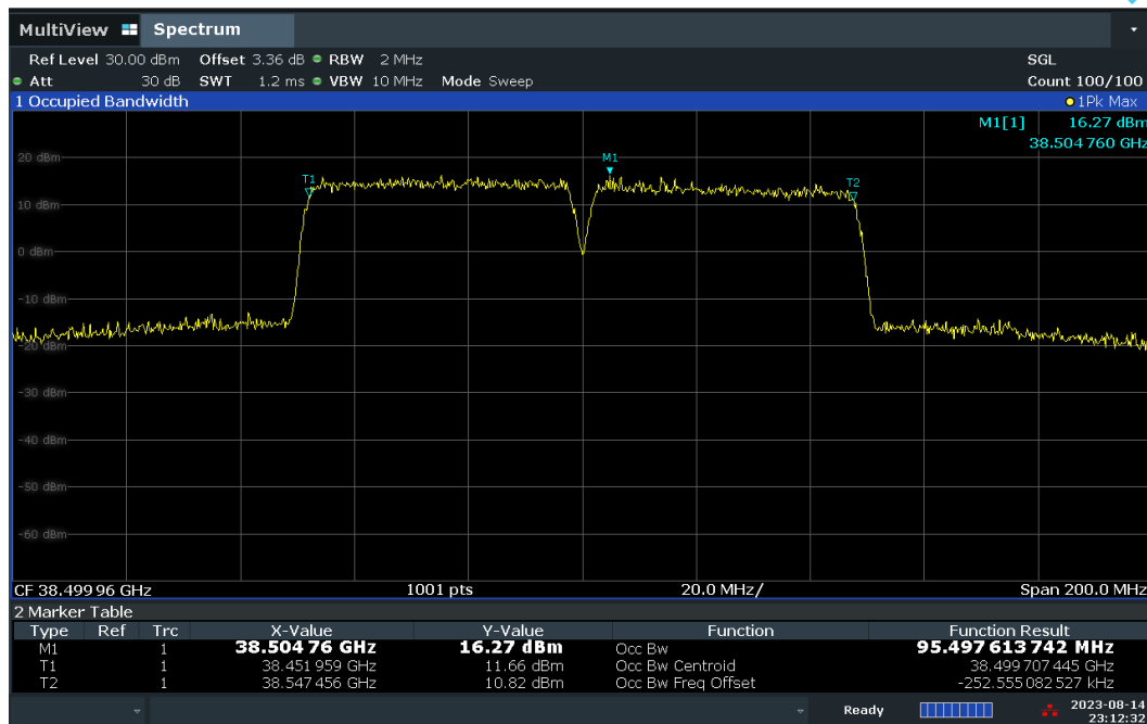
Plot 7-27. Occupied Bandwidth Plot – DFT-s – H-DL Polarization (50MHz-2CC – QPSK – Mid Channel)
