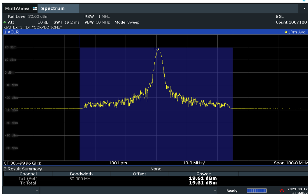
Plot 7-46. Conducted Power Plot – DFT-S – V-DL Polarization (50MHz-1CC – QPSK – Mid Ch. – 1 RB)
