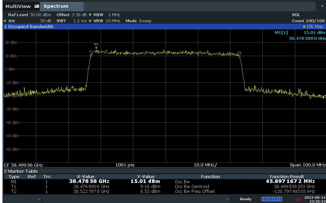
Plot 7-31. Occupied Bandwidth Plot – CP – V-DL Polarization (50MHz-1CC – QPSK – Mid Channel)
