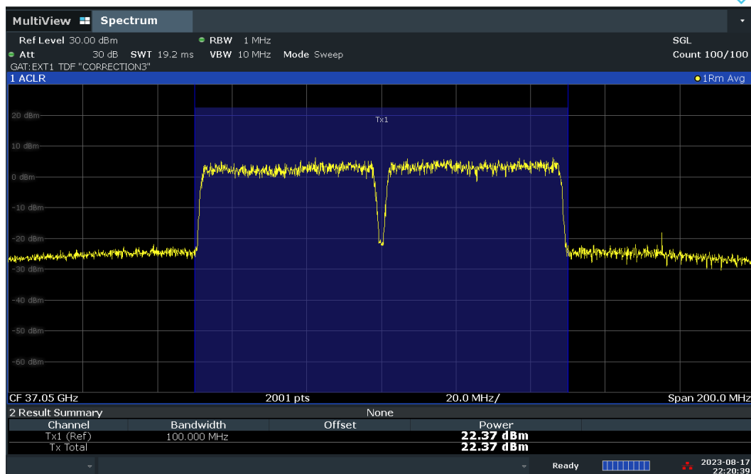
Plot 7-50. Conducted Power Plot – DFT-S – V-DL Polarization (50MHz-2CC – QPSK – Low Ch. – Full RB)
