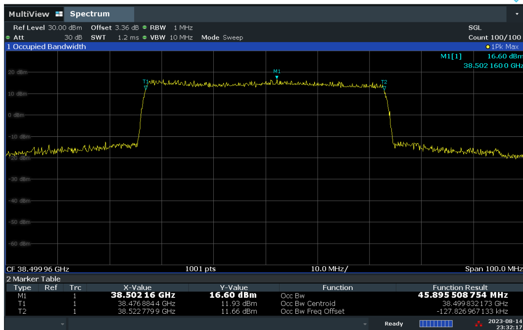
Plot 7-19. Occupied Bandwidth Plot – DFT-s – V-DL Polarization (50MHz-1CC – QPSK – Mid Channel)
