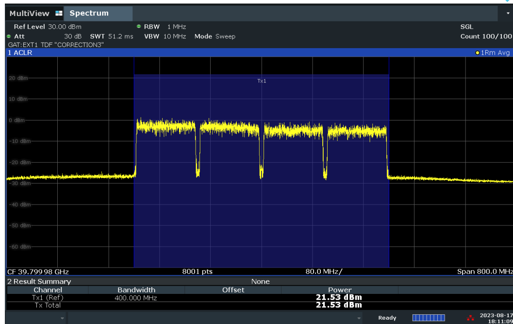
Plot 7-84. Conducted Power Plot – DFT-S – H-DL Polarization (100MHz-4CC – 16QAM – High Ch. – Full RB)
