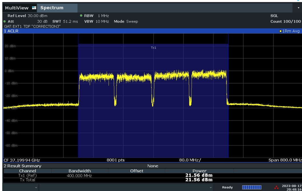
Plot 7-57. Conducted Power Plot – DFT-S – V-DL Polarization (100MHz-4CC – QPSK – Low Ch. – Full RB)
