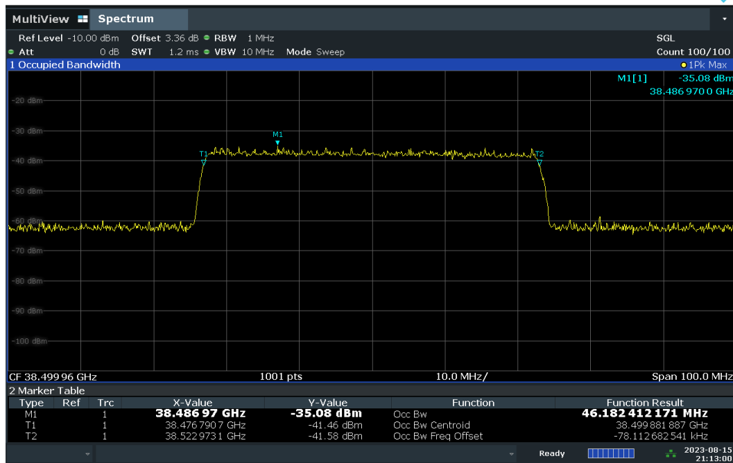
Plot 7-1. Occupied Bandwidth Input at 0.5dB below AGC Threshold – DFT-s – V-DL Polarization.
