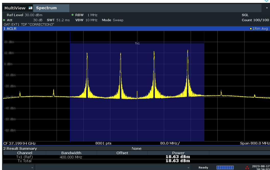
Plot 7-58. Conducted Power Plot – DFT-S – V-DL Polarization (100MHz-4CC – QPSK – Low Ch. – 1RB)
