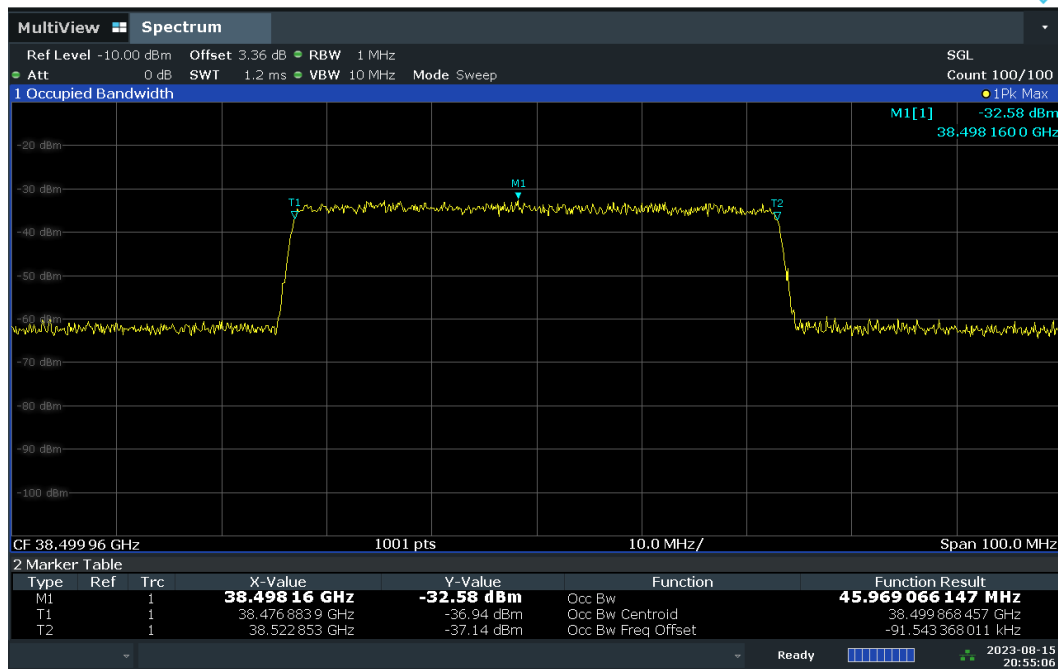
Plot 7-11. Occupied Bandwidth Input at 3dB above AGC Threshold – CP – V-DL Polarization.
