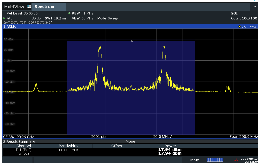
Plot 7-95. Conducted Power Plot – CP – V-DL Polarization (50MHz-2CC – QPSK – Mid Ch. – 1 RB)
