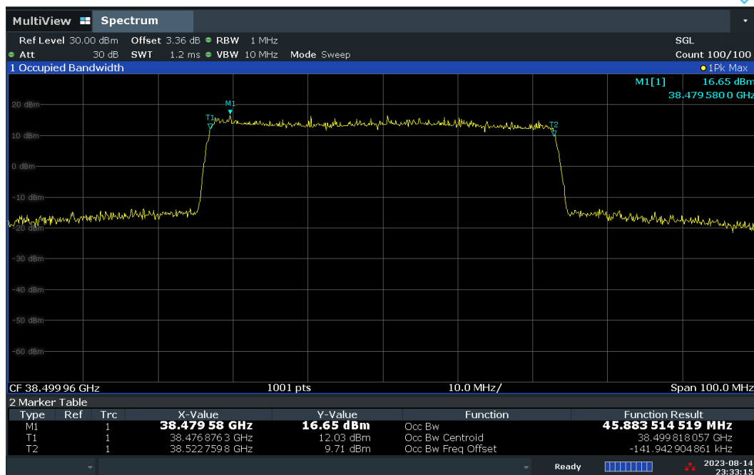
Plot 7-20. Occupied Bandwidth Plot – DFT-s – V-DL Polarization (50MHz-1CC – 16QAM – Mid Channel)
