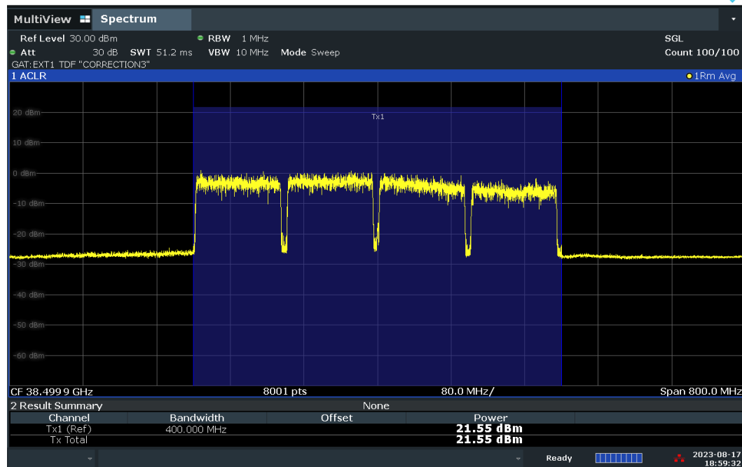
Plot 7-80. Conducted Power Plot – DFT-S – H-DL Polarization (100MHz-4CC – QPSK – Mid Ch. – Full RB)
