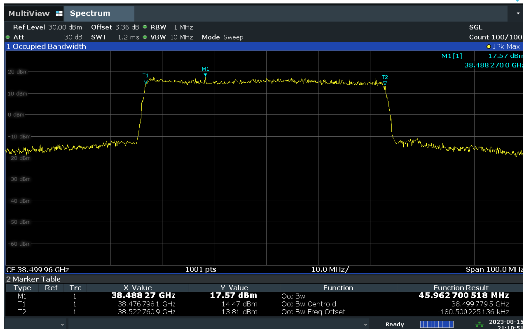
Plot 7-4. Occupied Bandwidth Output at 3dB above AGC Threshold – DFT-s – V-DL Polarization.
