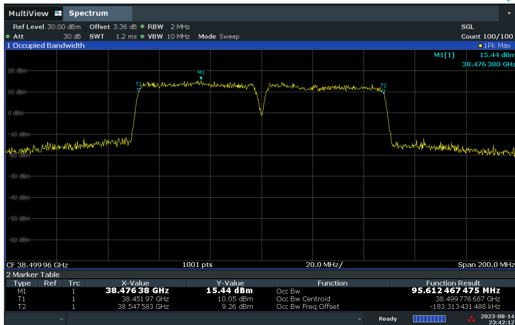
Plot 7-33. Occupied Bandwidth Plot – CP – V-DL Polarization (50MHz-2CC – QPSK – Mid Channel)
