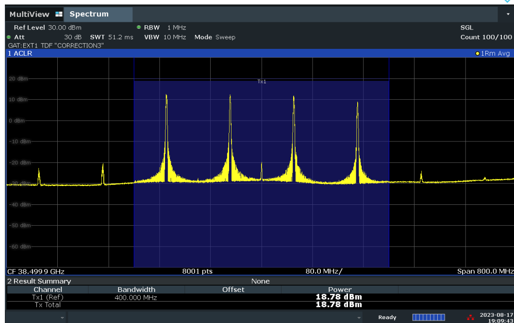
Plot 7-81. Conducted Power Plot – DFT-S – H-DL Polarization (100MHz-4CC – QPSK – Mid Ch. – 1 RB)
