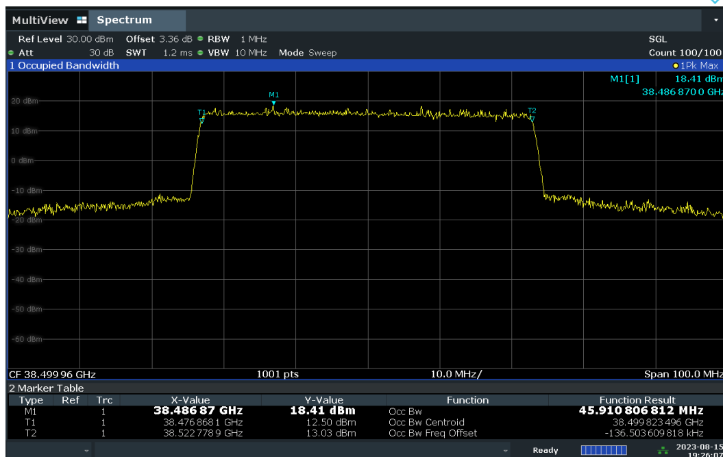
Plot 7-8. Occupied Bandwidth Output at 3dB above AGC Threshold – DFT-s – H-DL Polarization.
