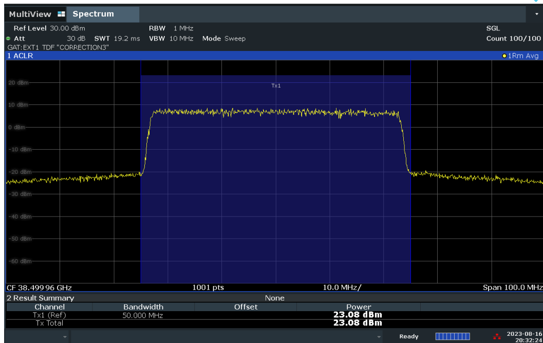
Plot 7-66. Conducted Power Plot – DFT-S – H-DL Polarization (50MHz-1CC – QPSK – Mid Ch. – Full RB)
