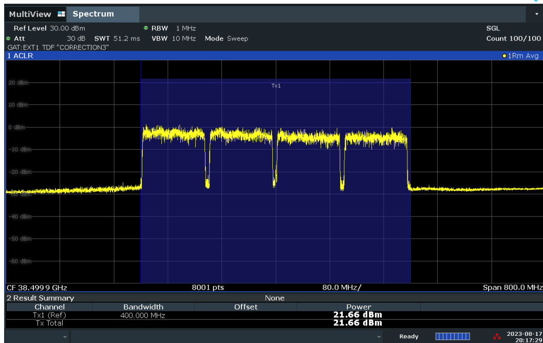
Plot 7-59. Conducted Power Plot – DFT-S – V-DL Polarization (100MHz-4CC – QPSK – Mid Ch. – Full RB)
