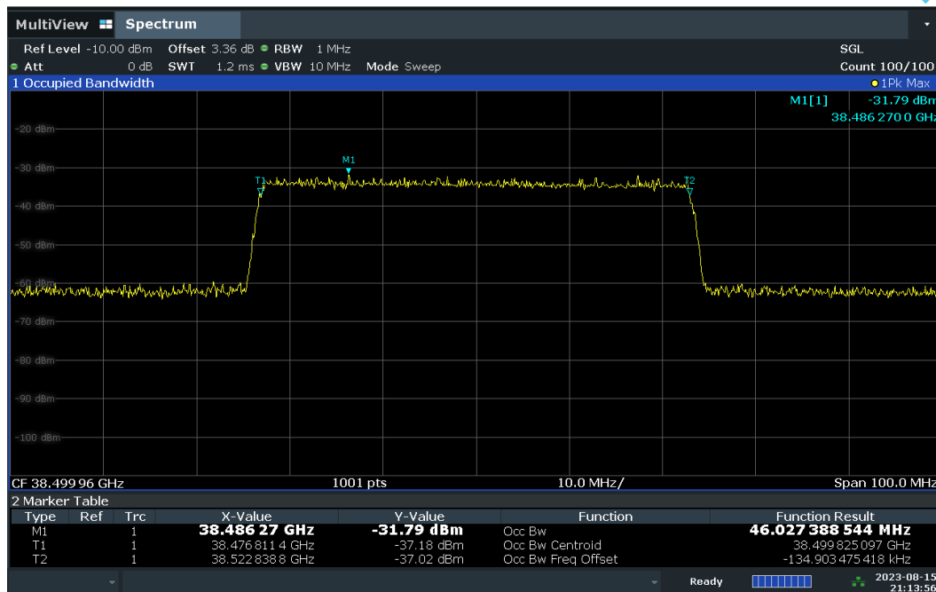
Plot 7-3. Occupied Bandwidth Input at 3dB above AGC Threshold – DFT-s – V-DL Polarization.
