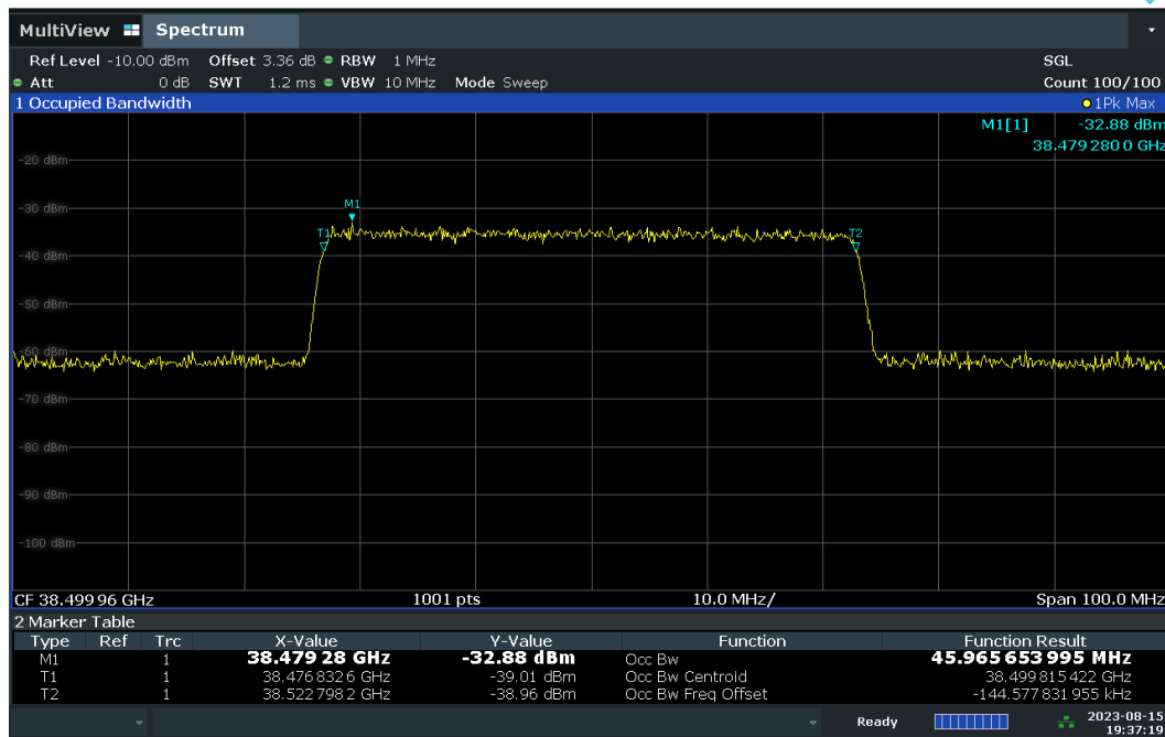
Plot 7-15. Occupied Bandwidth Input at 3dB above AGC Threshold – CP – H-DL Polarization.
