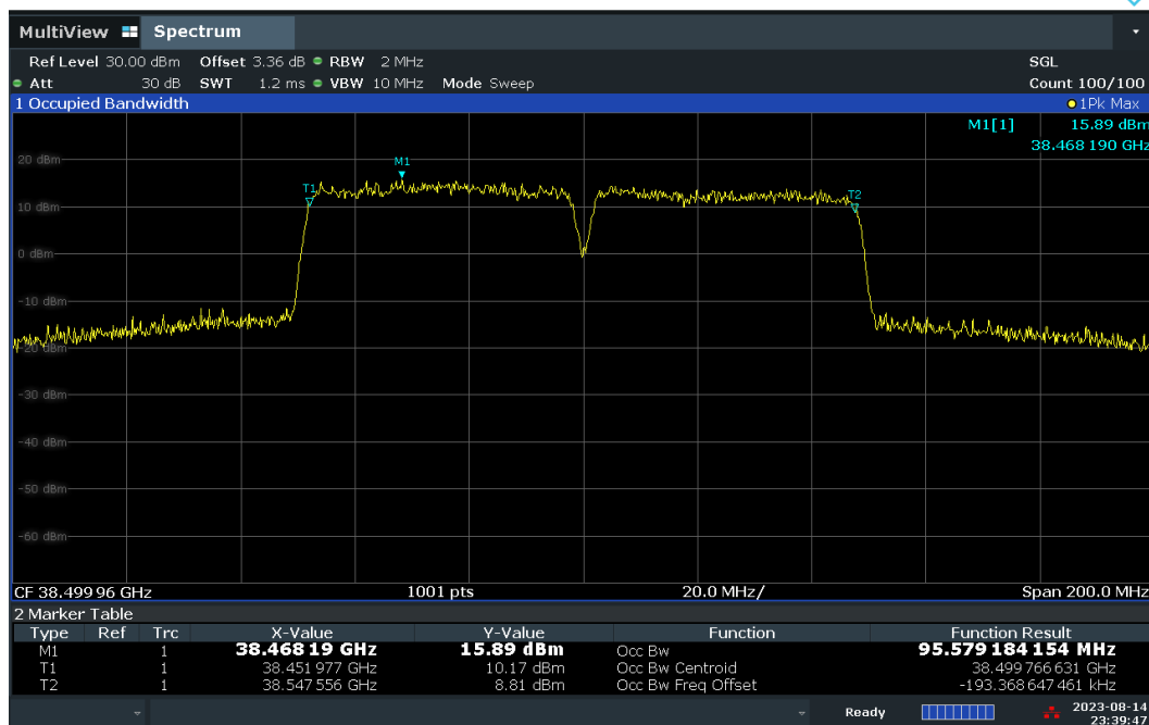
Plot 7-34. Occupied Bandwidth Plot – CP – V-DL Polarization (50MHz-2CC – 16QAM – Mid Channel)
