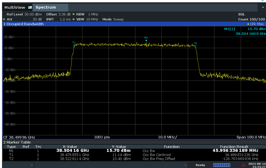
Plot 7-38. Occupied Bandwidth Plot – CP – H-DL Polarization (50MHz-1CC – 16QAM – Mid Channel)
