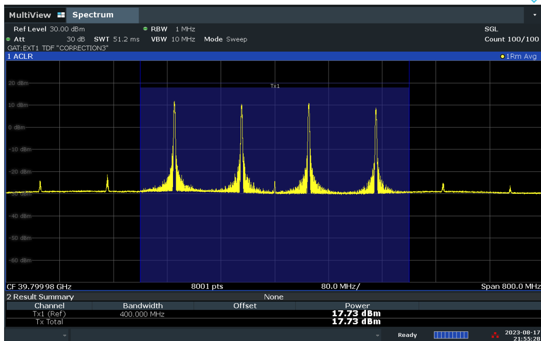
Plot 7-104. Conducted Power Plot – CP – V-DL Polarization (100MHz-4CC – QPSK – High Ch. – 1 RB)
