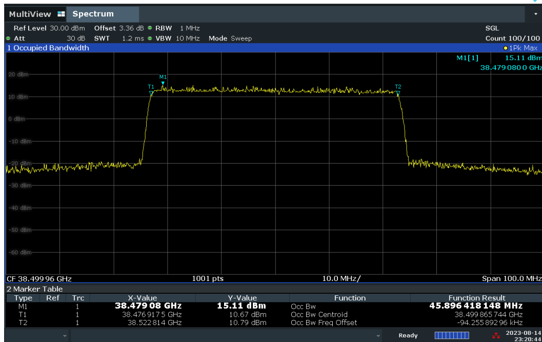
Plot 7-25. Occupied Bandwidth Plot – DFT-s – H-DL Polarization (50MHz-1CC – QPSK – Mid Channel)
