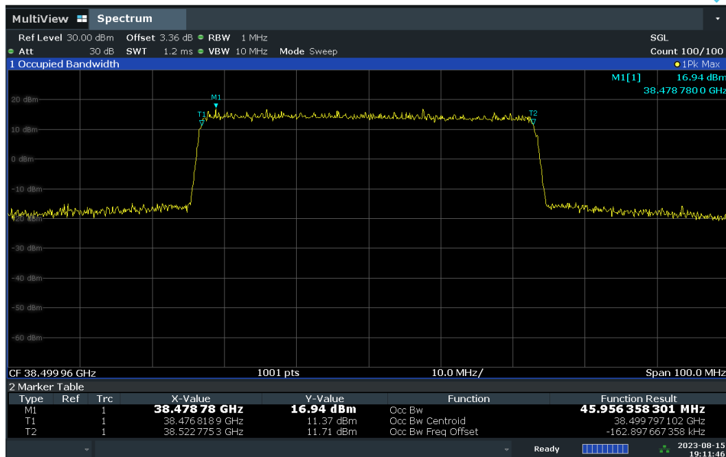
Plot 7-6. Occupied Bandwidth Output at 0.5dB below AGC Threshold – DFT-s – H-DL Polarization.
