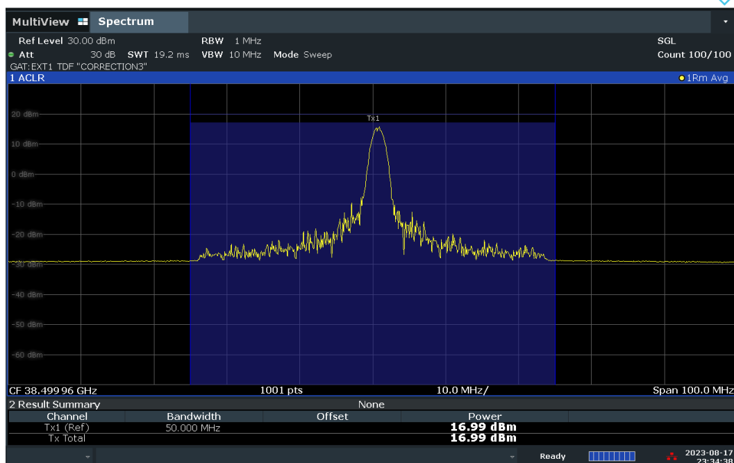
Plot 7-88. Conducted Power Plot – CP – V-DL Polarization (50MHz-1CC – QPSK – Mid Ch. – 1 RB)
