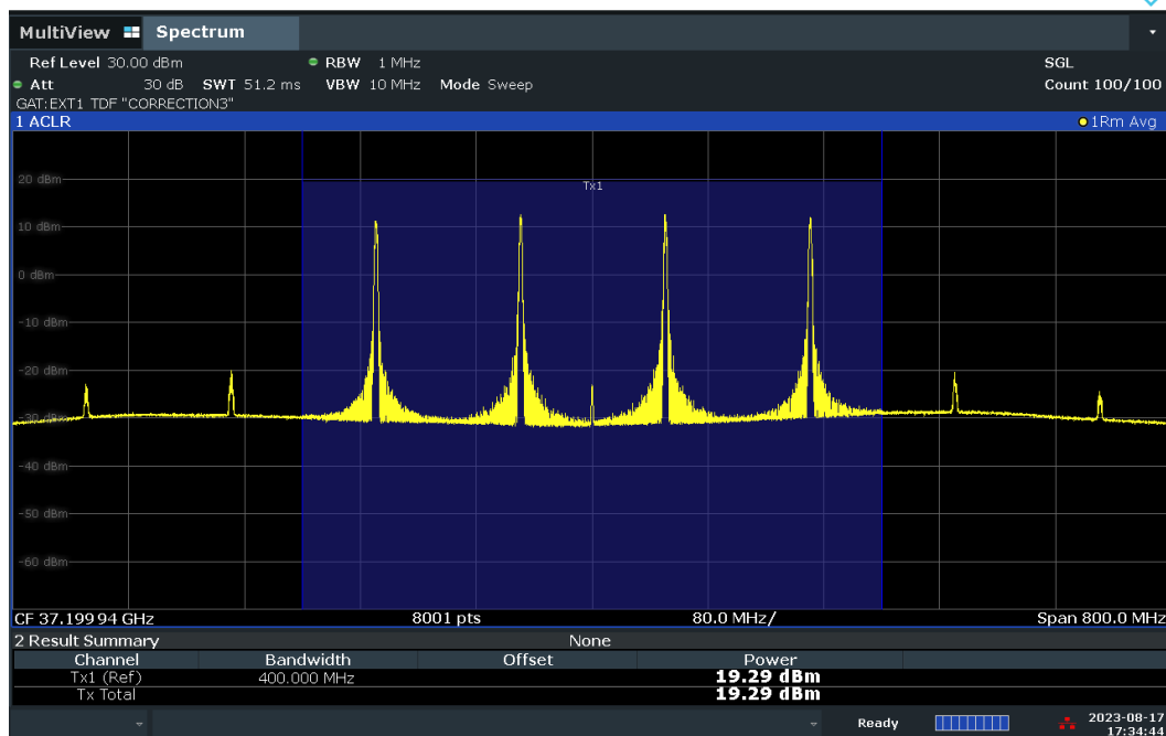
Plot 7-79. Conducted Power Plot – DFT-S – H-DL Polarization (100MHz-4CC – QPSK – Low Ch. – 1RB)
