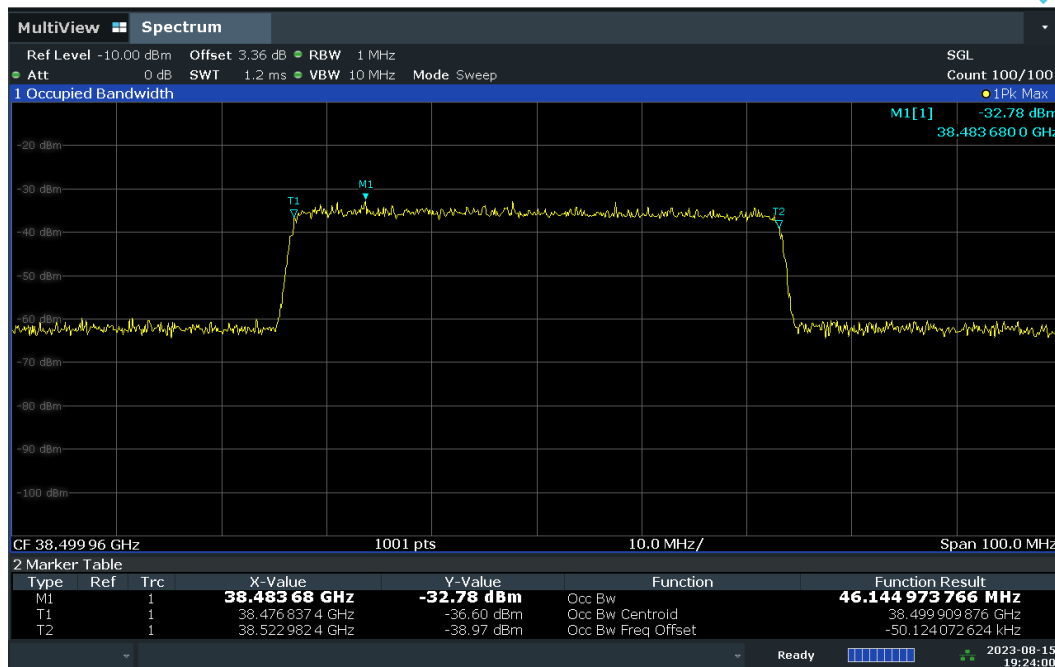
Plot 7-7. Occupied Bandwidth Input at 3dB above AGC Threshold – DFT-s – H-DL Polarization.
