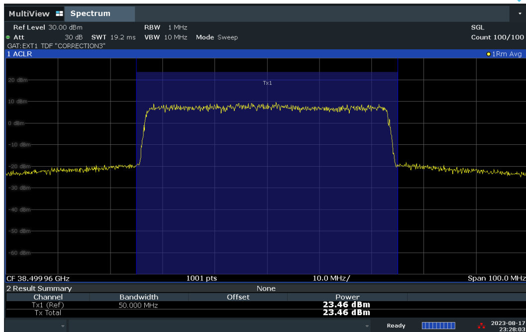
Plot 7-45. Conducted Power Plot – DFT-S – V-DL Polarization (50MHz-1CC – QPSK – Mid Ch. – Full RB)
