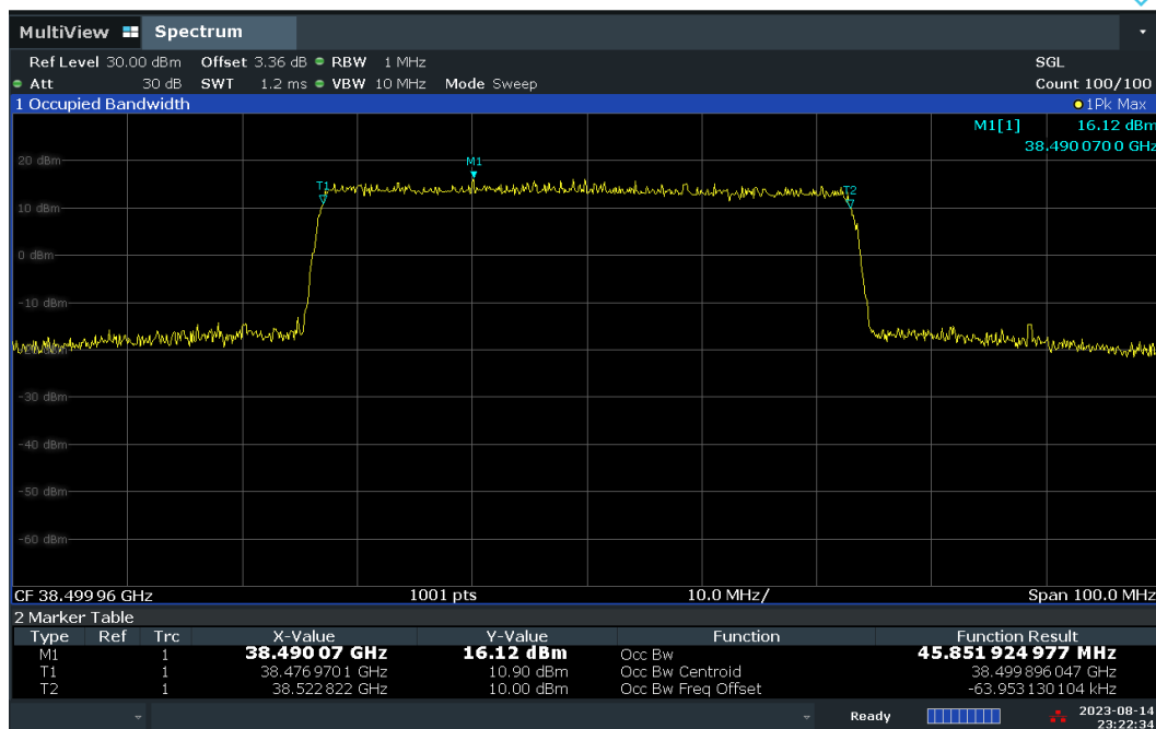
Plot 7-26. Occupied Bandwidth Plot – DFT-s – H-DL Polarization (50MHz-1CC – 16QAM – Mid Channel)
