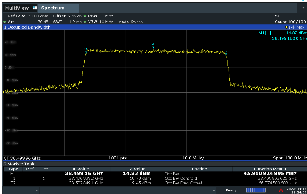
Plot 7-37. Occupied Bandwidth Plot – CP – H-DL Polarization (50MHz-1CC – QPSK – Mid Channel)
