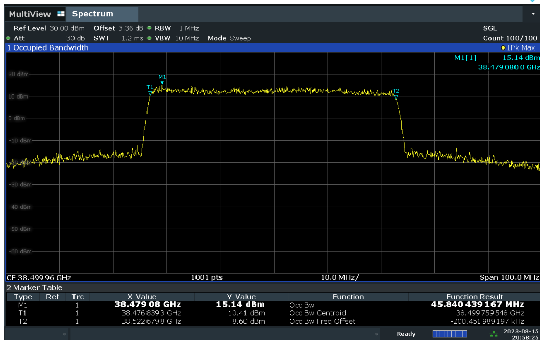
Plot 7-12. Occupied Bandwidth Output at 3dB above AGC Threshold – CP – V-DL Polarization.
