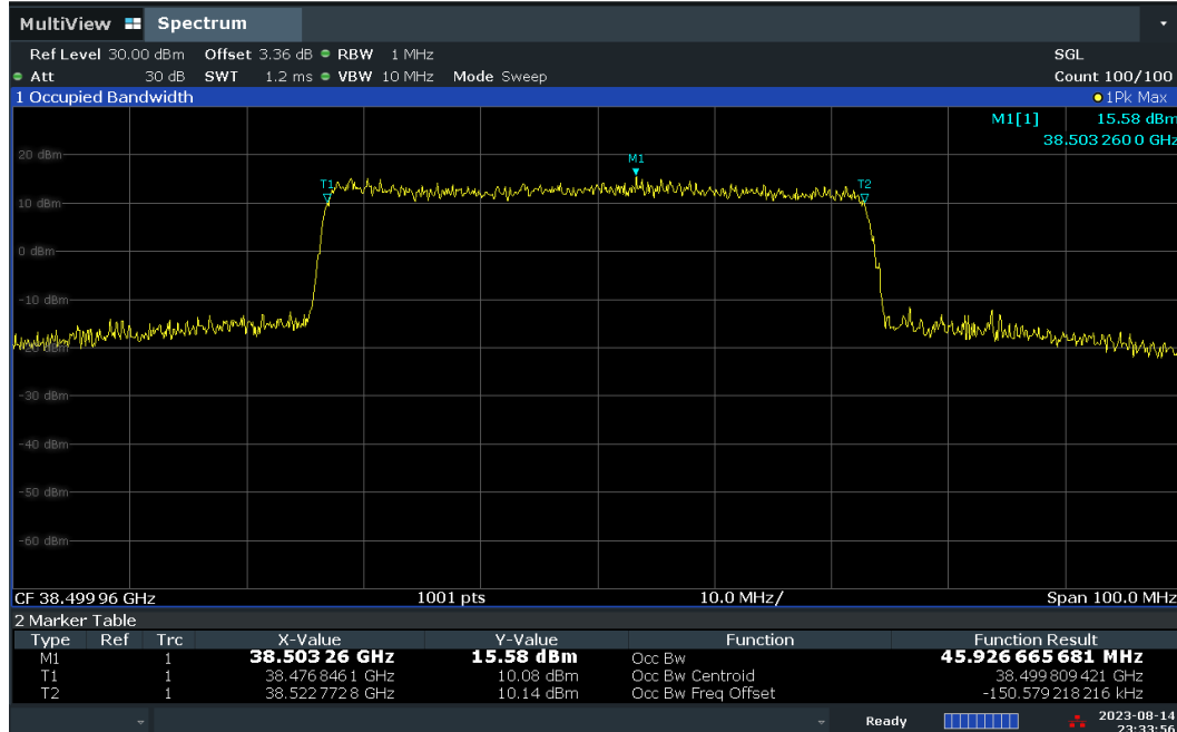
Plot 7-32. Occupied Bandwidth Plot – CP – V-DL Polarization (50MHz-1CC – 16QAM – Mid Channel)
