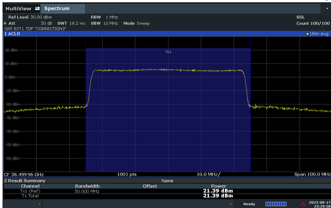
Plot 7-87. Conducted Power Plot – CP – V-DL Polarization (50MHz-1CC – QPSK – Mid Ch. – Full RB)
