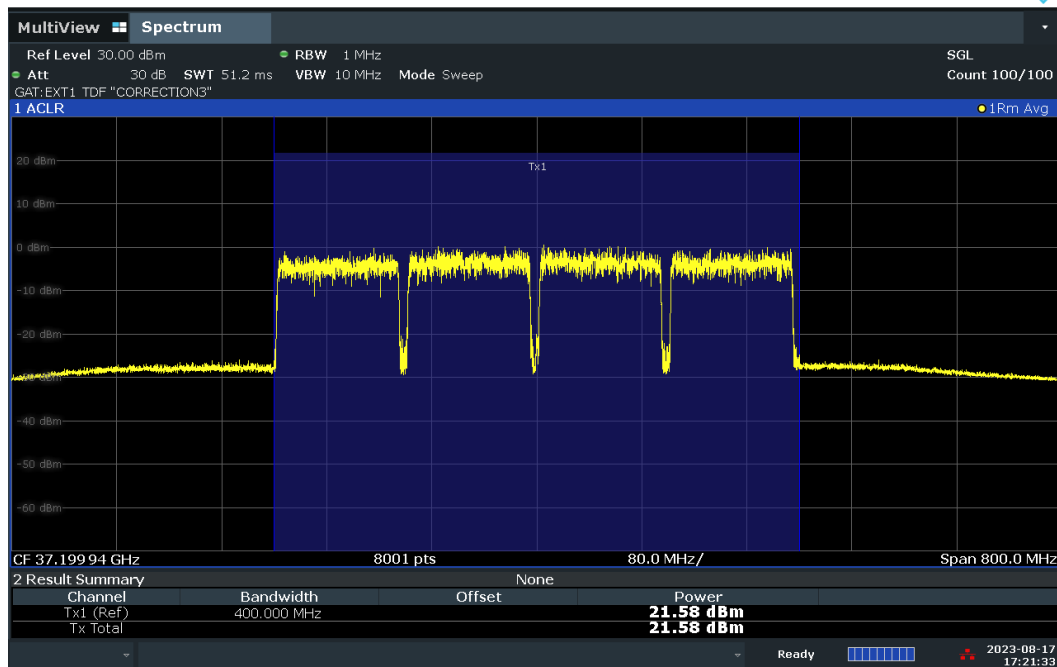
Plot 7-78. Conducted Power Plot – DFT-S – H-DL Polarization (100MHz-4CC – QPSK – Low Ch. – Full RB)
