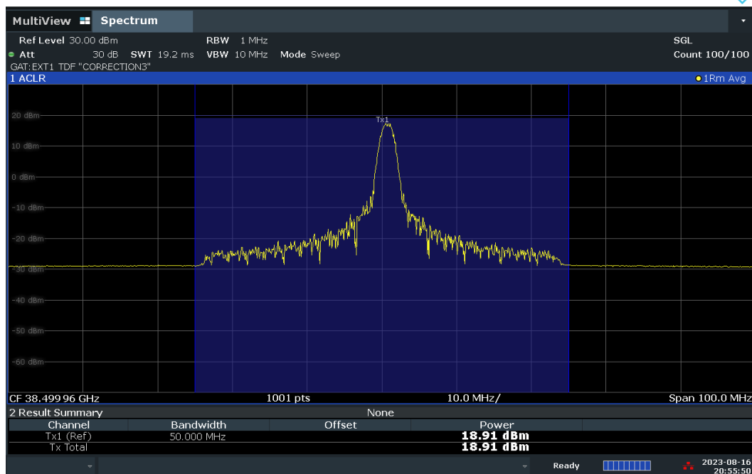
Plot 7-67. Conducted Power Plot – DFT-S – H-DL Polarization (50MHz-1CC – QPSK – Mid Ch. – 1 RB)
