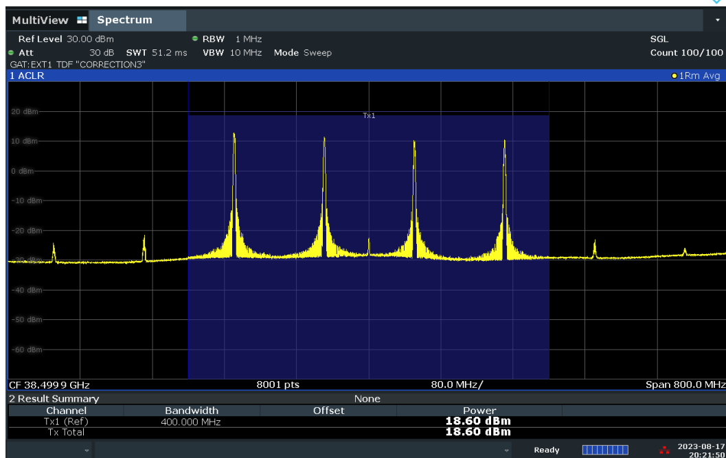
Plot 7-60. Conducted Power Plot – DFT-S – V-DL Polarization (100MHz-4CC – QPSK – Mid Ch. – 1 RB)
