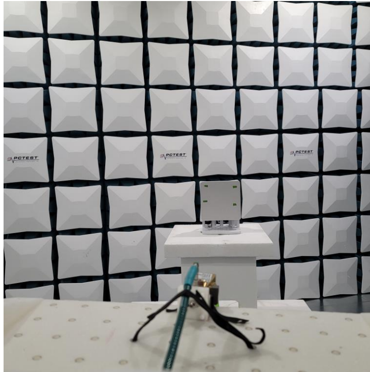
Setup 5. Test Setup 18-40GHz - SU
