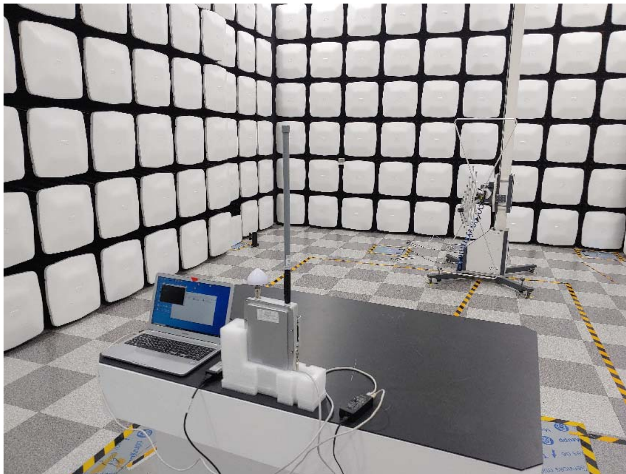
Radiated RF measurement (30 MHz ~ 1 GHz)
