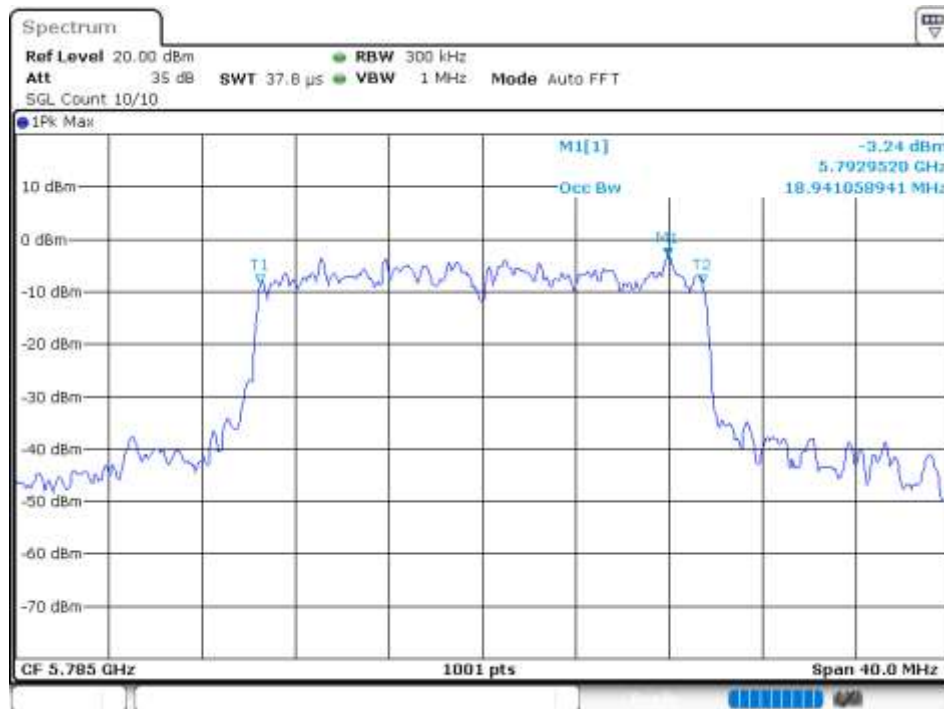
-26 dB BW NVNT 802.11ax20 5785MHz Ant 3
