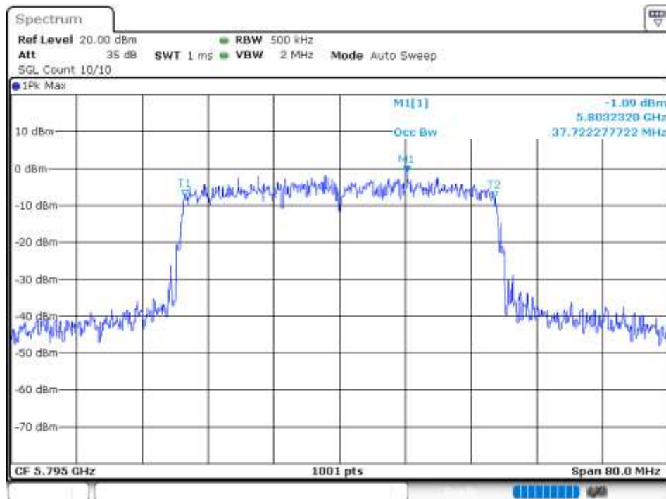
-26 dB BW NVNT 802.11ax40 5795MHz Ant 3
