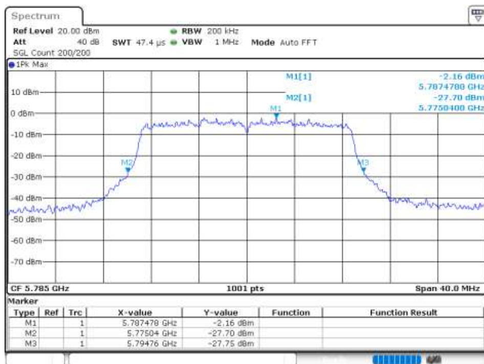
-26 dB BW NVNT 802.11ac20 5785MHz Ant 0
