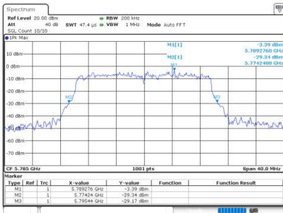
-26 dB BW NVNT 802.11ax20 5785MHz Ant 0
