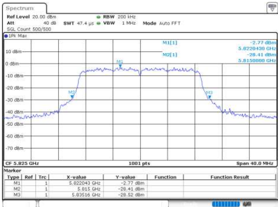
-26 dB BW NVNT 802.11n(HT20) 5825MHz Ant 0
