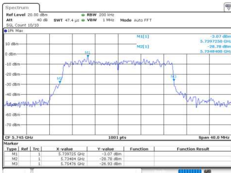
-26 dB BW NVNT 802.11ax20 5745MHz Ant 0
