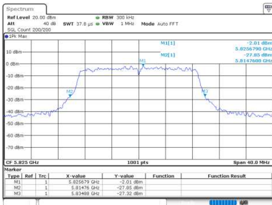
-26 dB BW NVNT 802.11ac20 5825MHz Ant 3
