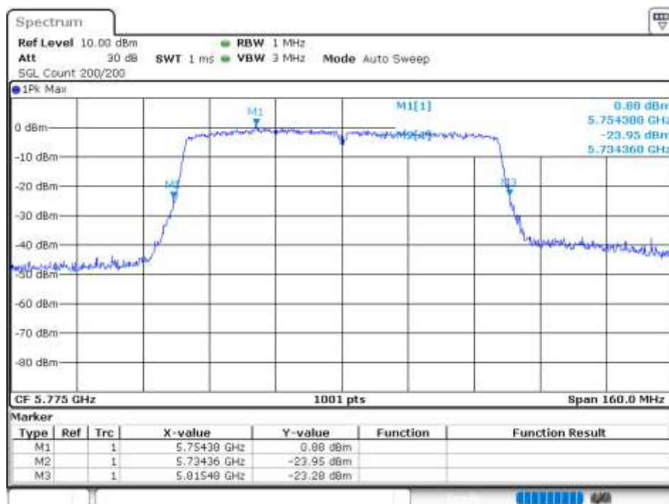
-26 dB BW NVNT 802.11ac80 5775MHz Ant 0
