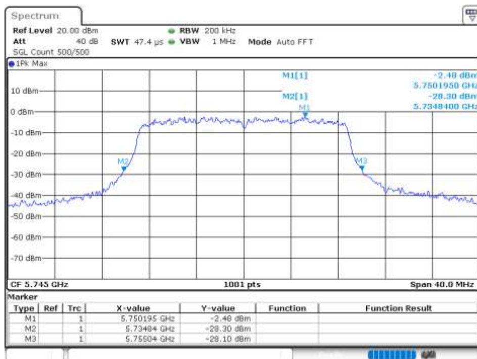
-26 dB BW NVNT 802.11n(HT20) 5745MHz Ant 3
