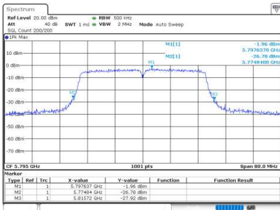
-26 dB BW NVNT 802.11ac40 5795MHz Ant 3
