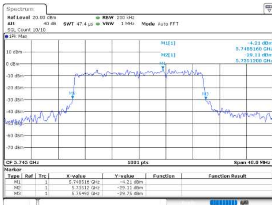
-26 dB BW NVNT 802.11ax20 5745MHz Ant 3
