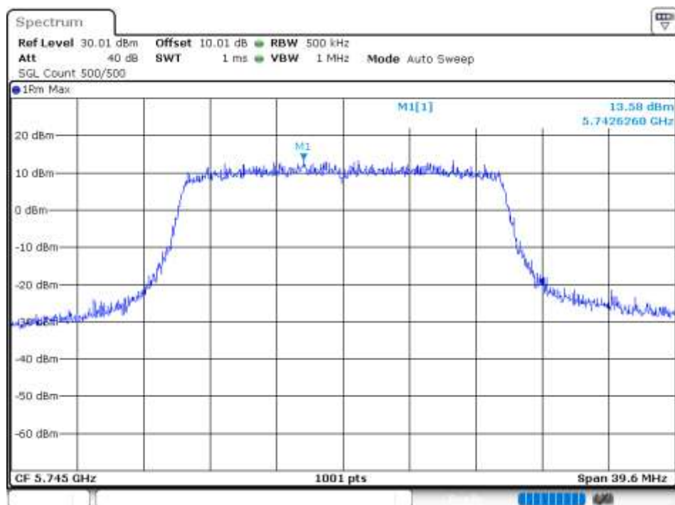
PSD NVNT 802.11ax20 5745MHz Ant 3
