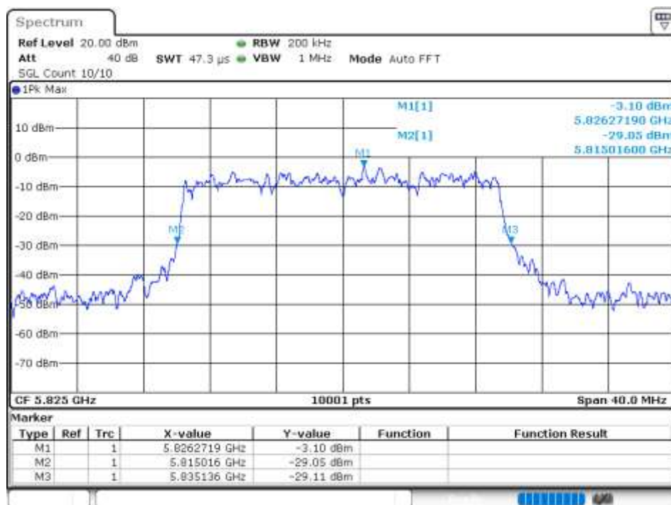
-26 dB BW NVNT 802.11ax20 5825MHz Ant 0
