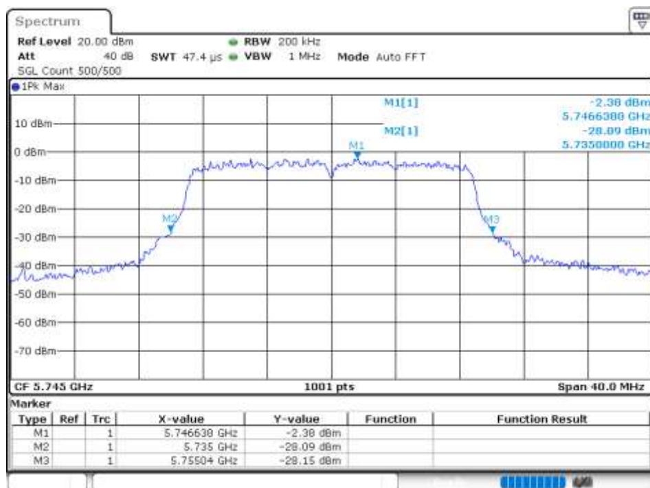
-26 dB BW NVNT 802.11ac20 5745MHz Ant 3
