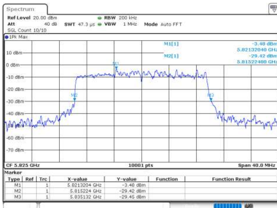
-26 dB BW NVNT 802.11ax20 5825MHz Ant 3
