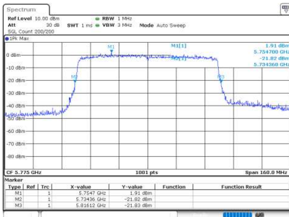
-26 dB BW NVNT 802.11ax80 5775MHz Ant 0
