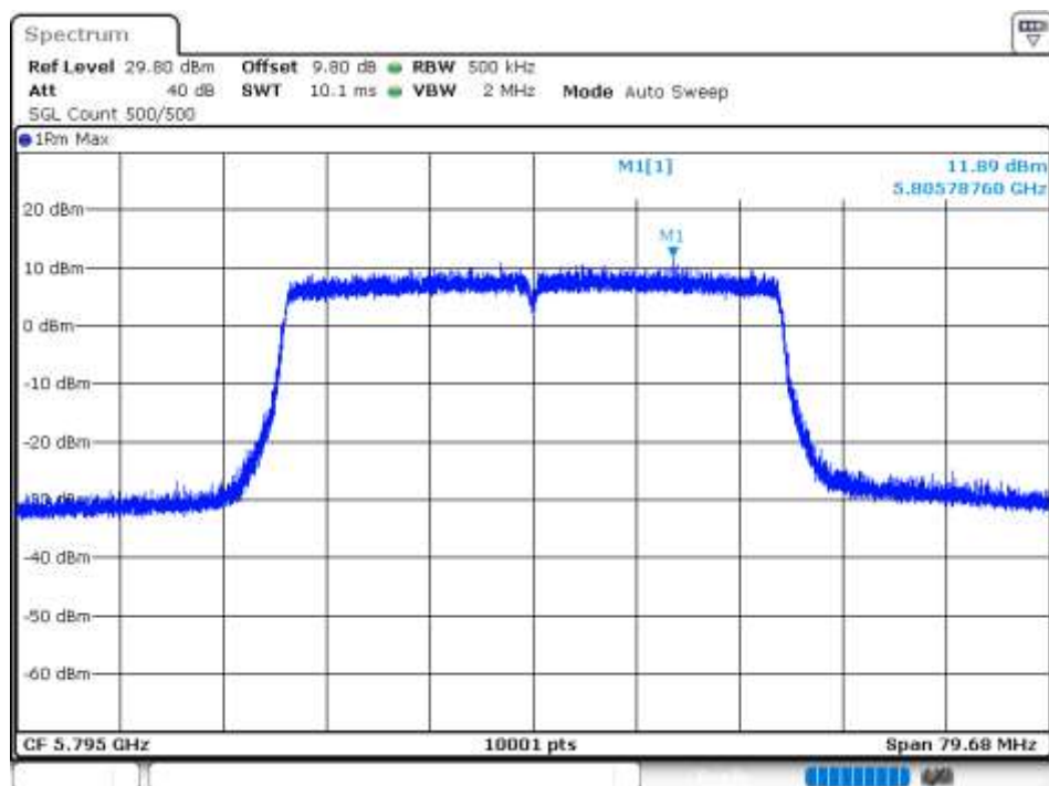
PSD NVNT 802.11ax40 5795MHz Ant 0
