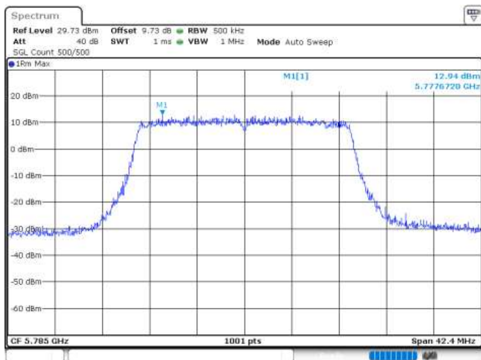
PSD NVNT 802.11ax20 5785MHz Ant 0
