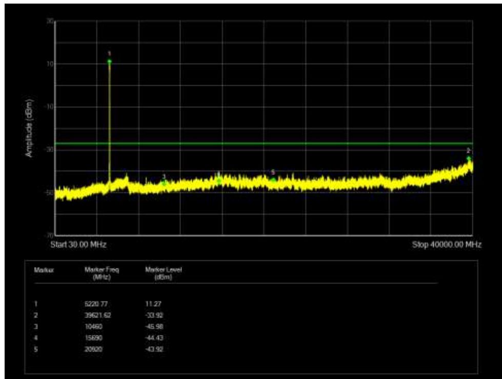
Tx. Spurious NVNT 802.11ax80 5210MHz Ant 4 Emission
