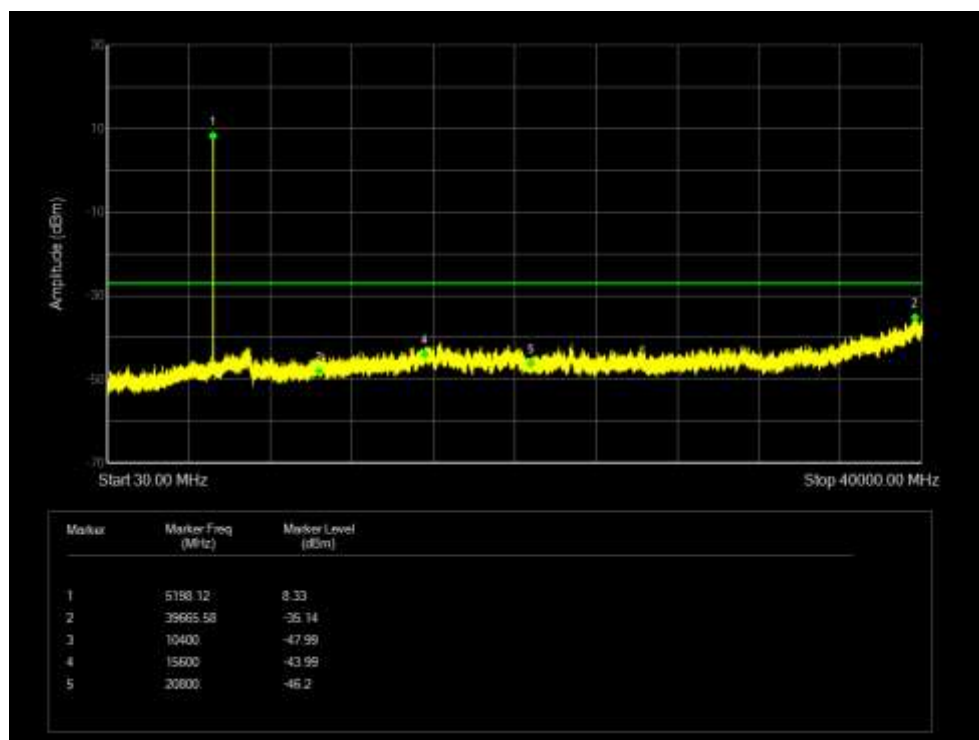
Tx. Spurious NVNT 802.11ac20 5240MHz Ant 5 Emission
