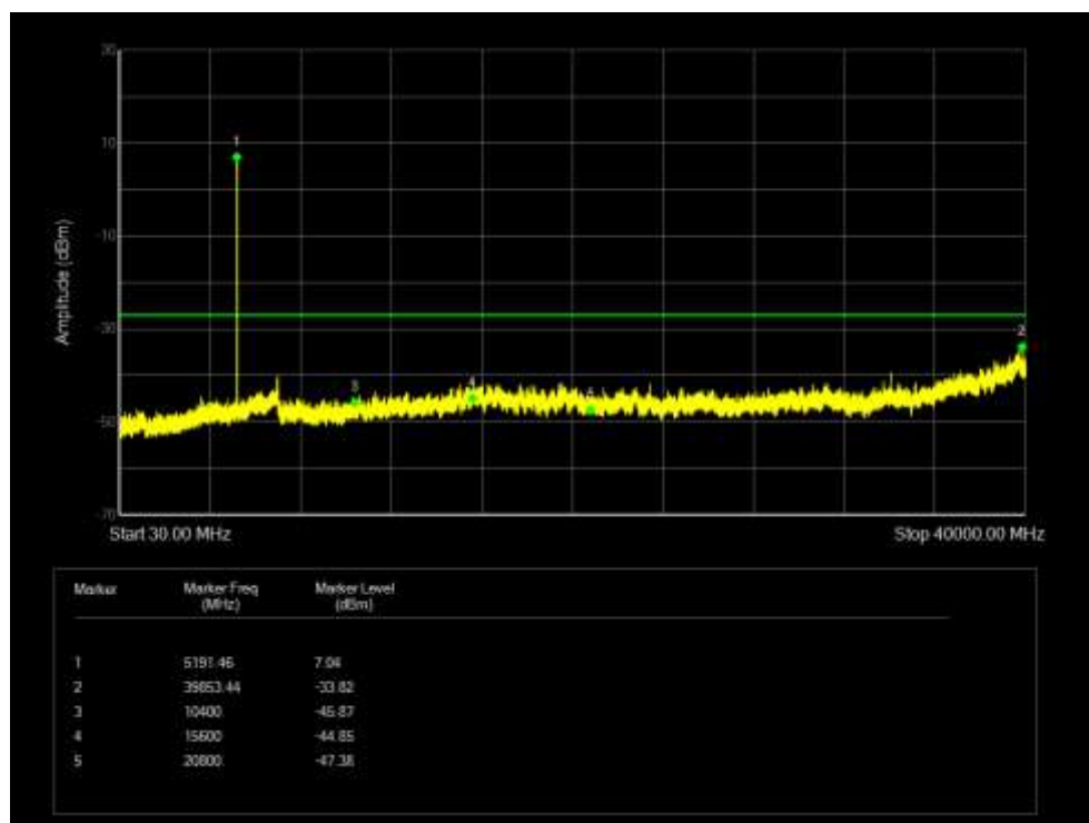
Tx. Spurious NVNT 802.11ax20 5240MHz Ant 5 Emission
