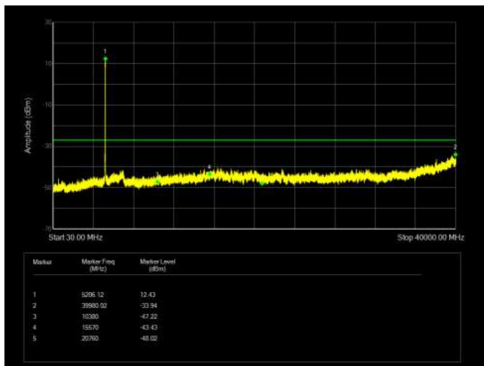
Tx. Spurious NVNT 802.11n(HT40) 5230MHz Ant 7 Emission
