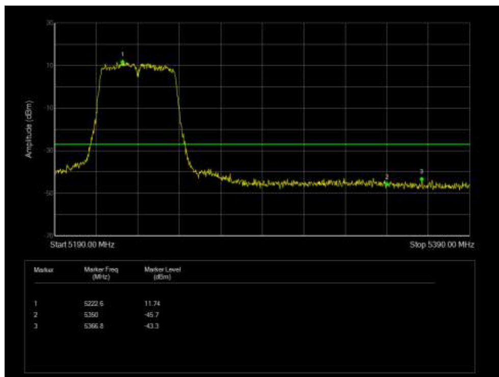
Band Edge NVNT 802.11n(HT40) 5190MHz Low Ant 7
