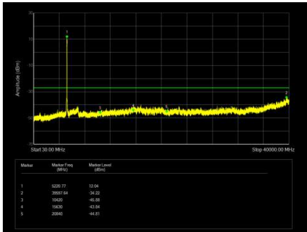
Tx. Spurious NVNT 802.11ax80 5210MHz Ant 6 Emission
