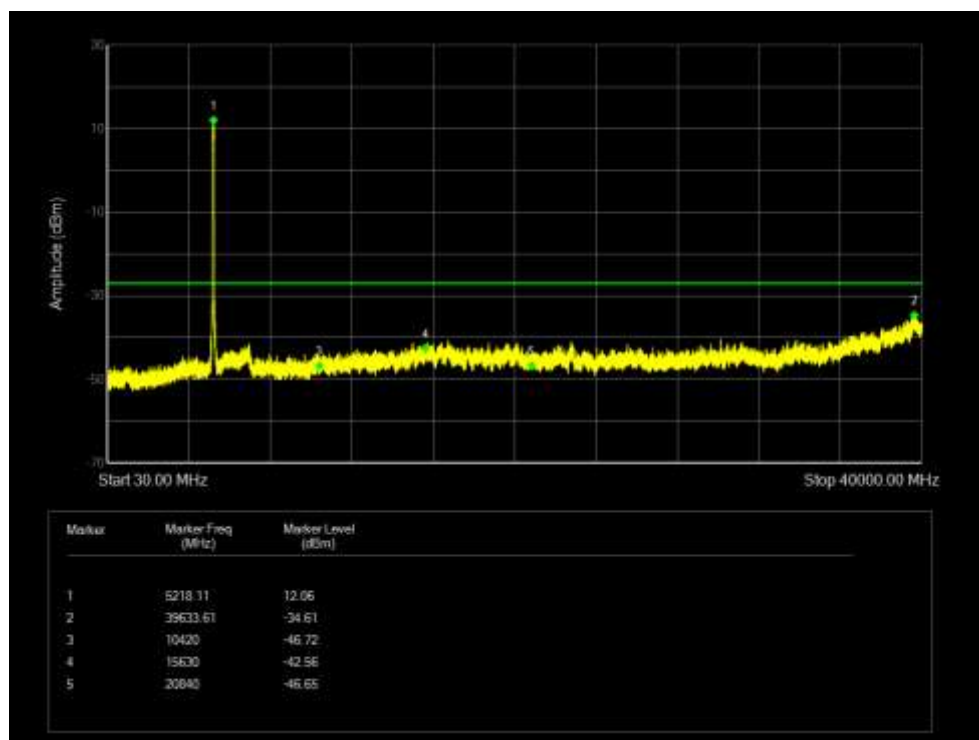
Tx. Spurious NVNT 802.11ac80 5210MHz Ant 7 Emission
