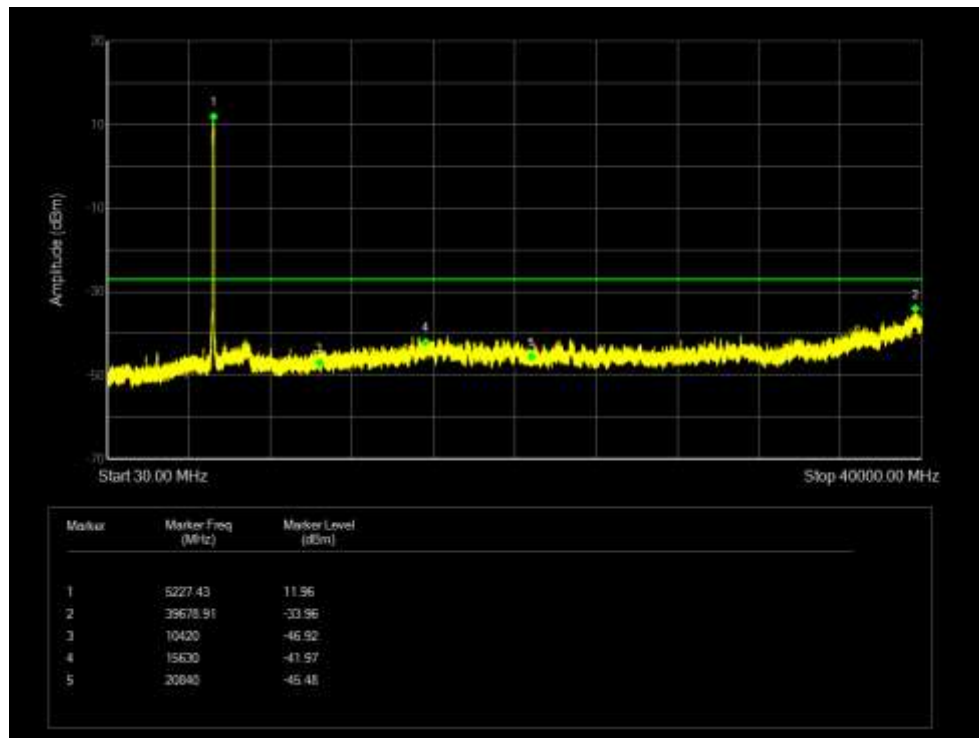
Tx. Spurious NVNT 802.11n(HT20) 5180MHz Ant 4 Emission
