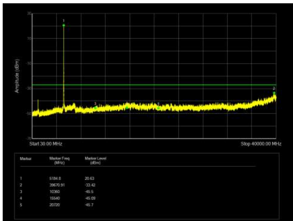
Tx. Spurious NVNT 802.11a 5180MHz Ant 4 Emission
