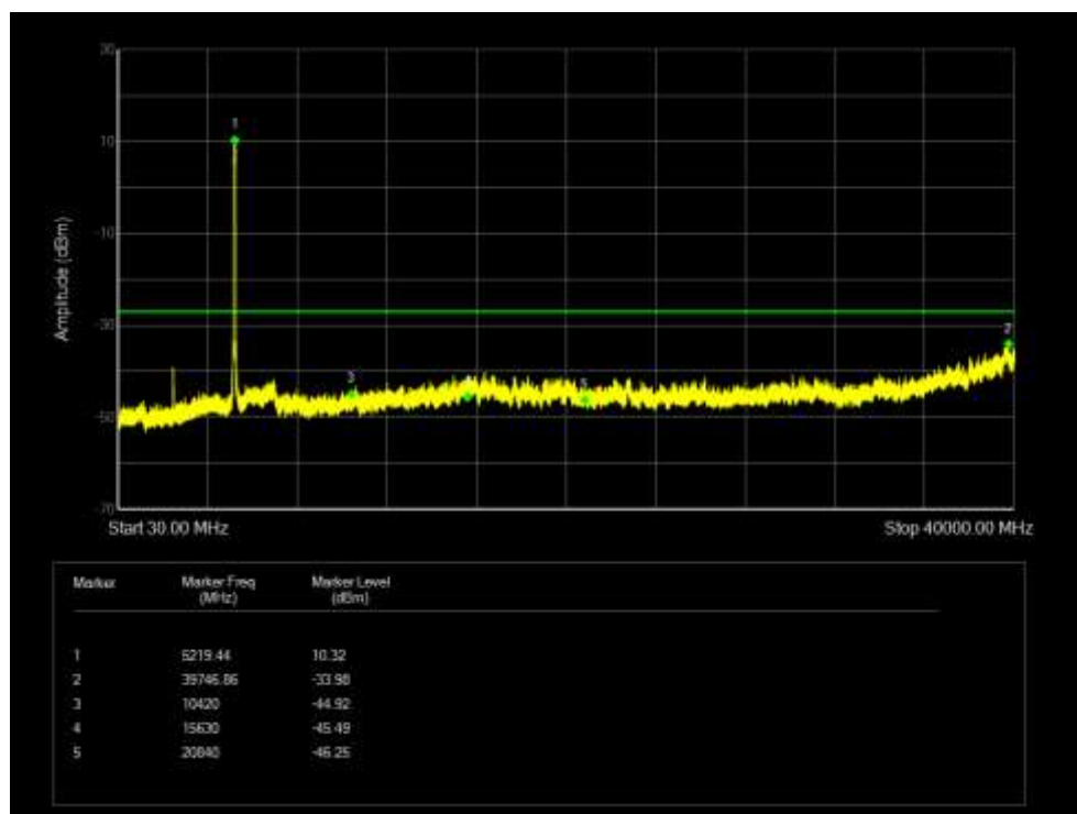
Tx. Spurious NVNT 802.11ax80 5210MHz Ant 5 Emission
