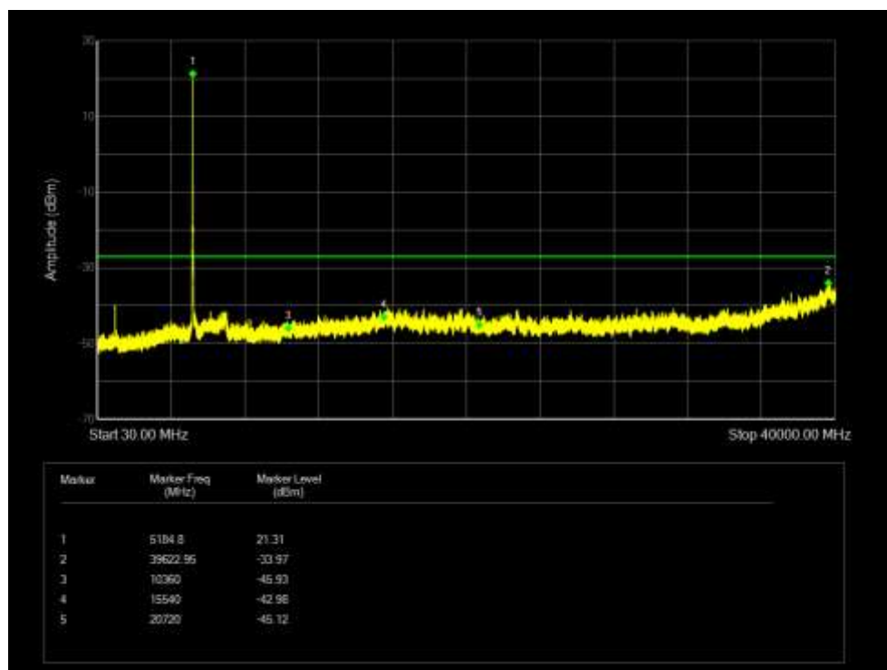
Tx. Spurious NVNT 802.11a 5200MHz Ant 6 Emission
