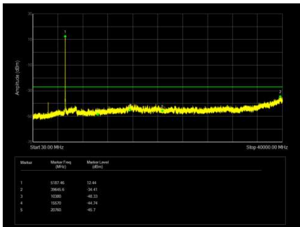
Tx. Spurious NVNT 802.11n(HT40) 5230MHz Ant 4 Emission
