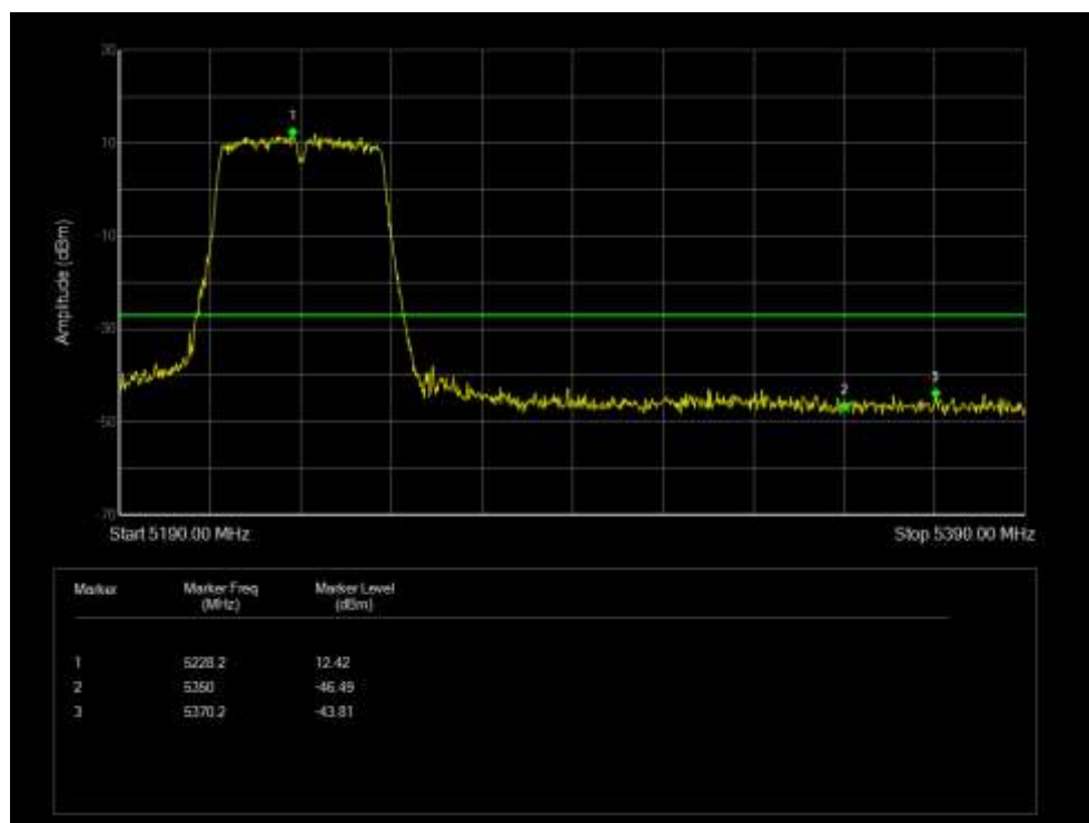
Band Edge NVNT 802.11n(HT40) 5230MHz High Ant 7
