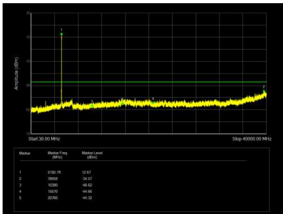
Tx. Spurious NVNT 802.11ac40 5230MHz Ant 7 Emission
