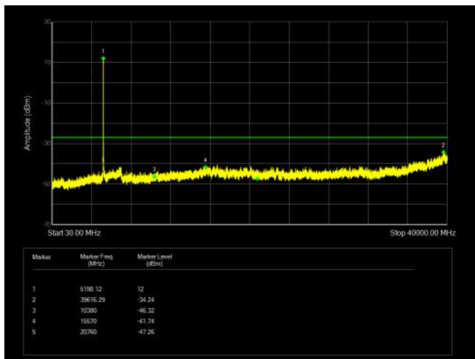
Tx. Spurious NVNT 802.11n(HT40) 5230MHz Ant 6 Emission
