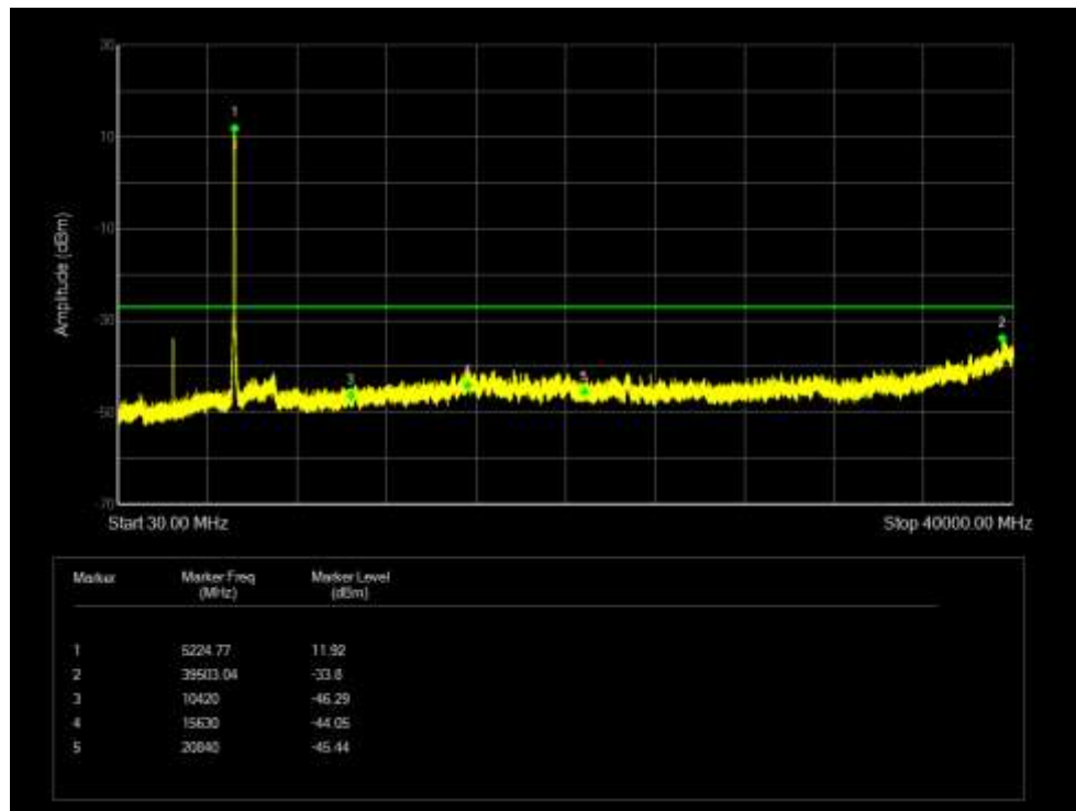
Tx. Spurious NVNT 802.11ac80 5210MHz Ant 6 Emission
