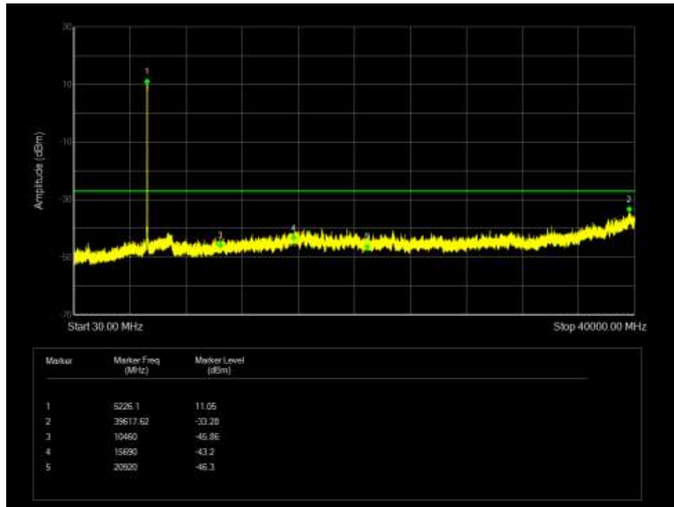
Tx. Spurious NVNT 802.11ac80 5210MHz Ant 4 Emission
