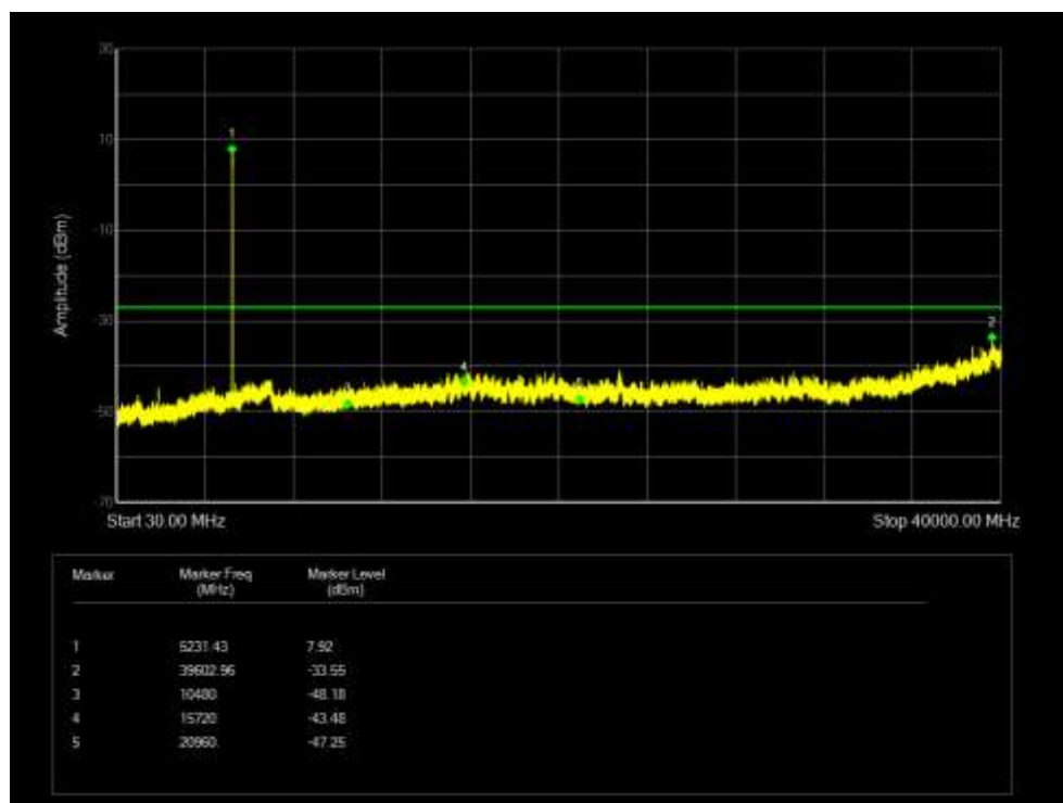
Tx. Spurious NVNT 802.11ax20 5180MHz Ant 7 Emission
