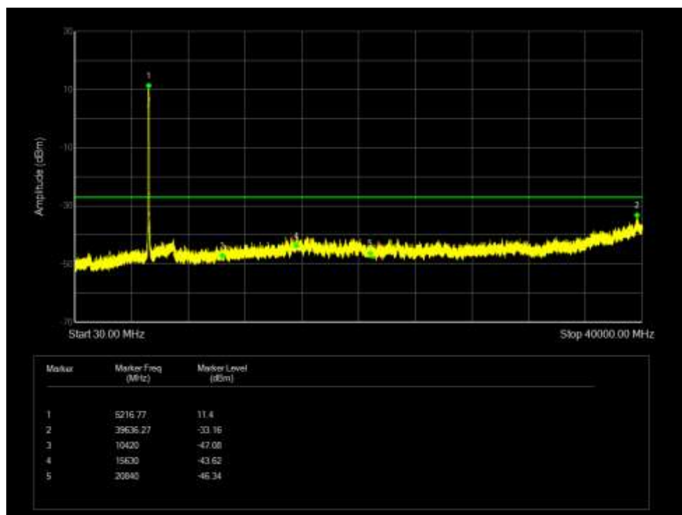
Tx. Spurious NVNT 802.11ax80 5210MHz Ant 7 Emission
