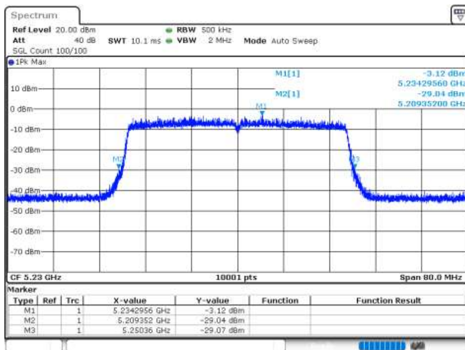
-26 dB BW NVNT 802.11ax40 5230MHz Ant 7
