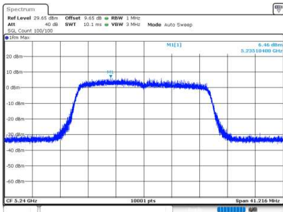
PSD NVNT 802.11ax20 5240MHz Ant 5
