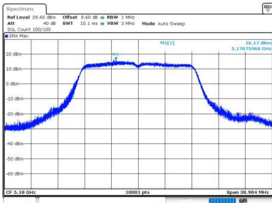
PSD NVNT 802.11a 5180MHz Ant 5
