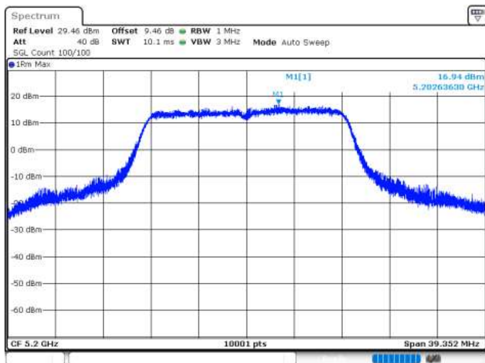
PSD NVNT 802.11a 5200MHz Ant 6
