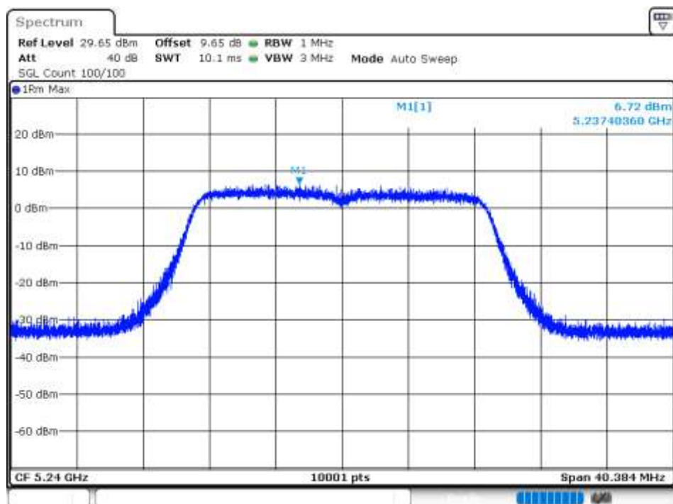
PSD NVNT 802.11n(HT20) 5240MHz Ant 5
