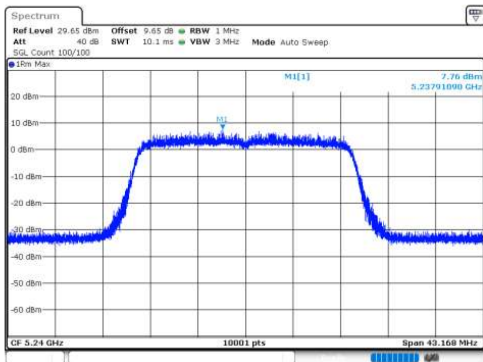
PSD NVNT 802.11ax20 5240MHz Ant 7
