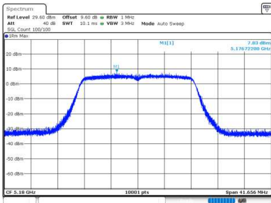
PSD NVNT 802.11ac20 5180MHz Ant 7
