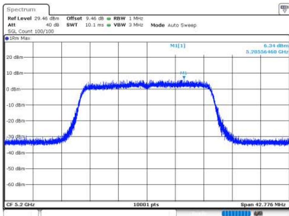
PSD NVNT 802.11ax20 5200MHz Ant 4
