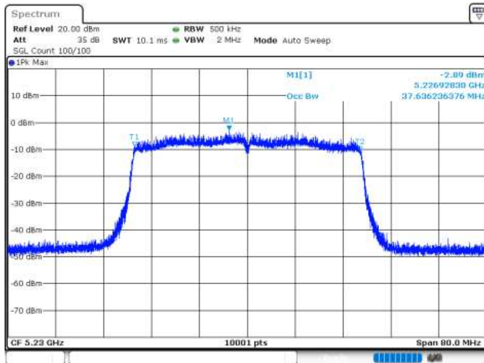
-26 dB BW NVNT 802.11ax40 5230MHz Ant 6
