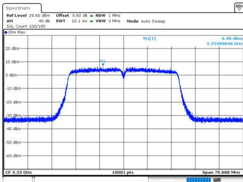
PSD NVNT 802.11ac40 5230MHz Ant 7
