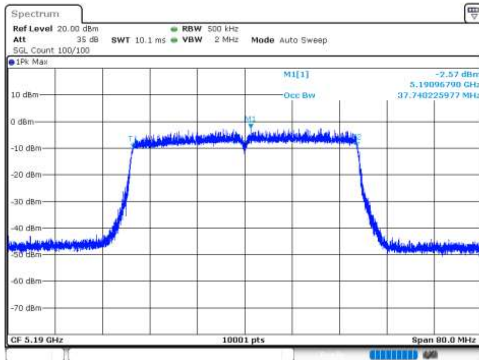
-26 dB BW NVNT 802.11ax40 5190MHz Ant 7
