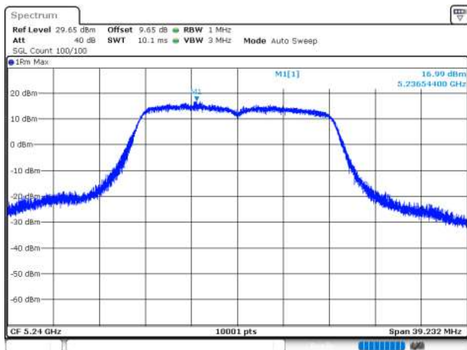
PSD NVNT 802.11a 5240MHz Ant 5
