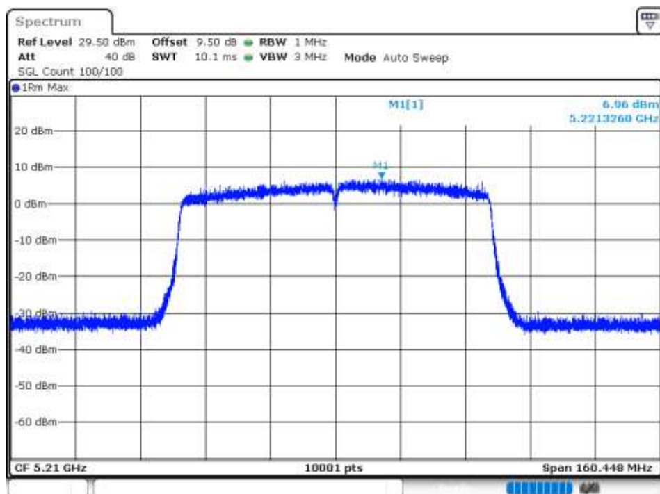
PSD NVNT 802.11ac80 5210MHz Ant 7
