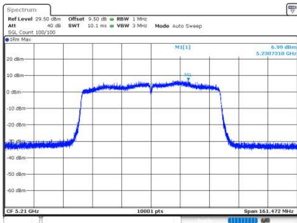
PSD NVNT 802.11ac80 5210MHz Ant 5
