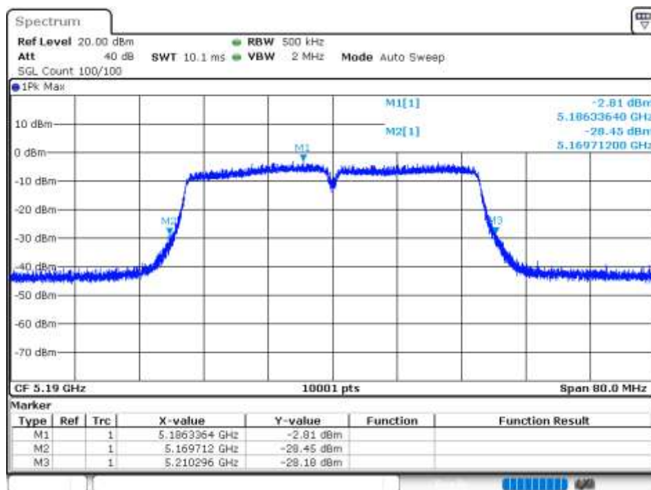
-26 dB BW NVNT 802.11n(HT40) 5190MHz Ant 5
