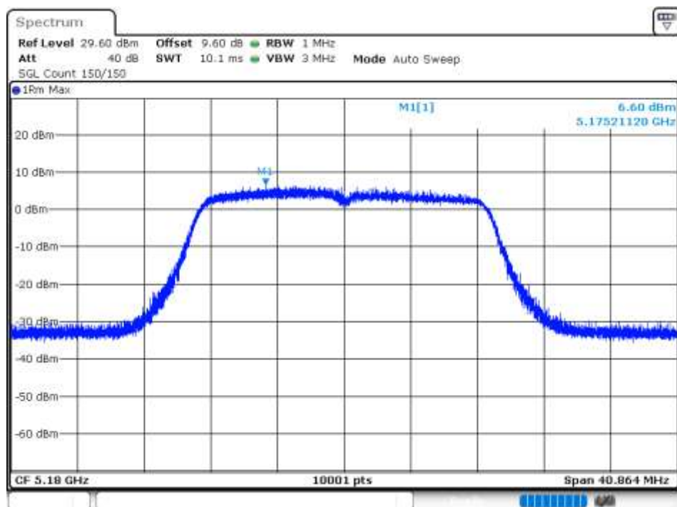
PSD NVNT 802.11n(HT20) 5180MHz Ant 5
