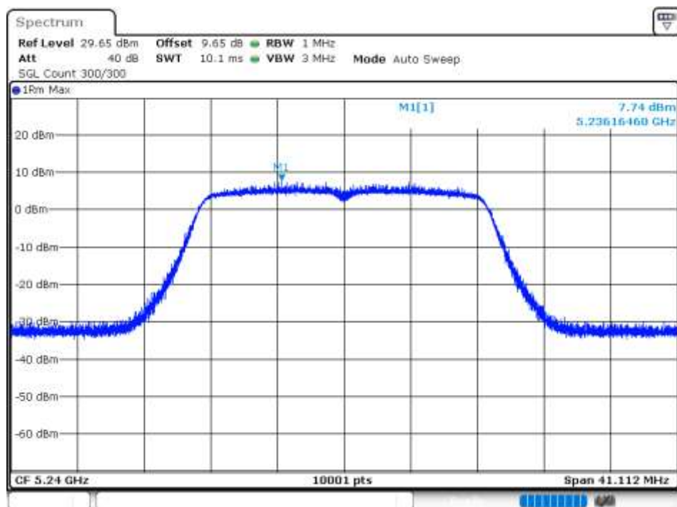
PSD NVNT 802.11n(HT20) 5240MHz Ant 7
