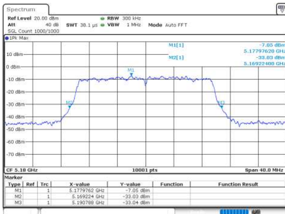
-26 dB BW NVNT 802.11ax20 5180MHz Ant 7
