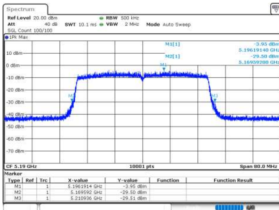
-26 dB BW NVNT 802.11ax40 5190MHz Ant 5
