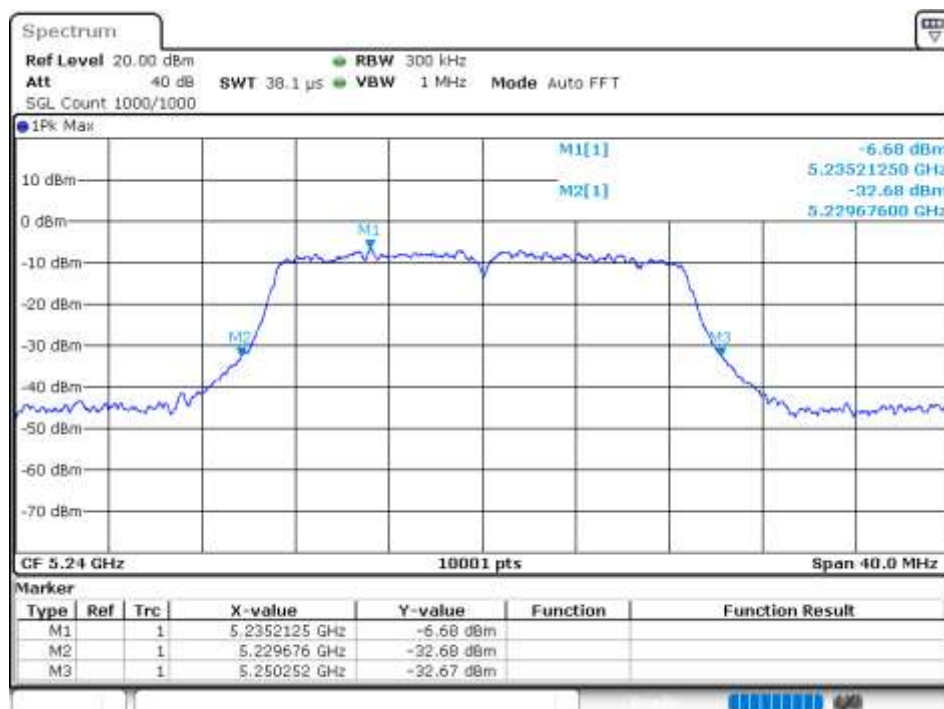
-26 dB BW NVNT 802.11n(HT20) 5240MHz Ant 6
