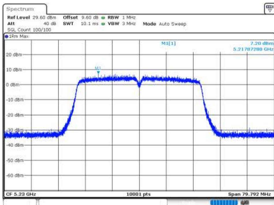
PSD NVNT 802.11n(HT40) 5230MHz Ant 7
