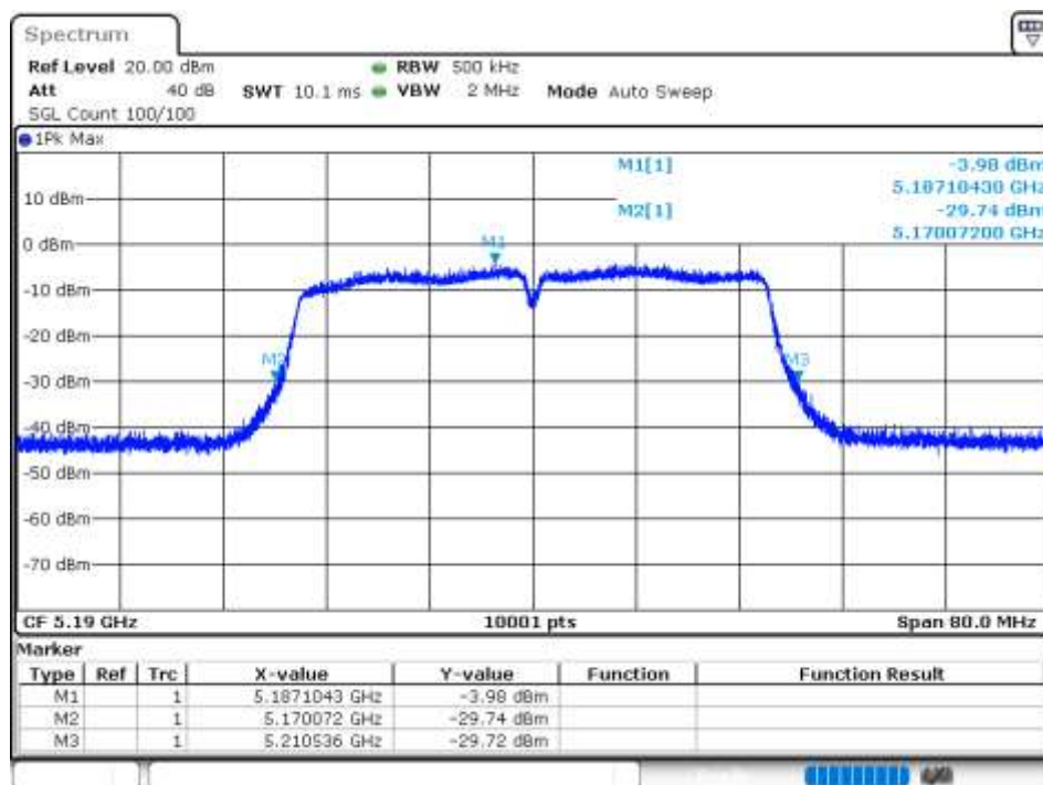
-26 dB BW NVNT 802.11n(HT40) 5190MHz Ant 6
