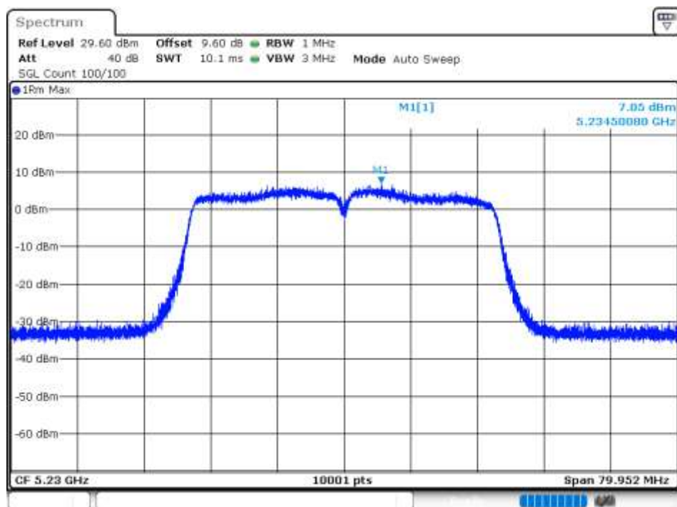
PSD NVNT 802.11ac40 5230MHz Ant 6
