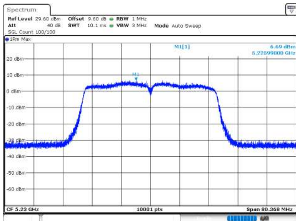
PSD NVNT 802.11n(HT40) 5230MHz Ant 6
