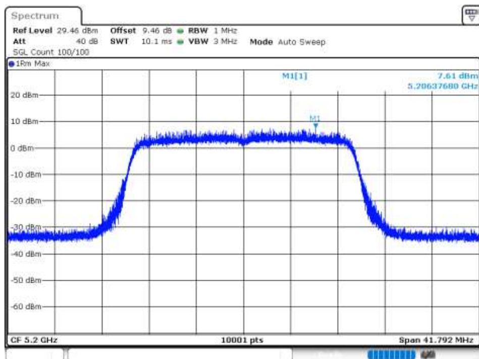
PSD NVNT 802.11ax20 5200MHz Ant 6
