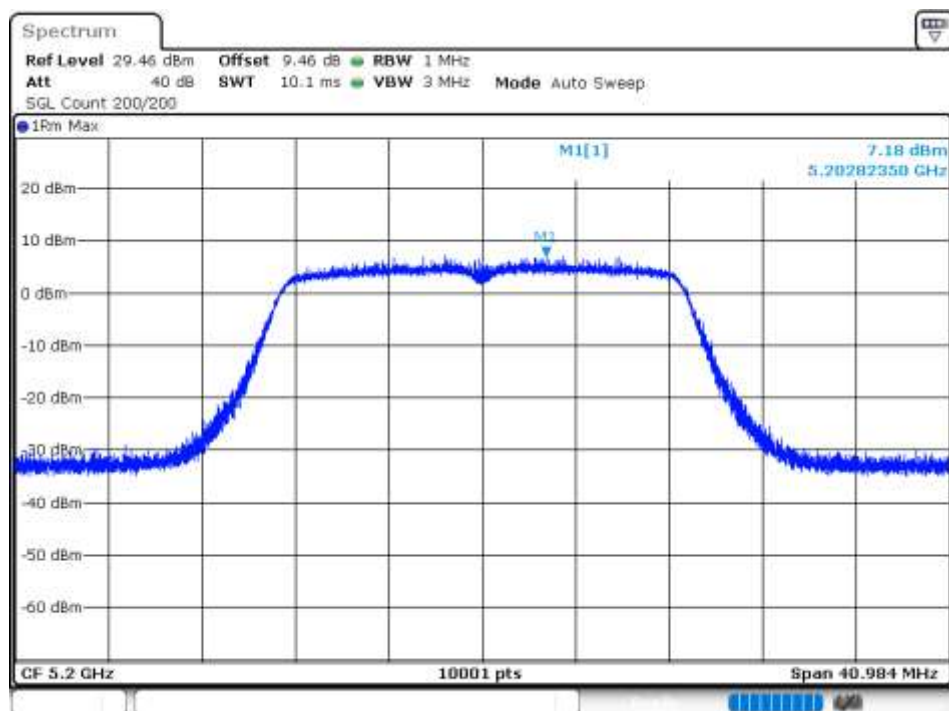
PSD NVNT 802.11n(HT20) 5200MHz Ant 6
