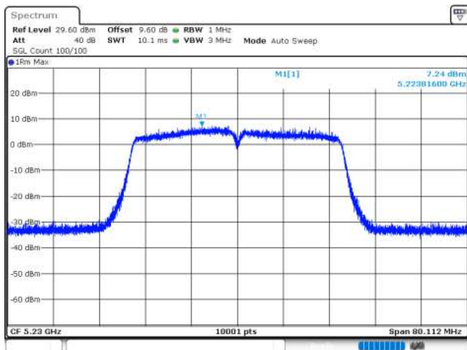
PSD NVNT 802.11n(HT40) 5230MHz Ant 5
