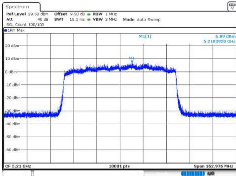
PSD NVNT 802.11ax80 5210MHz Ant 7
