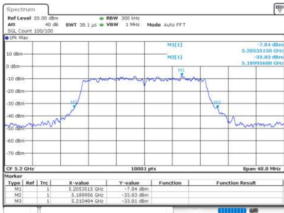
-26 dB BW NVNT 802.11n(HT20) 5200MHz Ant 5
