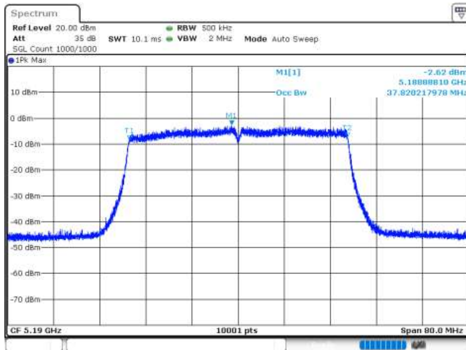
-26 dB BW NVNT 802.11ax40 5190MHz Ant 4
