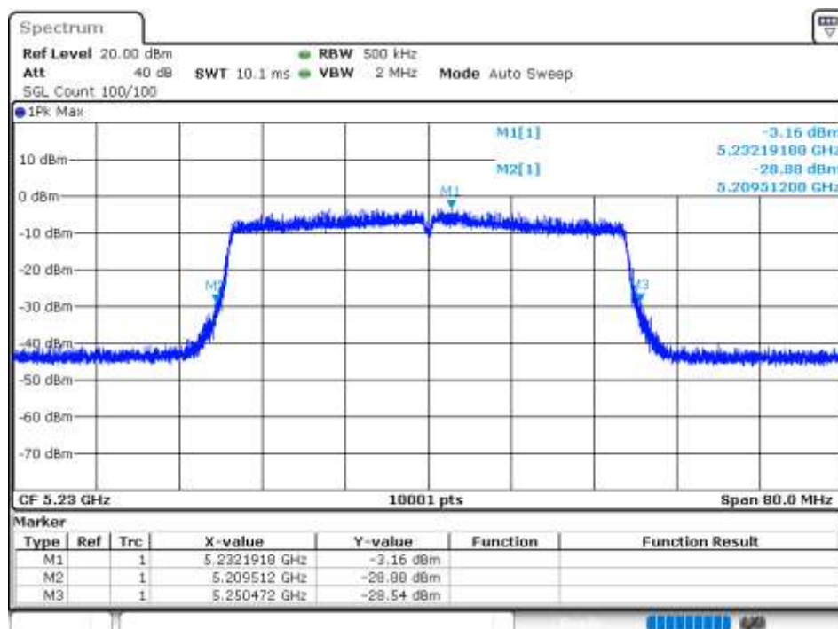
-26 dB BW NVNT 802.11ax40 5230MHz Ant 5
