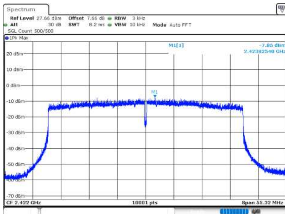
PSD NVNT 802.11ax40 2422MHz Ant 0
