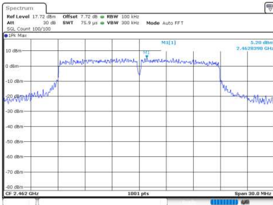
Band Edge NVNT 802.11n(HT20) 2462MHz Ant 0 Ref
