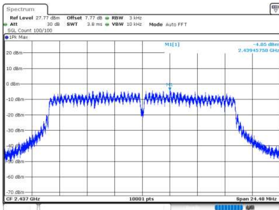
PSD NVNT 802.11g 2437MHz Ant 3
