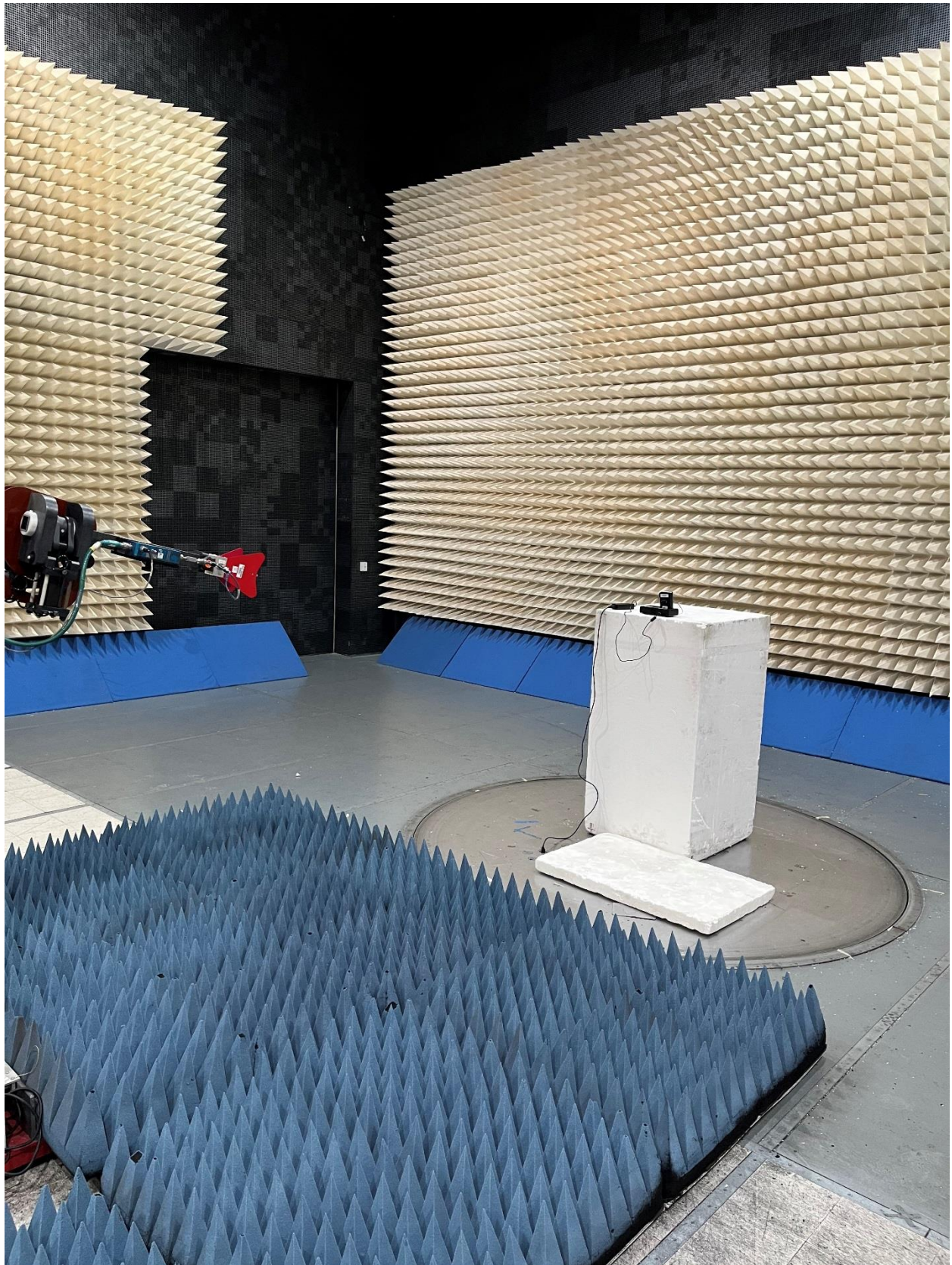
Radiated Emissions Above 1GHz
