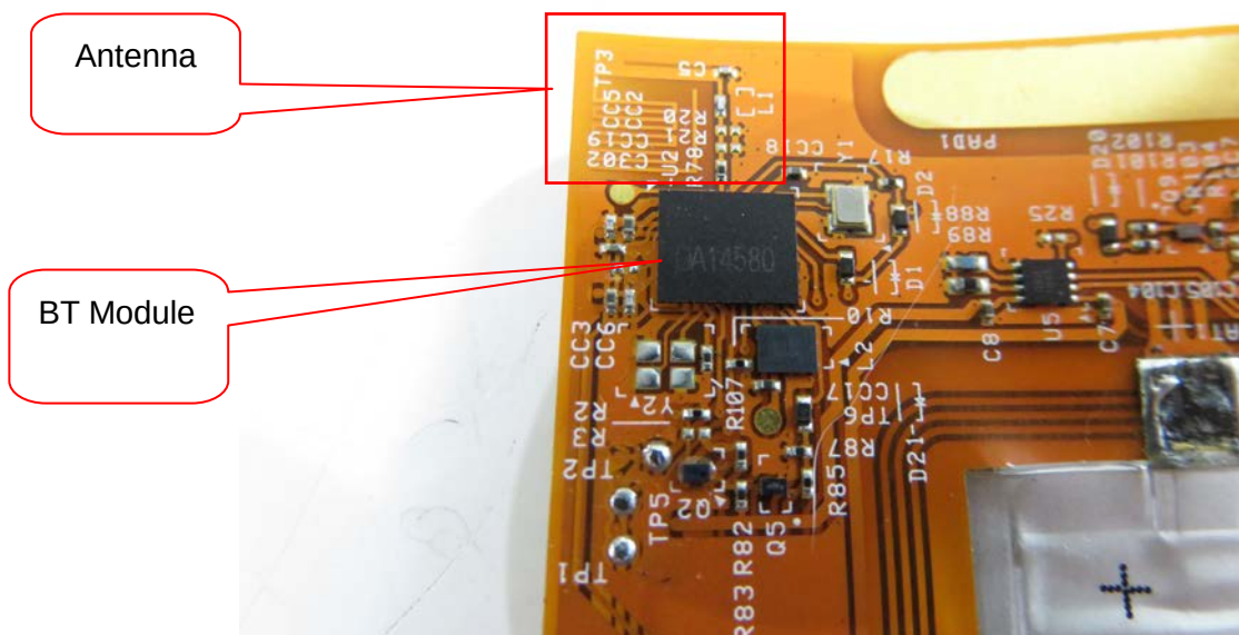
Close Up View of the BT module & Antenna
