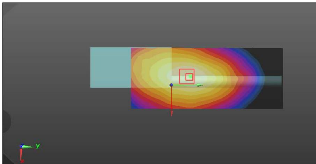
Figure 31: PMR_FM12.5KHz_Face held_25mm
