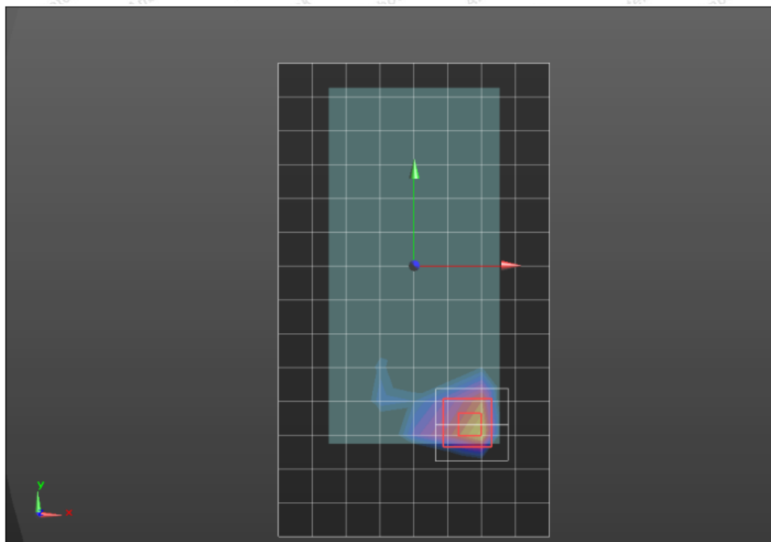
Figure 16: GSM850_Front side_0mm
