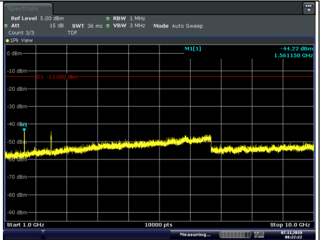
1GHz~10GHz
