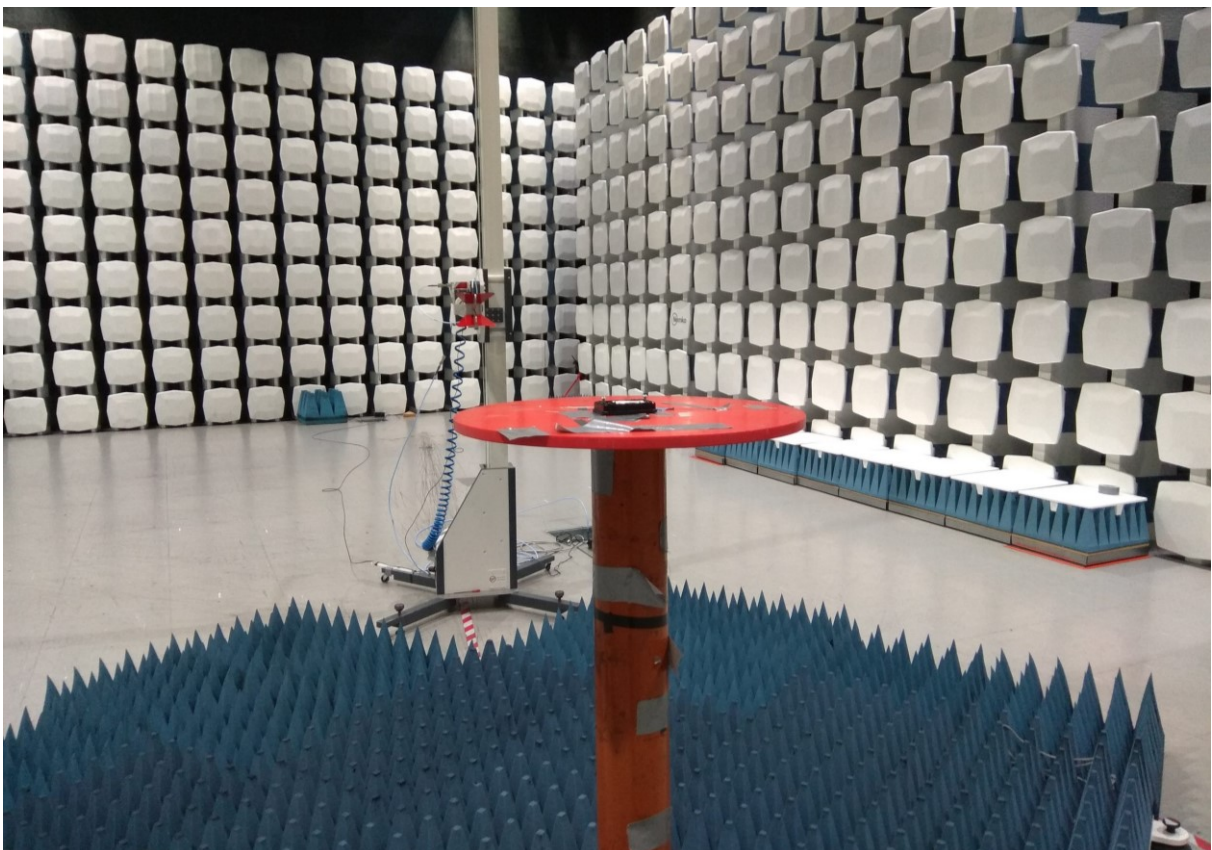
Radiated Emissions, 1 - 18 GHz
