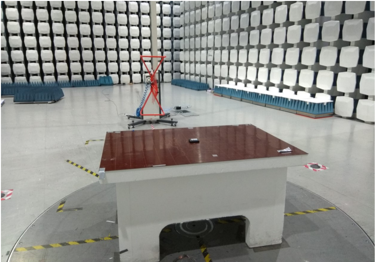
Radiated Emission, Below 1 GHz
