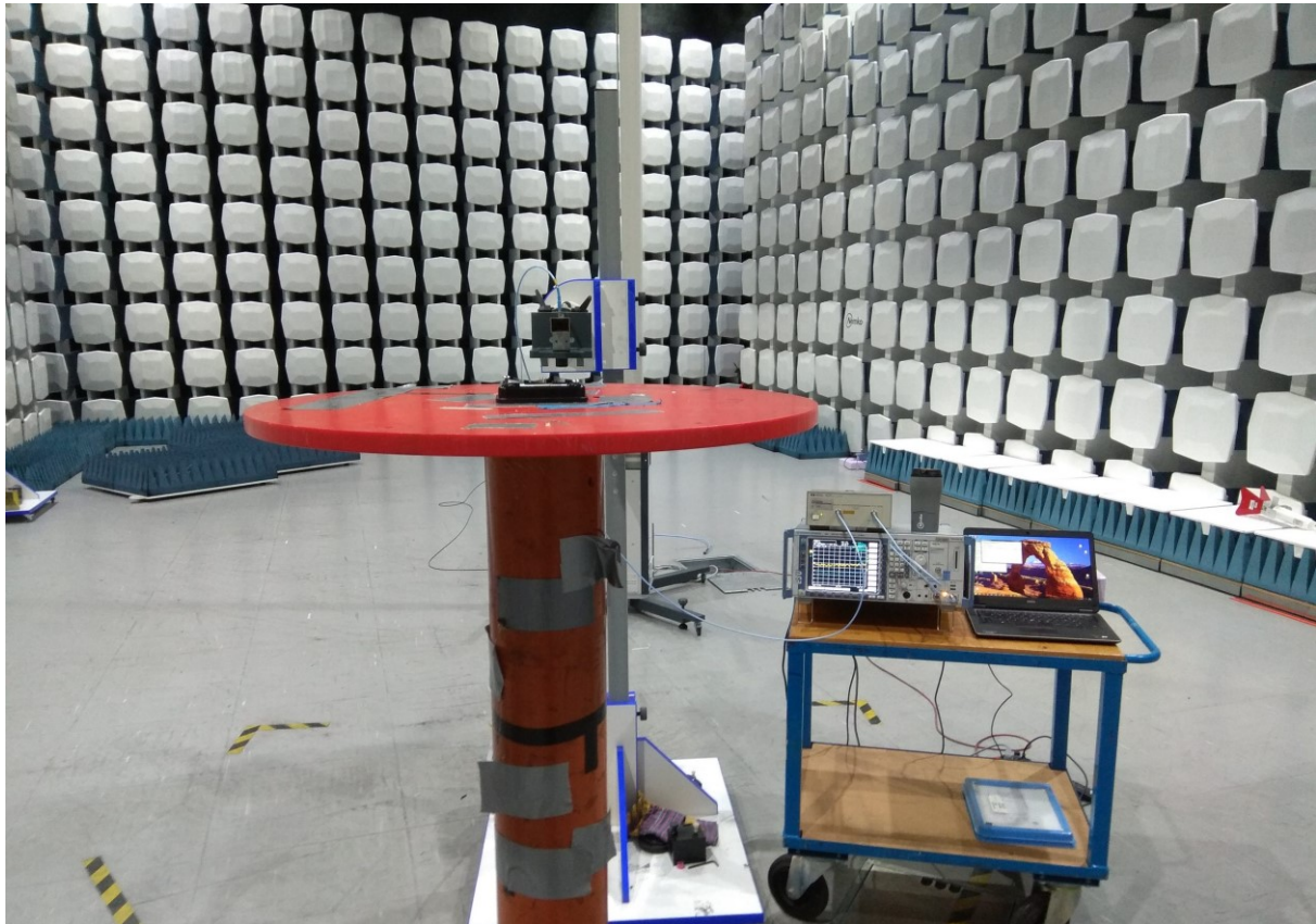
Radiated Emissions, above 18 GHz
