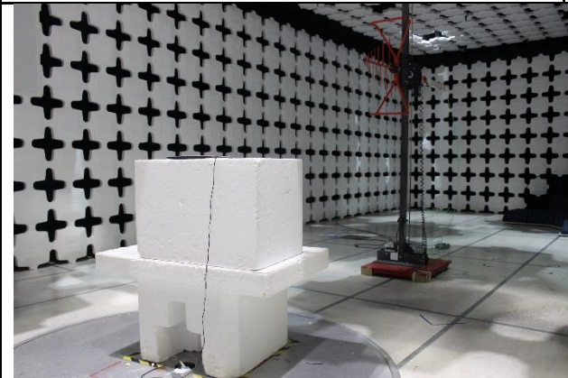
Radiated Emission Below 1G – Front View
