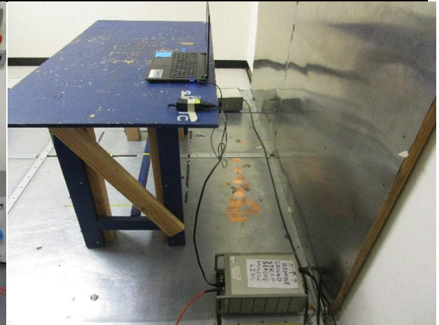
Conducted Emission – Side View
