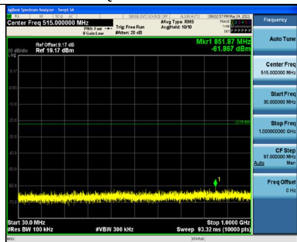
\pi/4 -DQPSK on Channel 78
