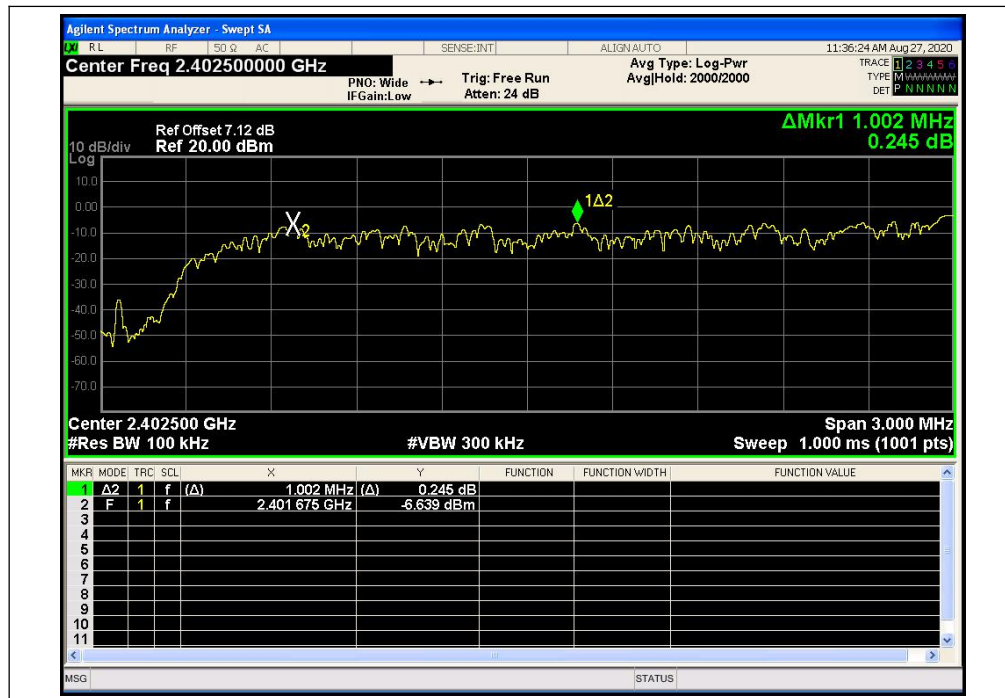
(8-DPSK, Channel 0 and 1, 2402MHz)
