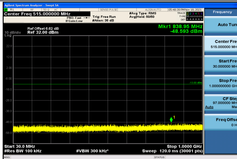
Band2-15MHz-QPSK-18900-1RB#0-30~1000MHz
