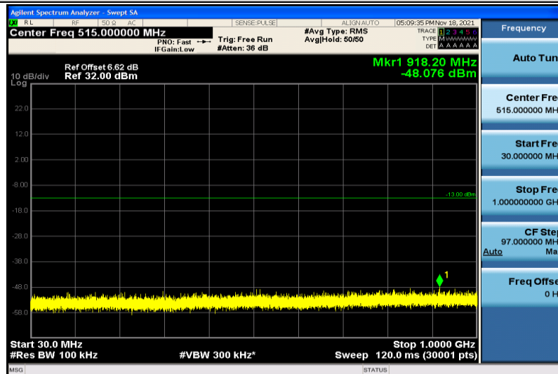
Band2-5MHz-QPSK-18900-1RB#0-30~1000MHz
