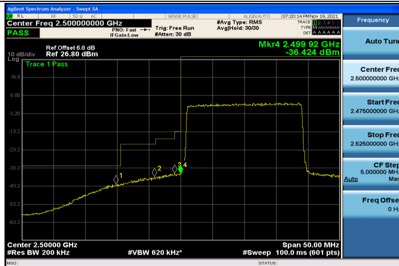
Band7-20MHz-16QAM-20850-100RB#0
