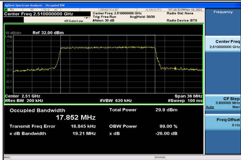
Band7-20MHz-QPSK-20850-100RB#0-17.852
