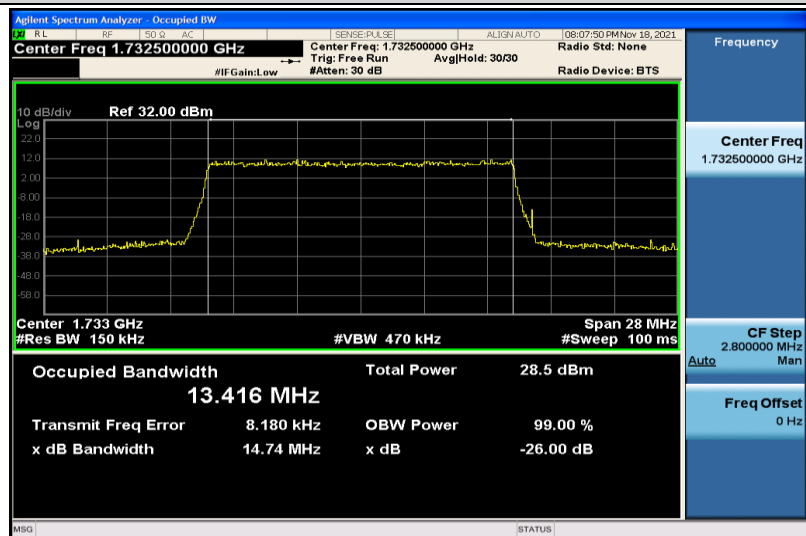
Band4-15MHz-16QAM-20175-75RB#0-13.416
