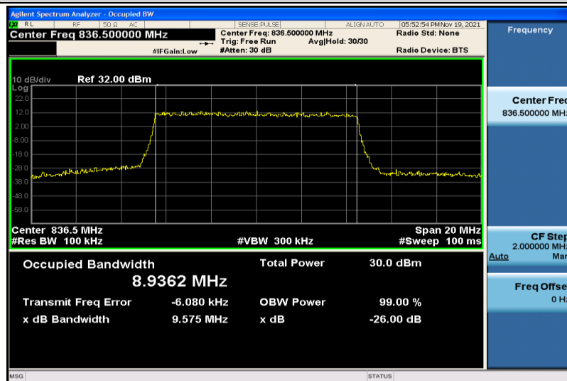
Band5-10MHz-QPSK-20525-50RB#0-8.9362
