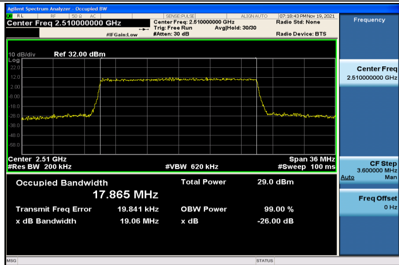
Band7-20MHz-16QAM-20850-100RB#0-17.865
