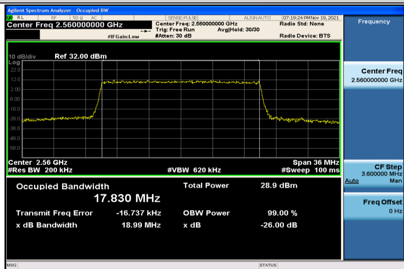
Band7-20MHz-16QAM-21350-100RB#0-17.830
