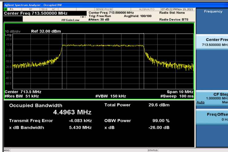
Band17-5MHz-QPSK-23825-25RB#0-4.4963
