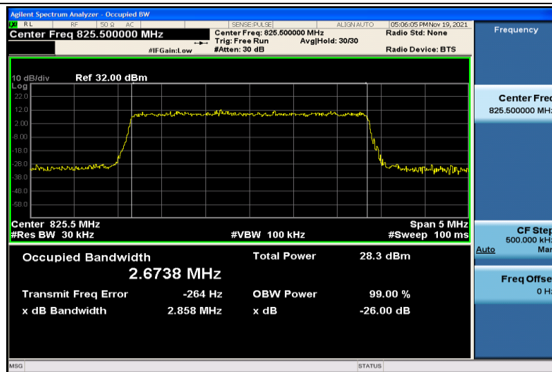
Band5-3MHz-16QAM-20415-15RB#0-2.6738
