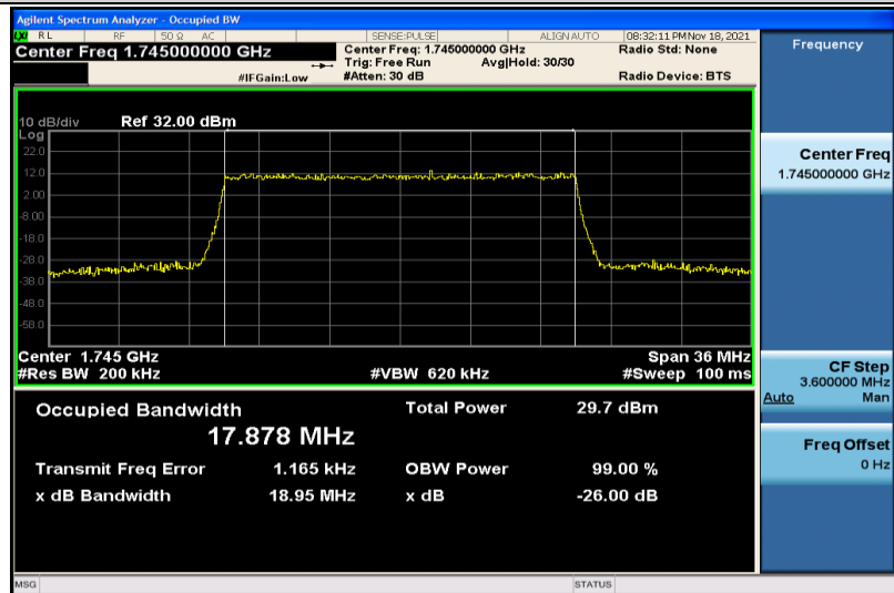
Band4-20MHz-QPSK-20300-100RB#0-17.878
