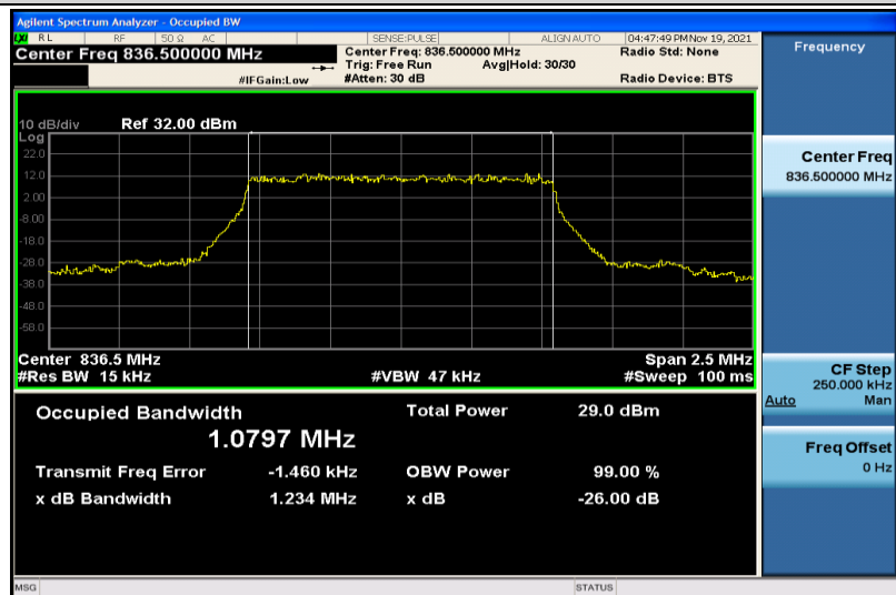
Band5-1.4MHz-QPSK-20525-6RB#0-1.0797
