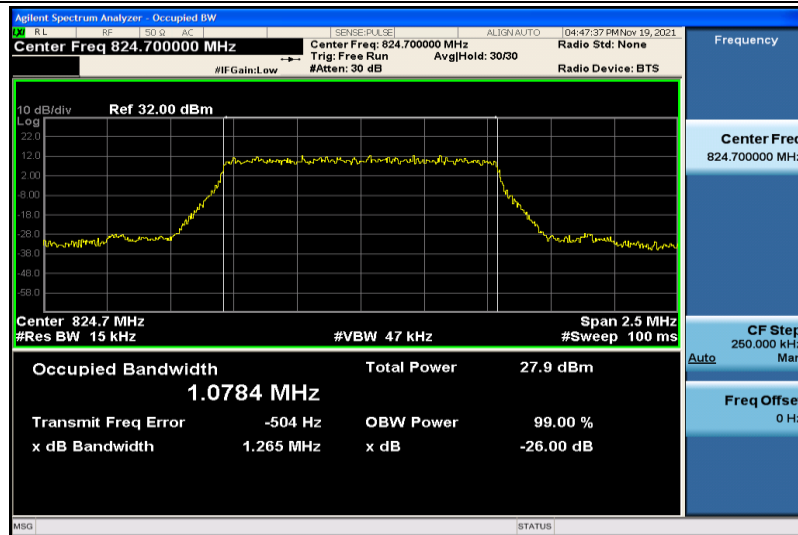
Band5-1.4MHz-16QAM-20407-6RB#0-1.0784
