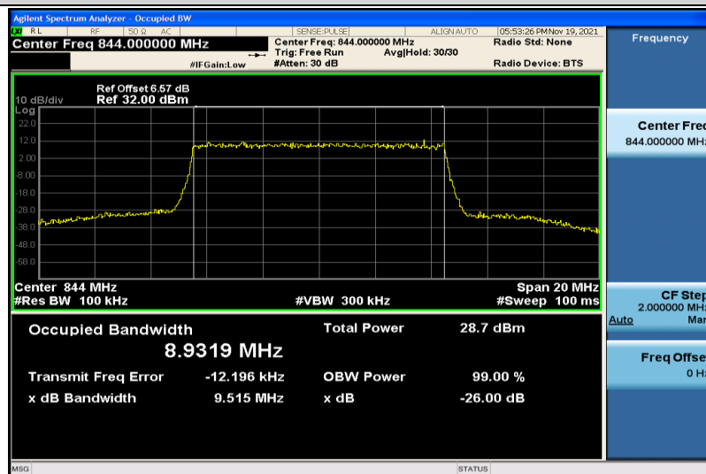
Band5-10MHz-16QAM-20600-50RB#0-8.9319
