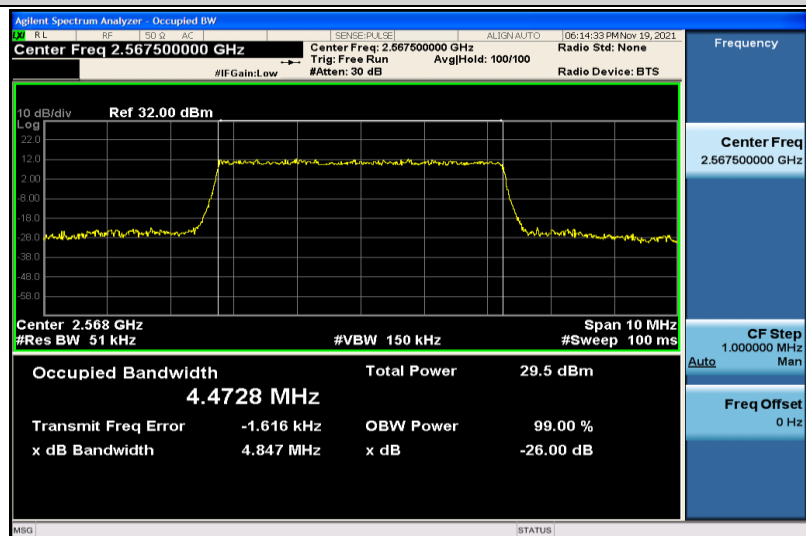
Band7-5MHz-QPSK-21425-25RB#0-4.4728
