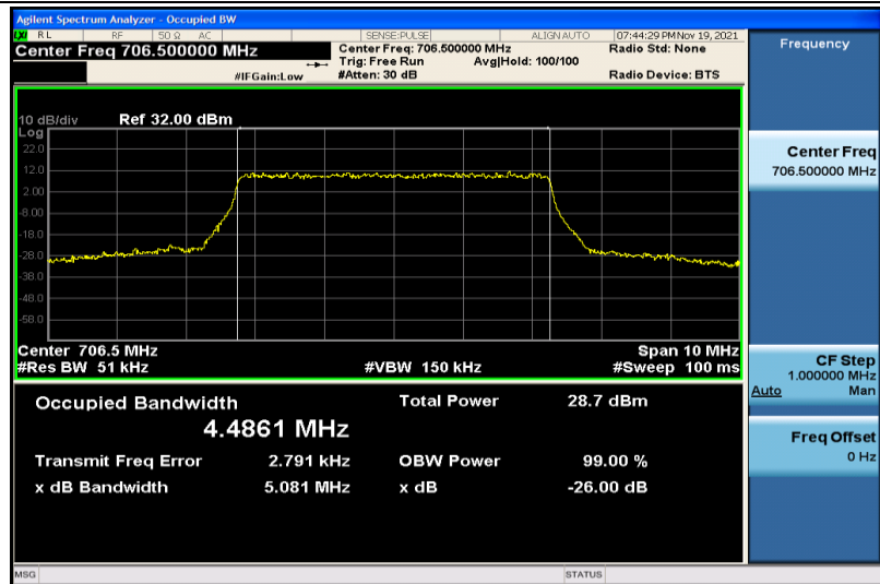
Band17-5MHz-16QAM-23755-25RB#0-4.4861
