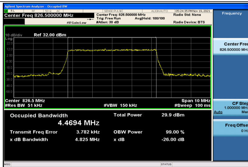
Band5-5MHz-QPSK-20425-25RB#0-4.4694
