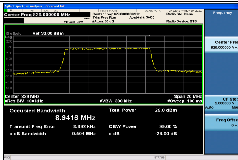
Band5-10MHz-16QAM-20450-50RB#0-8.9416
