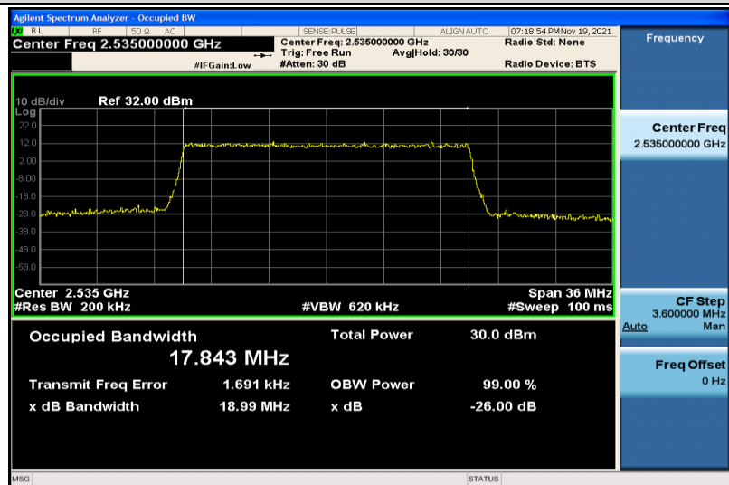
Band7-20MHz-QPSK-21100-100RB#0-17.843
