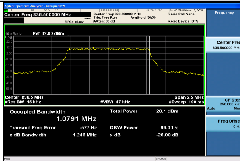
Band5-1.4MHz-16QAM-20525-6RB#0-1.0791
