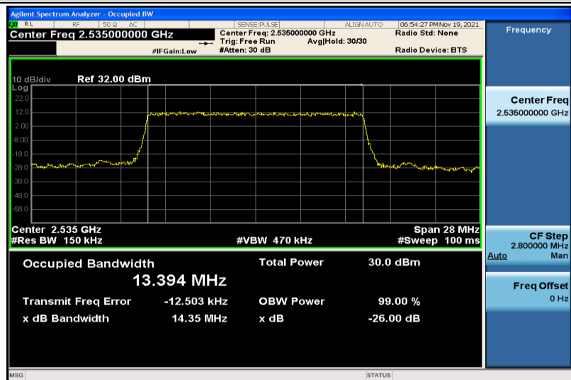
Band7-15MHz-QPSK-21100-75RB#0-13.394
