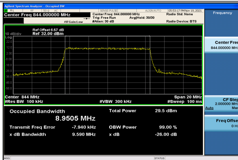
Band5-10MHz-QPSK-20600-50RB#0-8.9505
