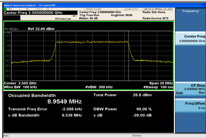
Band7-10MHz-16QAM-20800-50RB#0-8.9549
