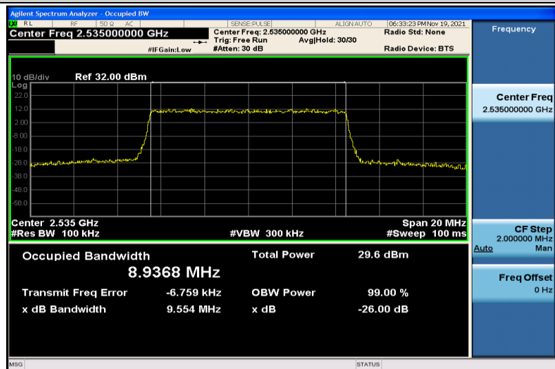
Band7-10MHz-QPSK-21100-50RB#0-8.9368
