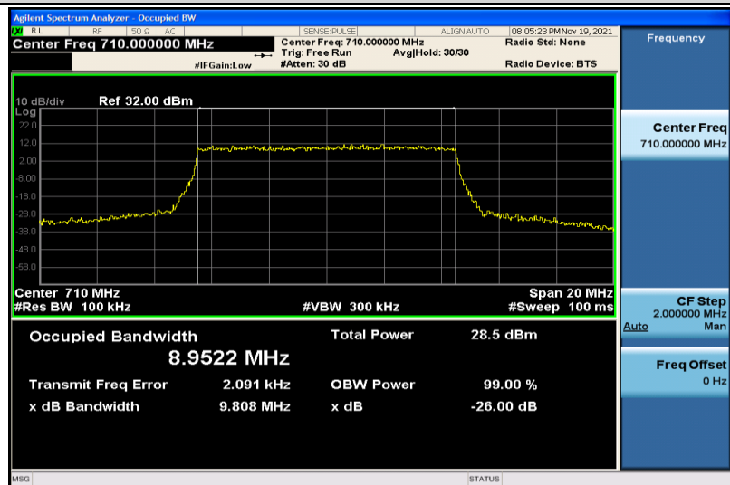
Band17-10MHz-16QAM-23790-50RB#0-8.9522
