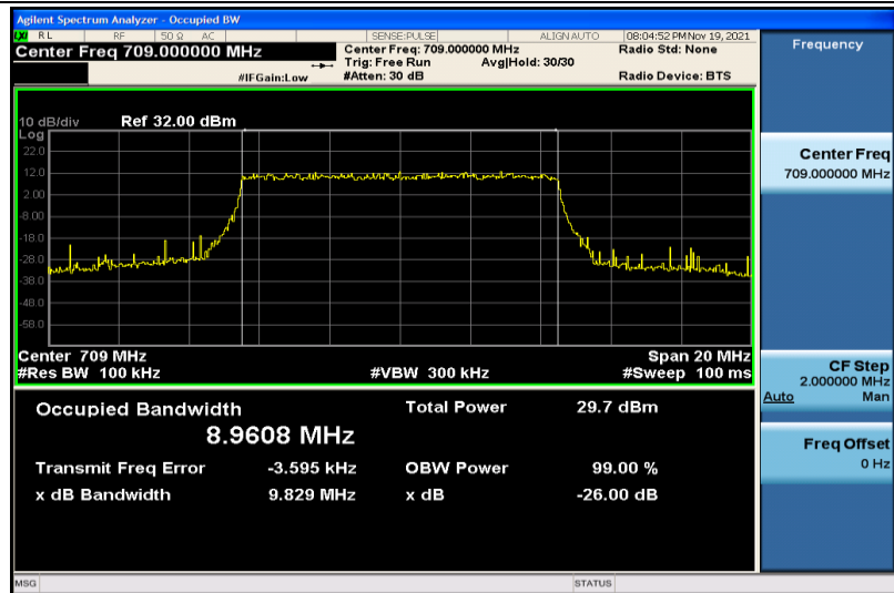
Band17-10MHz-QPSK-23780-50RB#0-8.9608
