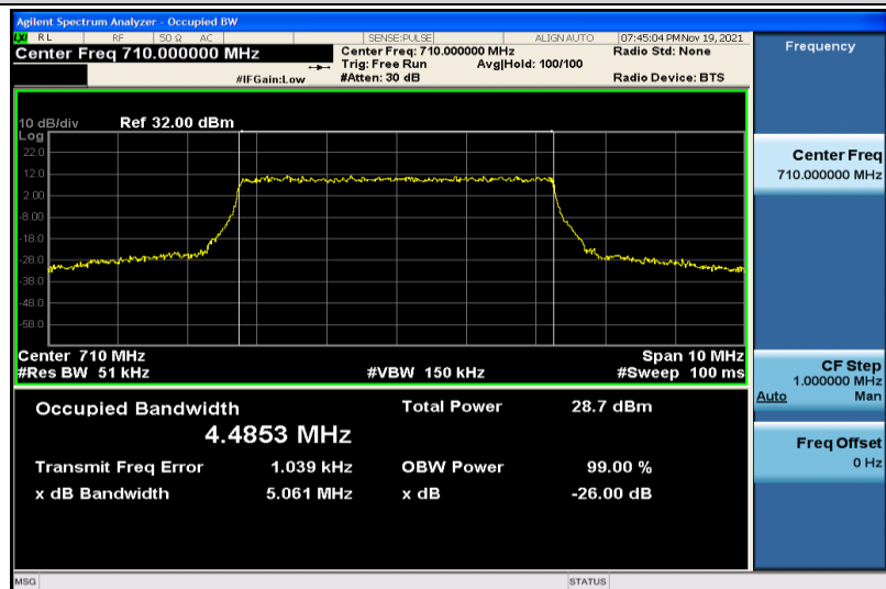
Band17-5MHz-16QAM-23790-25RB#0-4.4853
