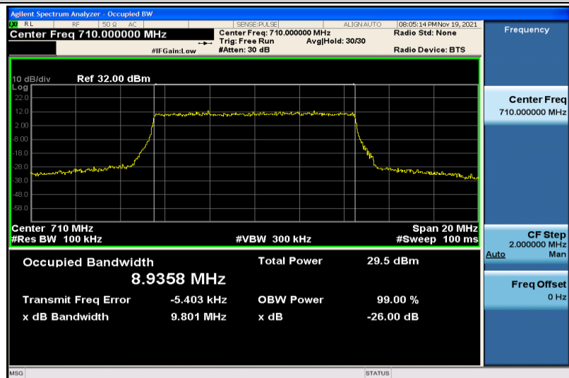
Band17-10MHz-QPSK-23790-50RB#0-8.9358
