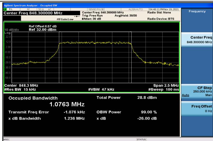
Band5-1.4MHz-QPSK-20643-6RB#0-1.0763
