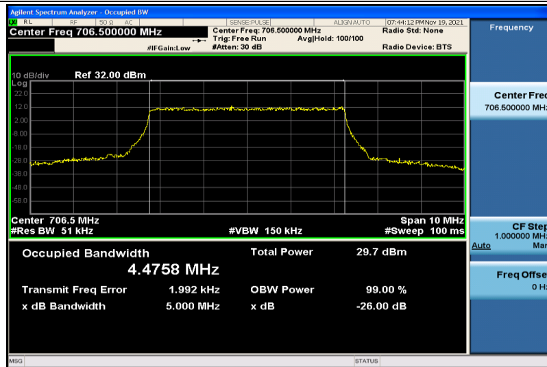
Band17-5MHz-QPSK-23755-25RB#0-4.4758
