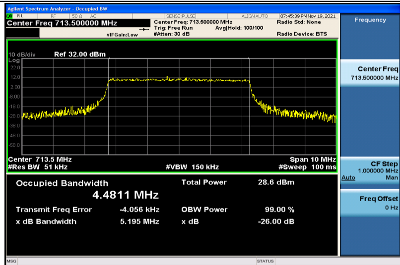
Band17-5MHz-16QAM-23825-25RB#0-4.4811
