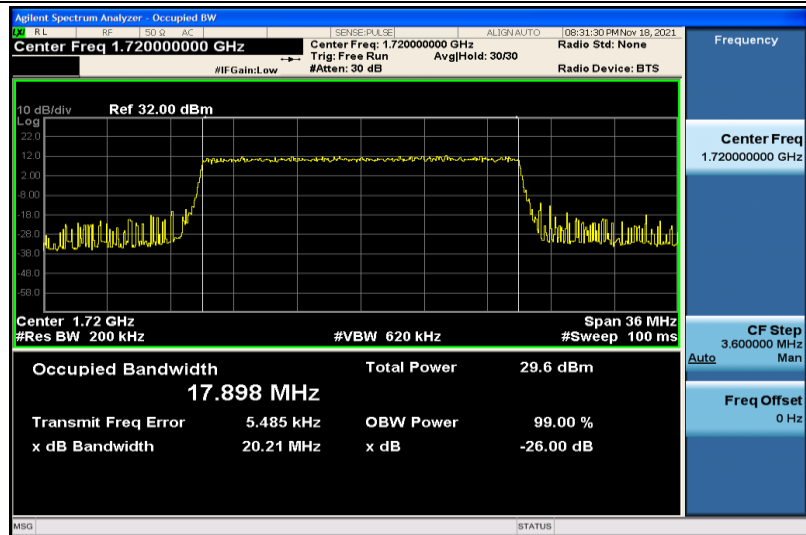
Band4-20MHz-QPSK-20050-100RB#0-17.898
