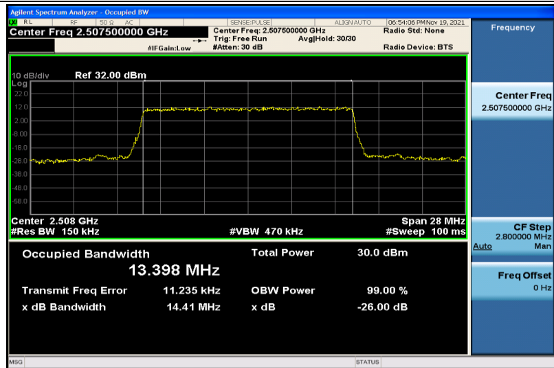
Band7-15MHz-QPSK-20825-75RB#0-13.398
