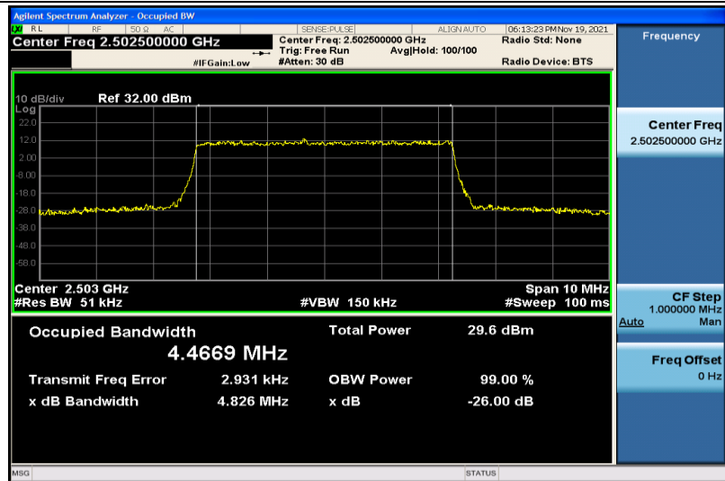
Band7-5MHz-QPSK-20775-25RB#0-4.4669
