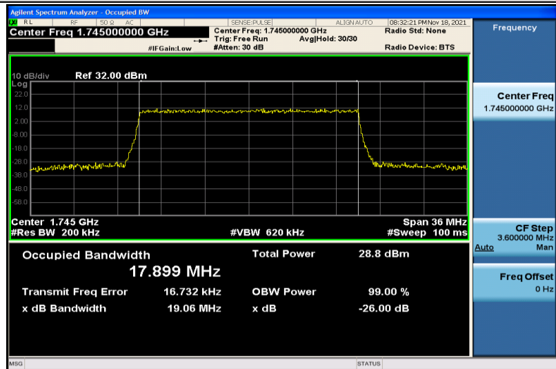
Band4-20MHz-16QAM-20300-100RB#0-17.899
