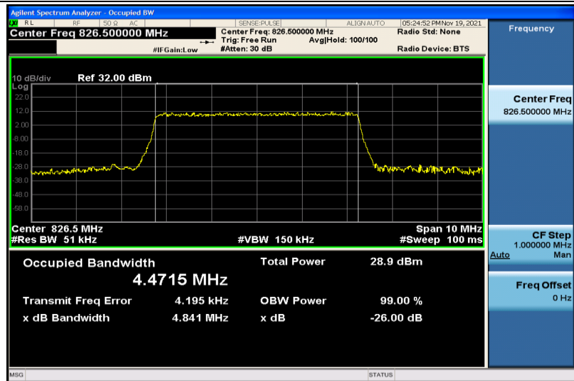
Band5-5MHz-16QAM-20425-25RB#0-4.4715
