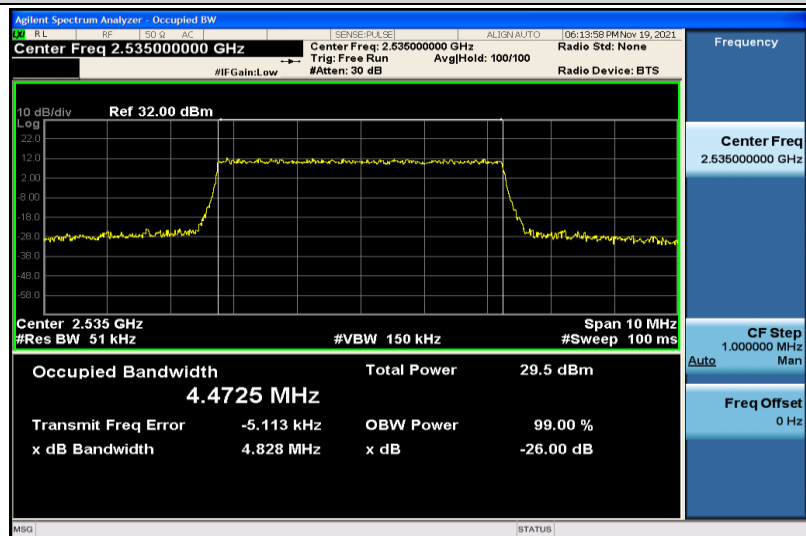
Band7-5MHz-QPSK-21100-25RB#0-4.4725
