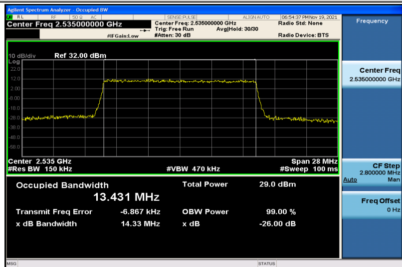
Band7-15MHz-16QAM-21100-75RB#0-13.431
