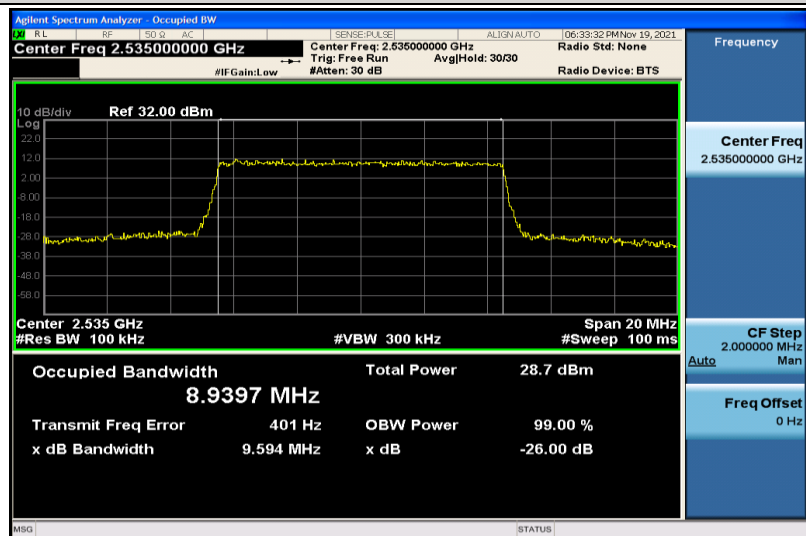
Band7-10MHz-16QAM-21100-50RB#0-8.9397
