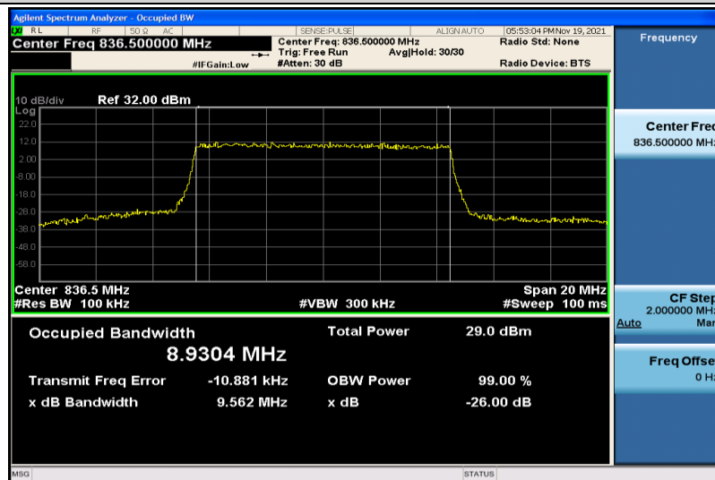
Band5-10MHz-16QAM-20525-50RB#0-8.9304
