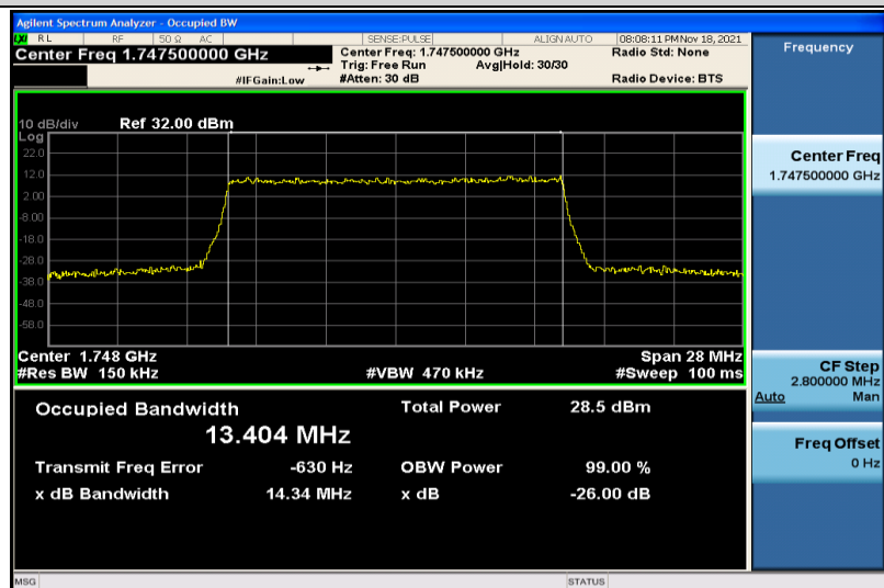
Band4-15MHz-16QAM-20325-75RB#0-13.404
