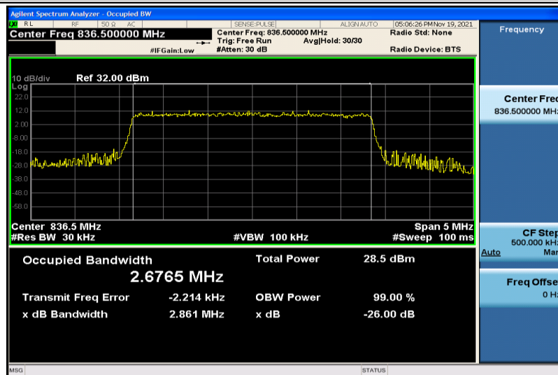
Band5-3MHz-16QAM-20525-15RB#0-2.6765
