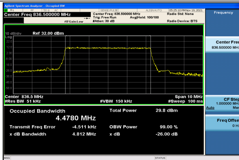
Band5-5MHz-QPSK-20525-25RB#0-4.4780
