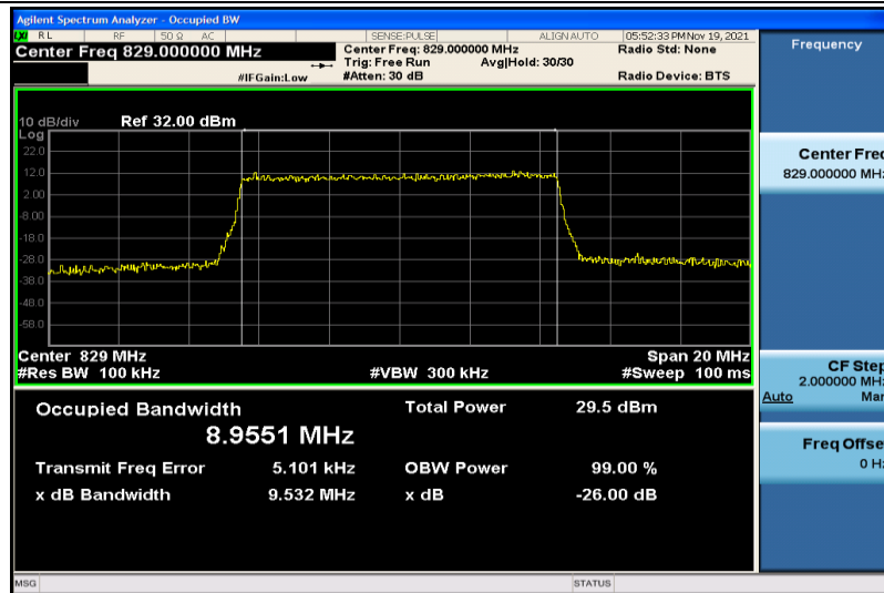
Band5-10MHz-QPSK-20450-50RB#0-8.9551
