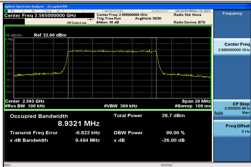
Band7-10MHz-16QAM-21400-50RB#0-8.9321
