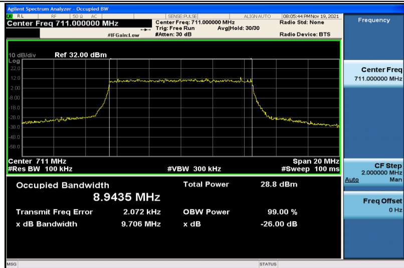
Band17-10MHz-16QAM-23800-50RB#0-8.9435
