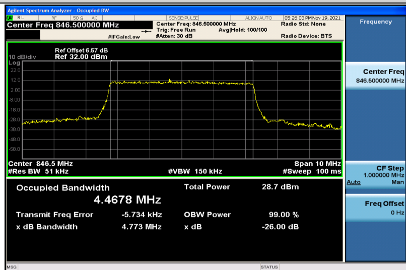
Band5-5MHz-16QAM-20625-25RB#0-4.4678
