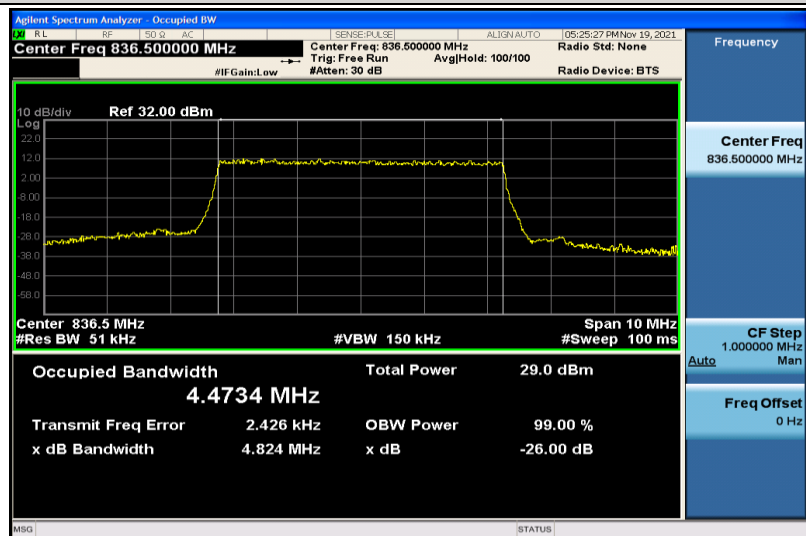
Band5-5MHz-16QAM-20525-25RB#0-4.4734
