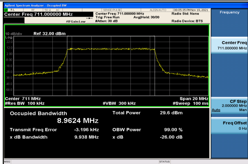
Band17-10MHz-QPSK-23800-50RB#0-8.9624
