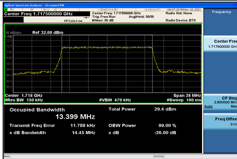
Band4-15MHz-QPSK-20025-75RB#0-13.399
