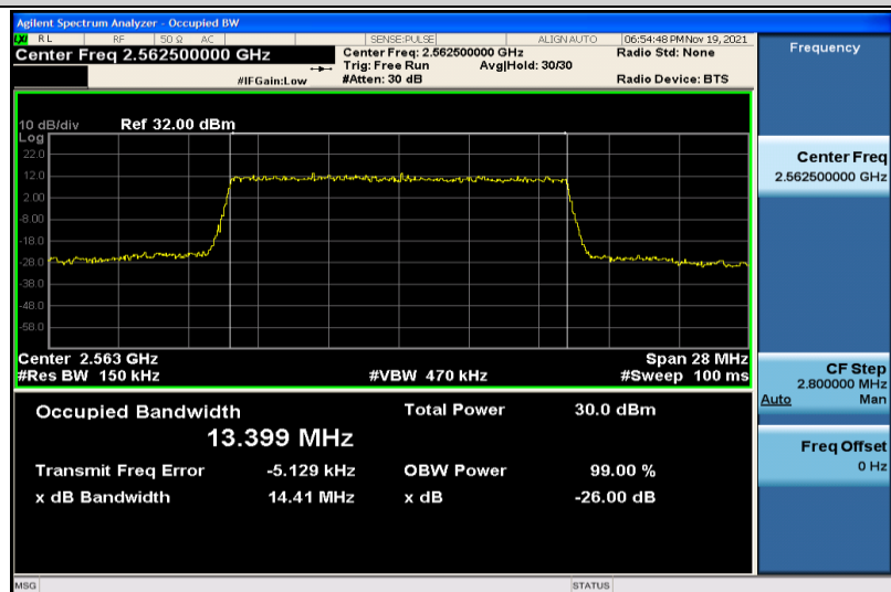
Band7-15MHz-QPSK-21375-75RB#0-13.399
