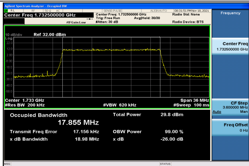
Band4-20MHz-QPSK-20175-100RB#0-17.855
