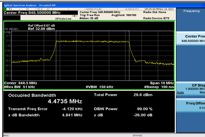
Band5-5MHz-QPSK-20625-25RB#0-4.4735
