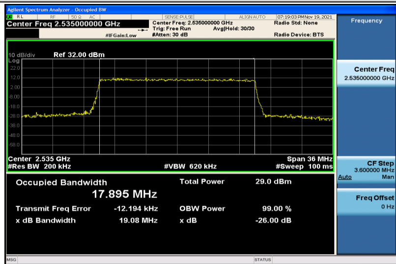
Band7-20MHz-16QAM-21100-100RB#0-17.895
