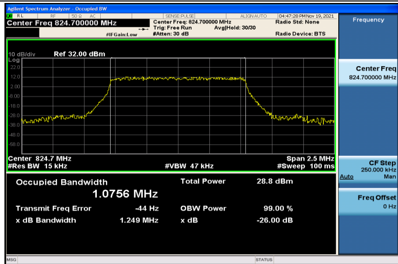
Band5-1.4MHz-QPSK-20407-6RB#0-1.0756
