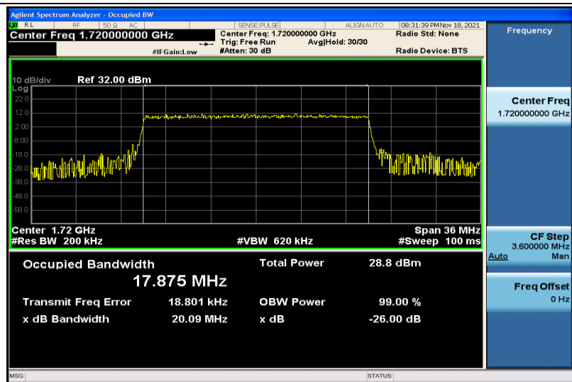
Band4-20MHz-16QAM-20050-100RB#0-17.875
