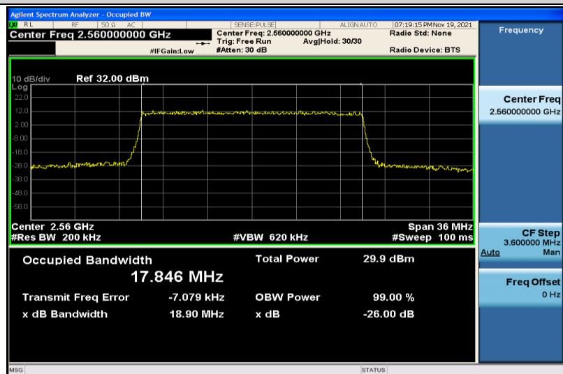
Band7-20MHz-QPSK-21350-100RB#0-17.846
