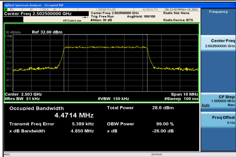
Band7-5MHz-16QAM-20775-25RB#0-4.4714
