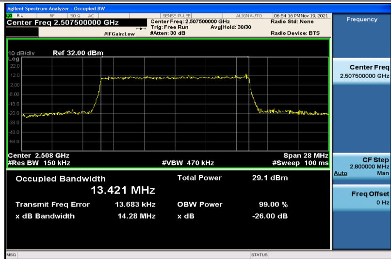
Band7-15MHz-16QAM-20825-75RB#0-13.421
