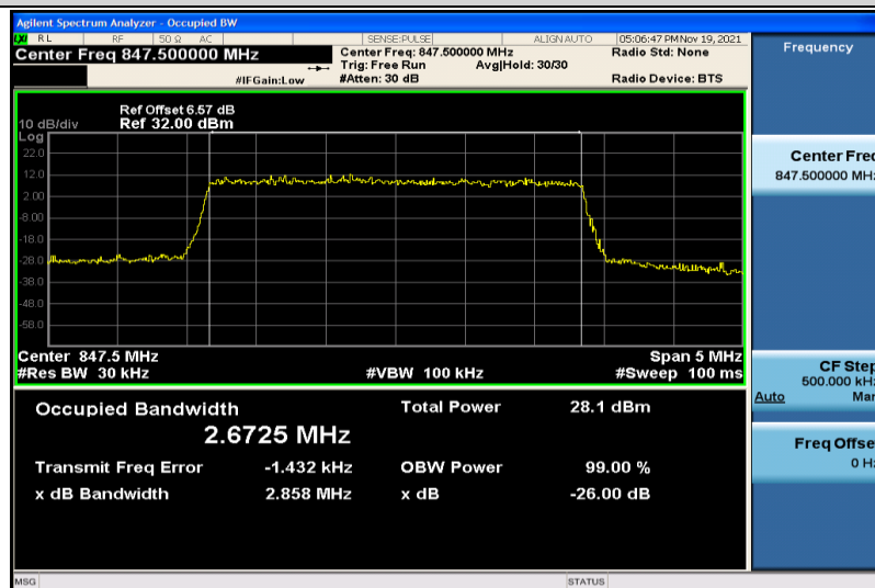
Band5-3MHz-16QAM-20635-15RB#0-2.6725
