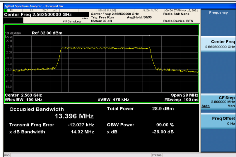
Band7-15MHz-16QAM-21375-75RB#0-13.396
