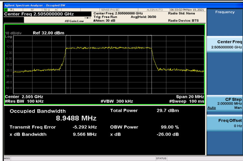
Band7-10MHz-QPSK-20800-50RB#0-8.9488
