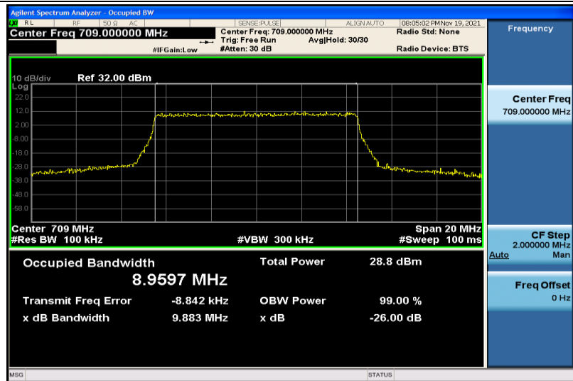
Band17-10MHz-16QAM-23780-50RB#0-8.9597
