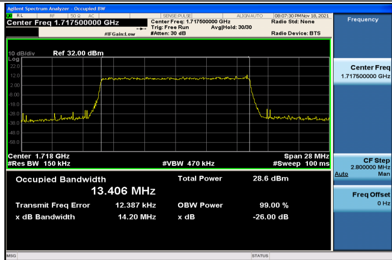
Band4-15MHz-16QAM-20025-75RB#0-13.406
