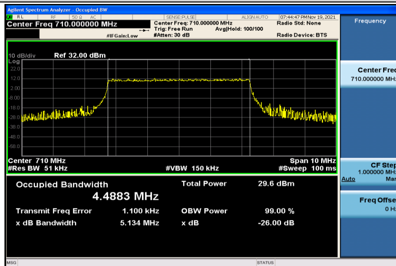
Band17-5MHz-QPSK-23790-25RB#0-4.4883
