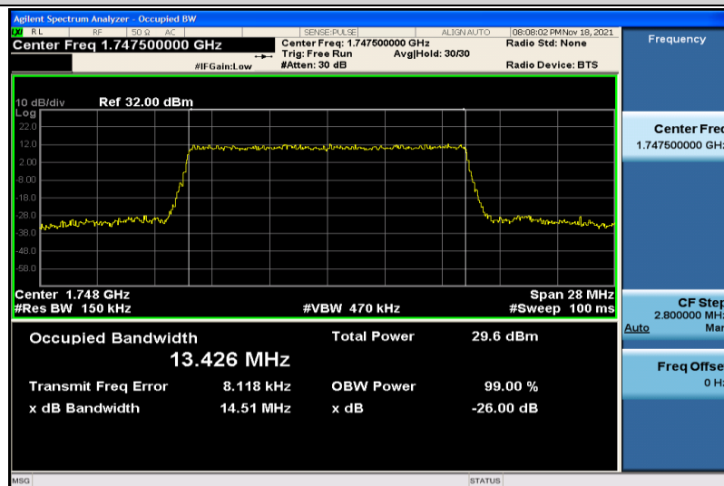
Band4-15MHz-QPSK-20325-75RB#0-13.426
