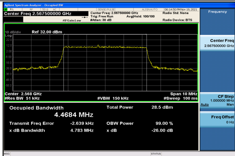
Band7-5MHz-16QAM-21425-25RB#0-4.4684
