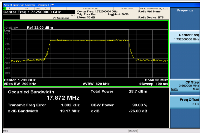
Band4-20MHz-16QAM-20175-100RB#0-17.872
