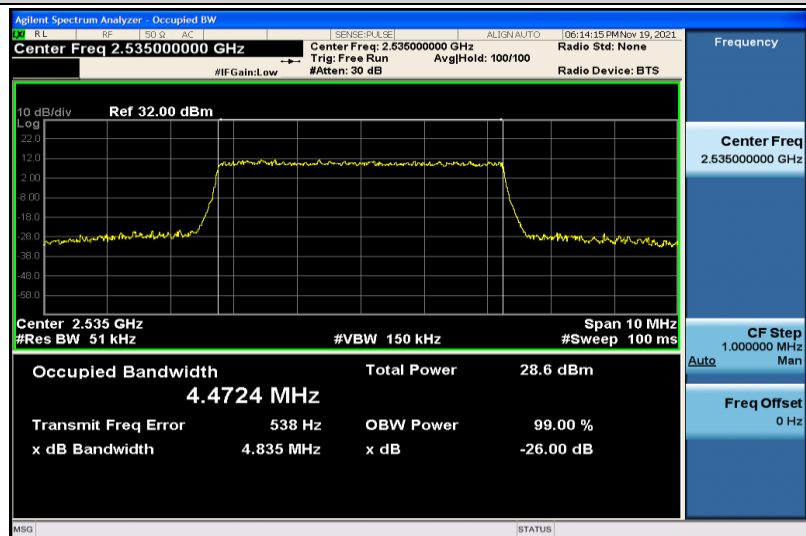
Band7-5MHz-16QAM-21100-25RB#0-4.4724
