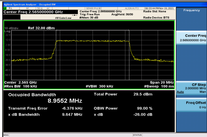
Band7-10MHz-QPSK-21400-50RB#0-8.9552
