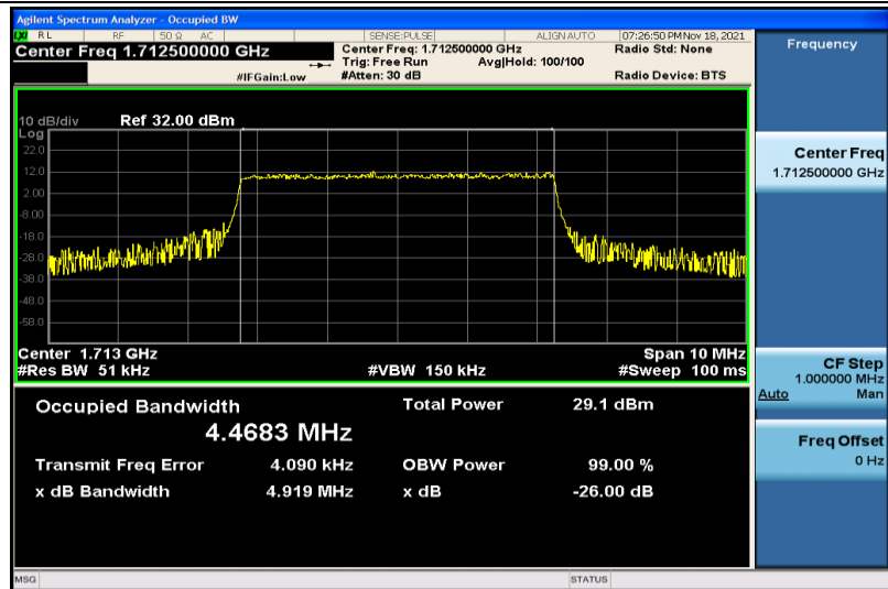
Band4-5MHz-QPSK-19975-25RB#0-4.4683
