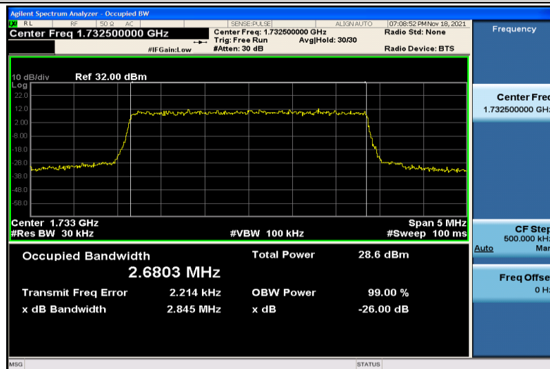
Band4-3MHz-QPSK-20175-15RB#0-2.6803
