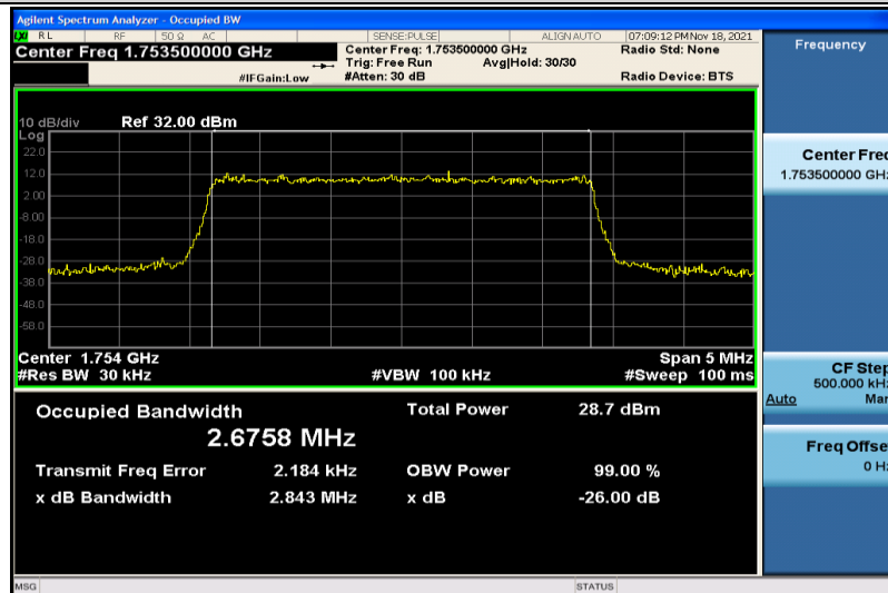
Band4-3MHz-QPSK-20385-15RB#0-2.6758
