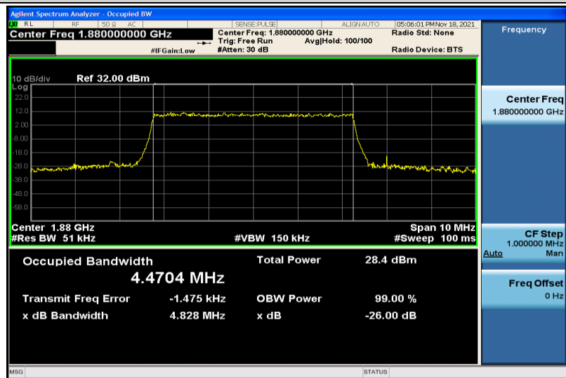
Band2-5MHz-16QAM-18900-25RB#0-4.4704
