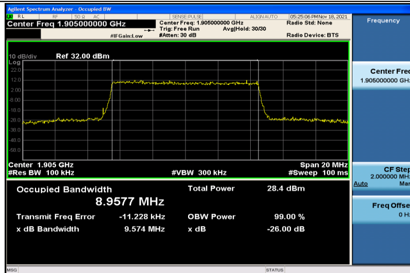
Band2-10MHz-16QAM-19150-50RB#0-8.9577
