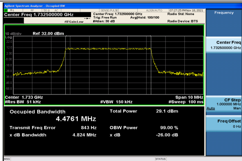
Band4-5MHz-QPSK-20175-25RB#0-4.4761
