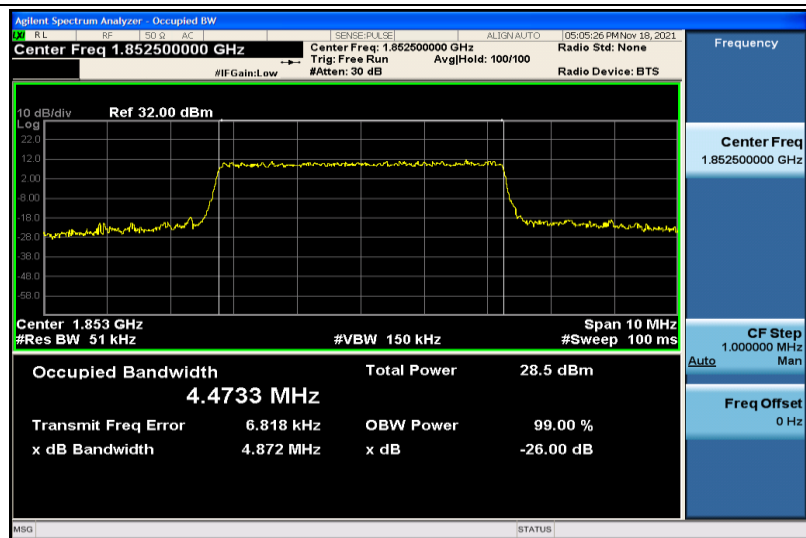
Band2-5MHz-16QAM-18625-25RB#0-4.4733
