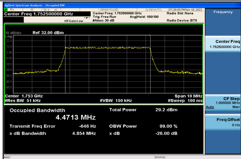
Band4-5MHz-QPSK-20375-25RB#0-4.4713
