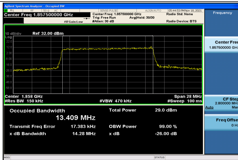
Band2-15MHz-16QAM-18675-75RB#0-13.409
