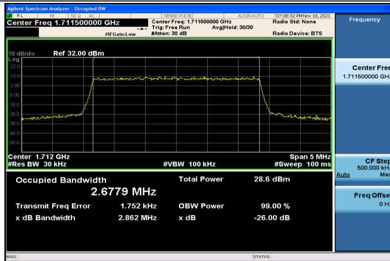
Band4-3MHz-QPSK-19965-15RB#0-2.6779
