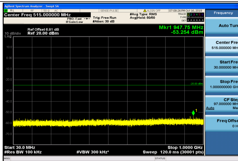
Band7-20MHz-16QAM-20850-1RB#0-30~1000MHz
