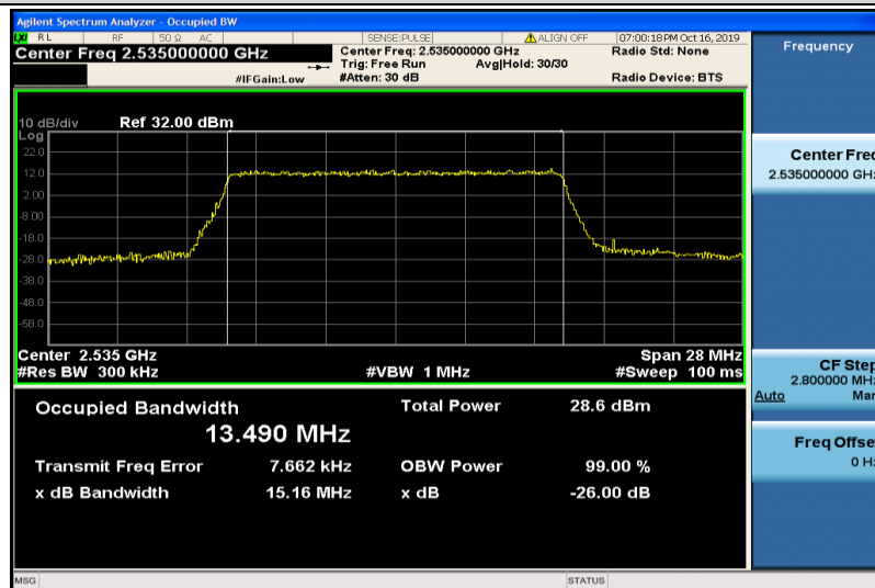
Band7-15MHz-QPSK-21100-75RB#0-13.490
