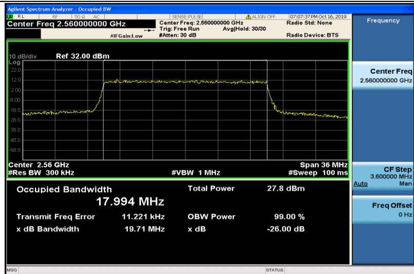
Band7-20MHz-16QAM-21350-100RB#0-17.994
