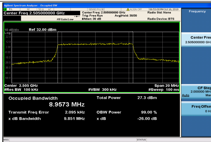
Band7-10MHz-16QAM-20800-50RB#0-8.9573
