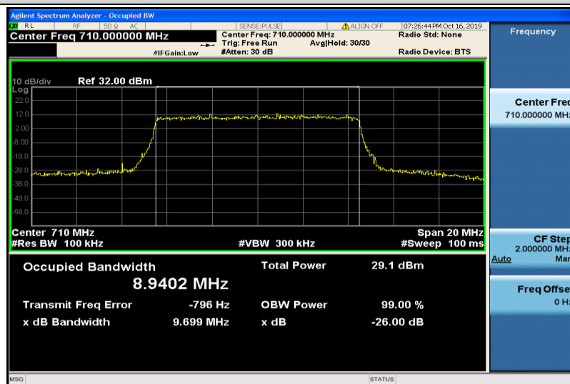
Band17-10MHz-QPSK-23790-50RB#0-8.9402
