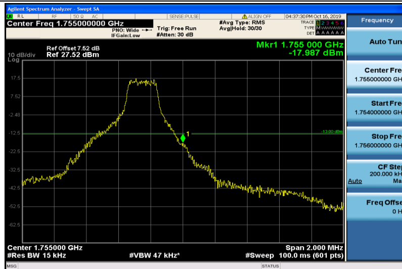
Band4-1.4MHz-QPSK-20393-1RB#5
