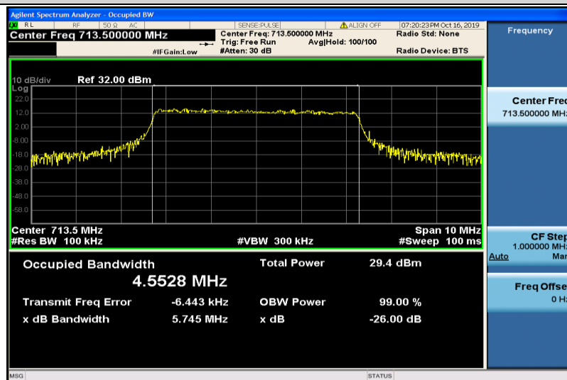
Band17-5MHz-QPSK-23825-25RB#0-4.5528
