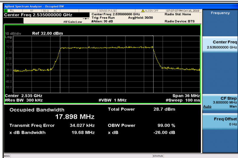
Band7-20MHz-QPSK-21100-100RB#0-17.898
