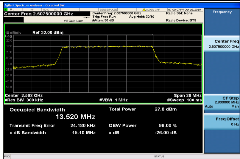
Band7-15MHz-16QAM-20825-75RB#0-13.520
