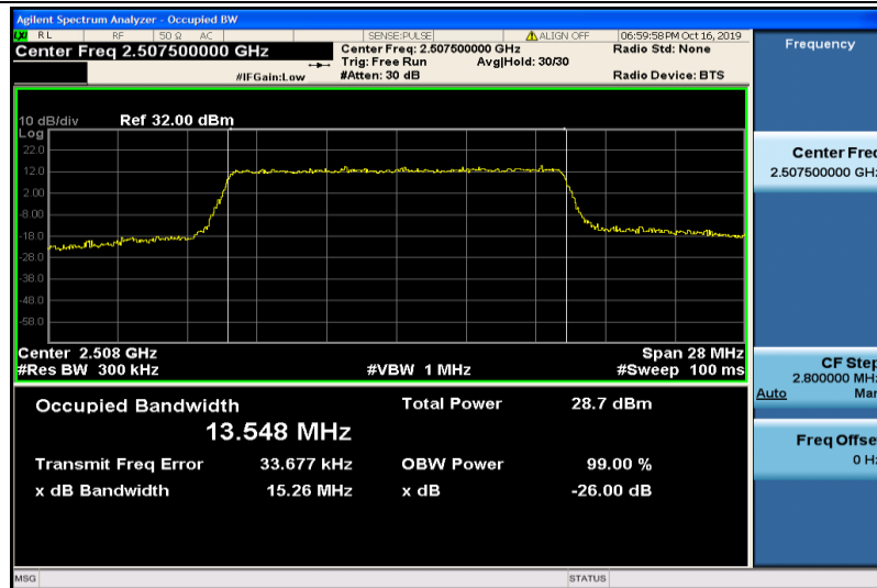
Band7-15MHz-QPSK-20825-75RB#0-13.548
