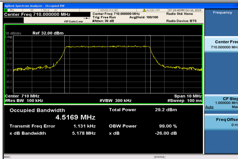
Band17-5MHz-QPSK-23790-25RB#0-4.5169
