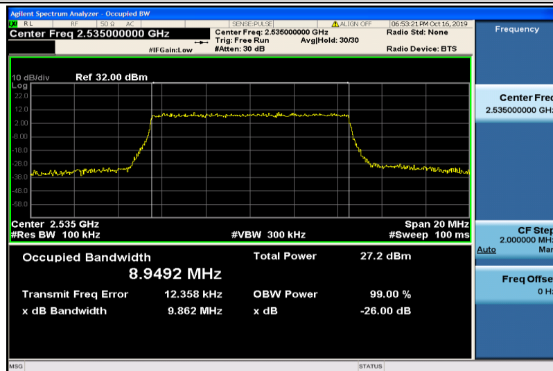
Band7-10MHz-16QAM-21100-50RB#0-8.9492
