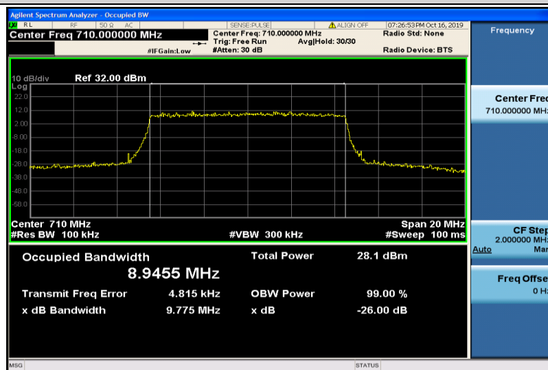
Band17-10MHz-16QAM-23790-50RB#0-8.9455
