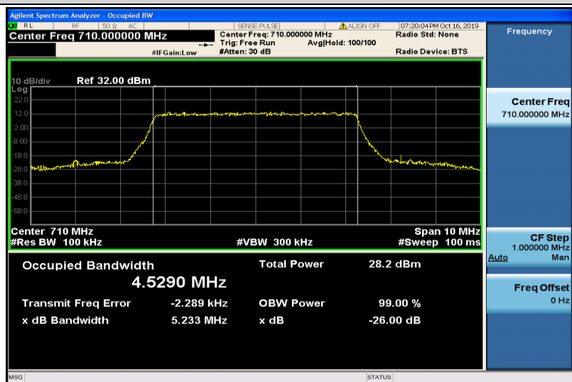
Band17-5MHz-16QAM-23790-25RB#0-4.5290
