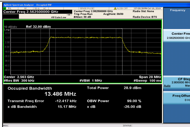
Band7-15MHz-QPSK-21375-75RB#0-13.486
