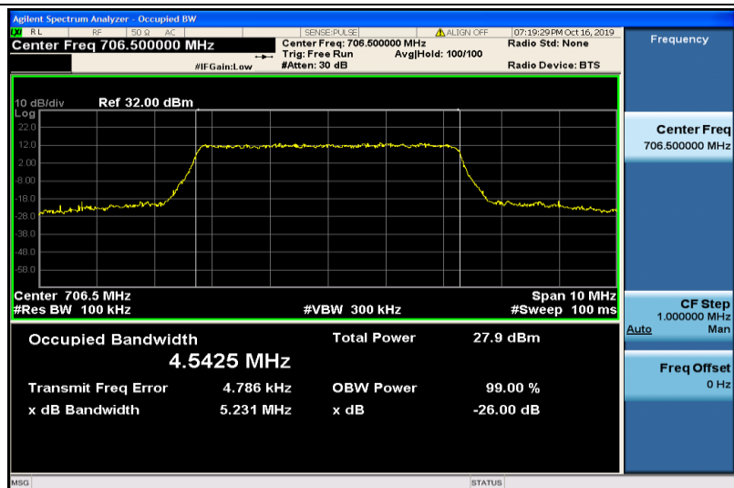
Band17-5MHz-16QAM-23755-25RB#0-4.5425
