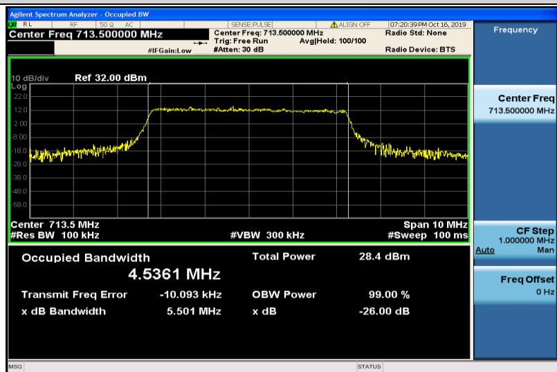
Band17-5MHz-16QAM-23825-25RB#0-4.5361
