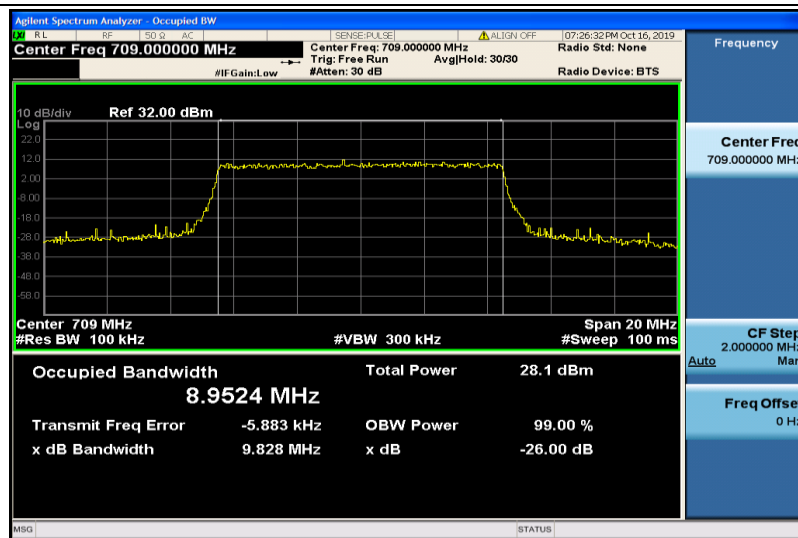
Band17-10MHz-16QAM-23780-50RB#0-8.9524
