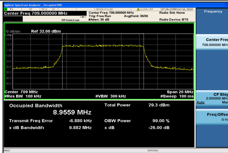
Band17-10MHz-QPSK-23780-50RB#0-8.9559
