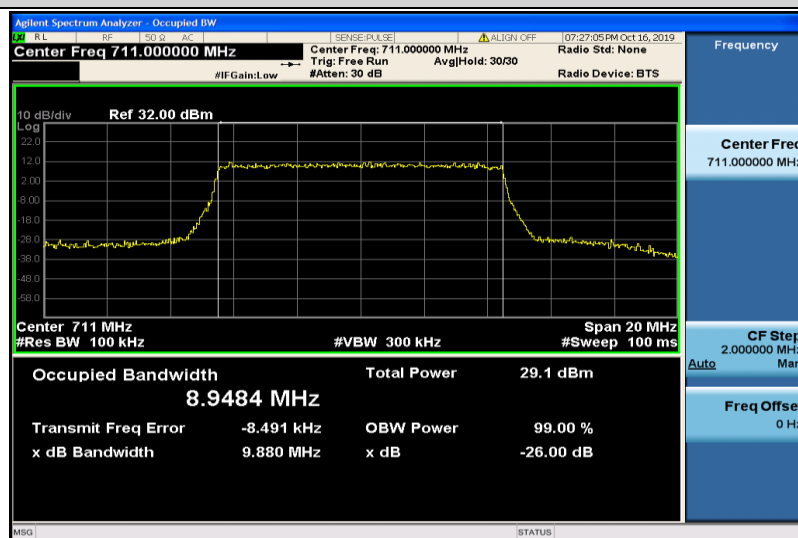
Band17-10MHz-QPSK-23800-50RB#0-8.9484
