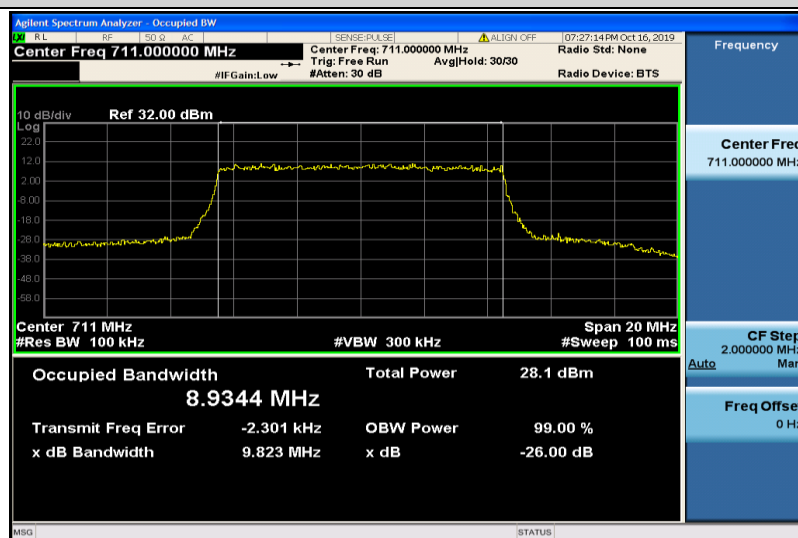
Band17-10MHz-16QAM-23800-50RB#0-8.9344
