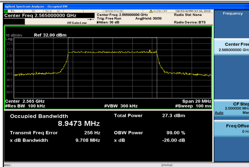
Band7-10MHz-16QAM-21400-50RB#0-8.9473
