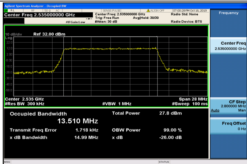
Band7-15MHz-16QAM-21100-75RB#0-13.510
