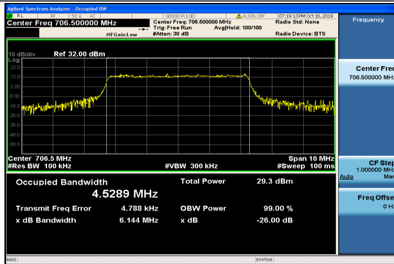
Band17-5MHz-QPSK-23755-25RB#0-4.5289
