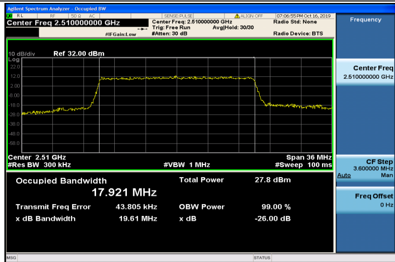
Band7-20MHz-16QAM-20850-100RB#0-17.921
