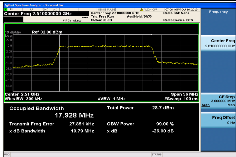
Band7-20MHz-QPSK-20850-100RB#0-17.928
