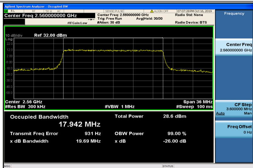
Band7-20MHz-QPSK-21350-100RB#0-17.942
