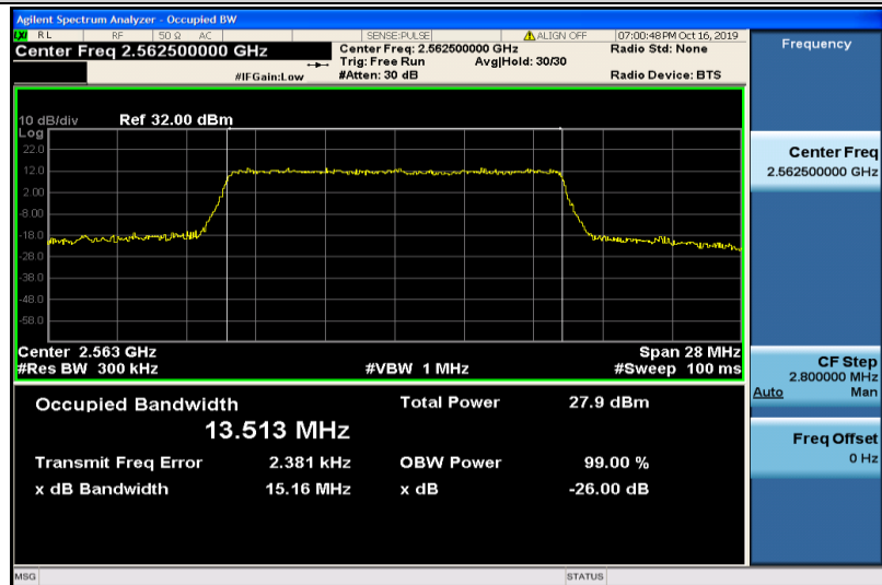
Band7-15MHz-16QAM-21375-75RB#0-13.513
