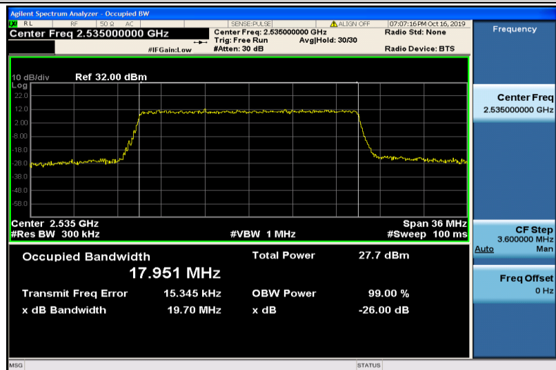
Band7-20MHz-16QAM-21100-100RB#0-17.951
