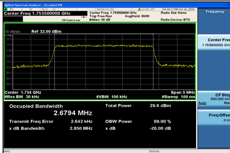
Band4-3MHz-QPSK-20385-15RB#0-2.6794
