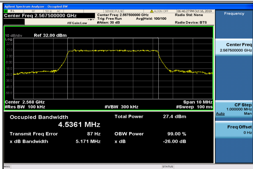
Band7-5MHz-16QAM-21425-25RB#0-4.5361
