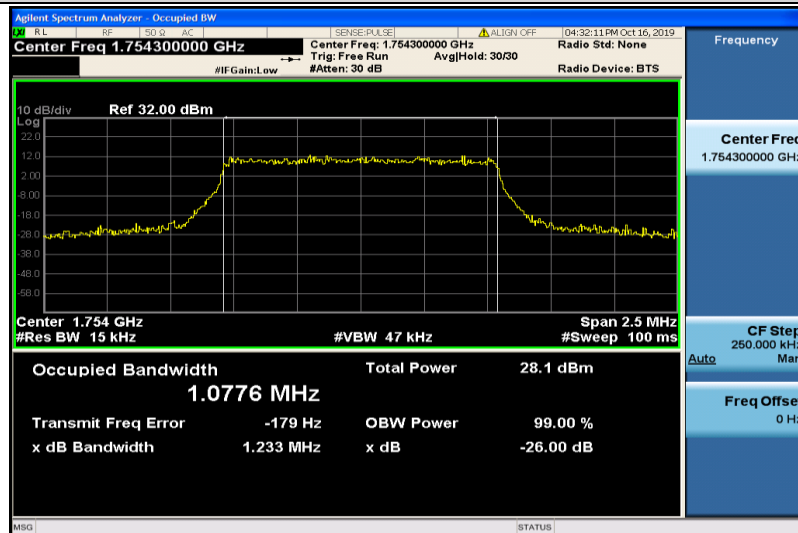
Band4-1.4MHz-16QAM-20393-6RB#0-1.0776
