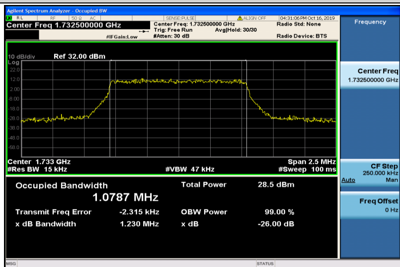
Band4-1.4MHz-QPSK-20175-6RB#0-1.0787
