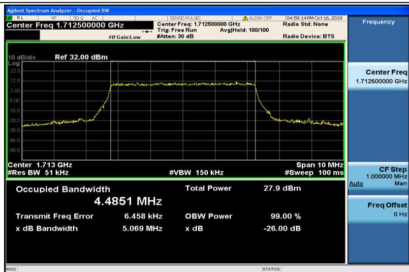
Band4-5MHz-16QAM-19975-25RB#0-4.4851
