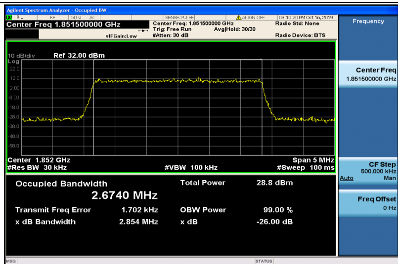
Band2-3MHz-QPSK-18615-15RB#0-2.6740
