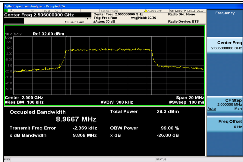
Band7-10MHz-QPSK-20800-50RB#0-8.9667
