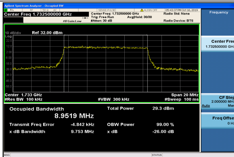
Band4-10MHz-16QAM-20175-50RB#0-8.9519
