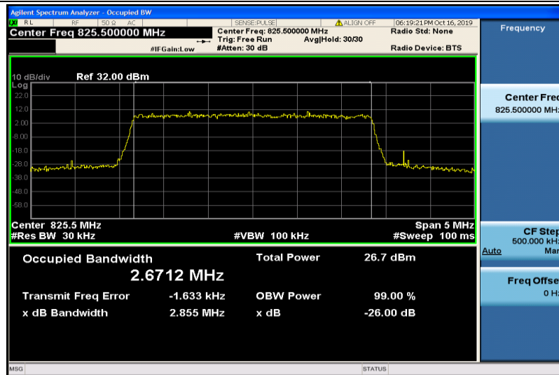
Band5-3MHz-16QAM-20415-15RB#0-2.6712
