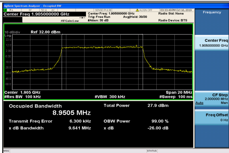
Band2-10MHz-16QAM-19150-50RB#0-8.9505
