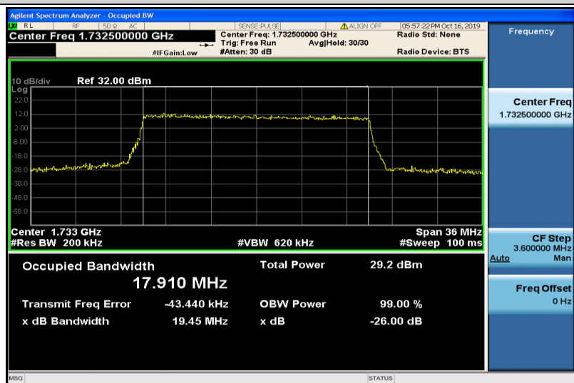
Band4-20MHz-16QAM-20175-100RB#0-17.910
