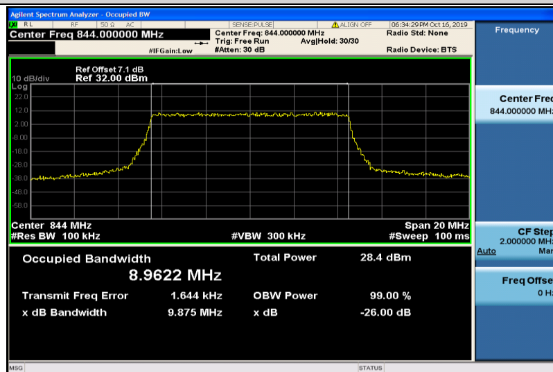
Band5-10MHz-QPSK-20600-50RB#0-8.9622
