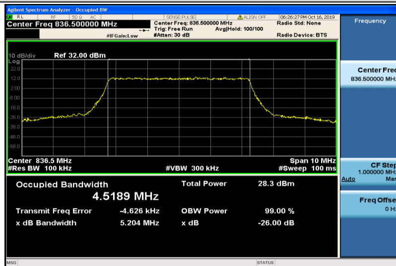
Band5-5MHz-QPSK-20525-25RB#0-4.5189
