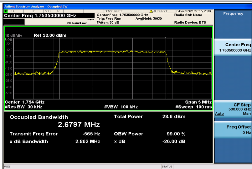
Band4-3MHz-16QAM-20385-15RB#0-2.6797
