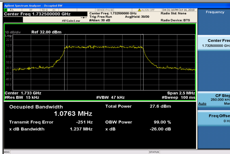
Band4-1.4MHz-16QAM-20175-6RB#0-1.0763
