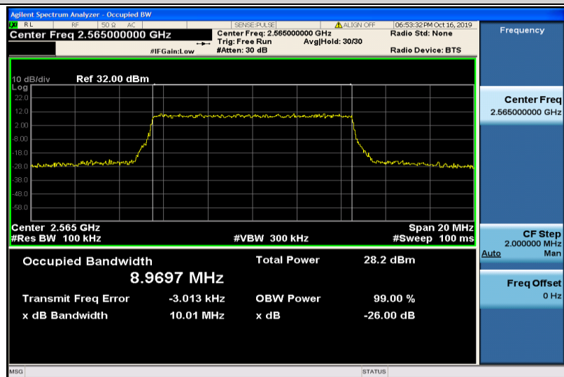
Band7-10MHz-QPSK-21400-50RB#0-8.9697
