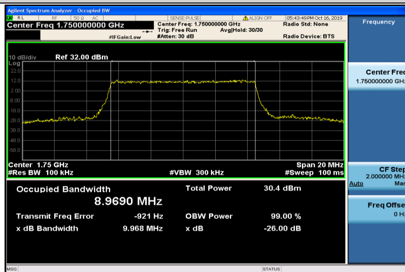
Band4-10MHz-QPSK-20350-50RB#0-8.9690
