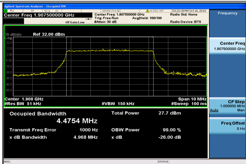
Band2-5MHz-16QAM-19175-25RB#0-4.4754
