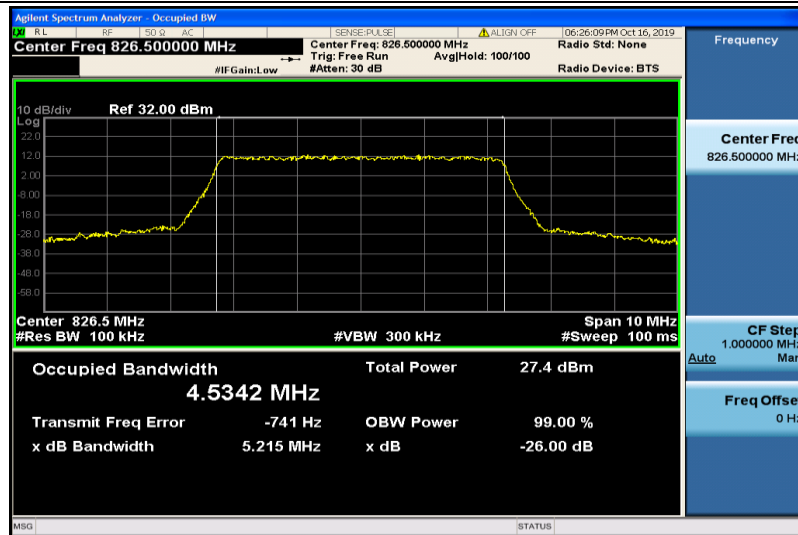
Band5-5MHz-16QAM-20425-25RB#0-4.5342
