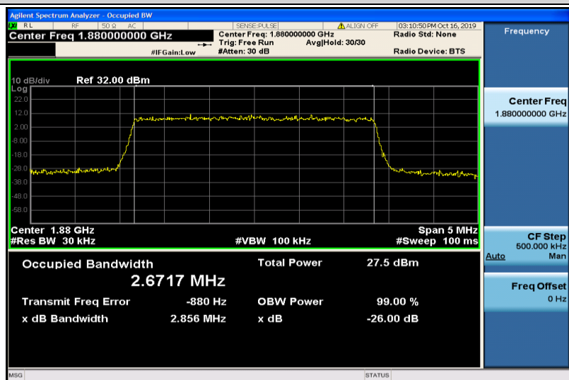
Band2-3MHz-16QAM-18900-15RB#0-2.6717
