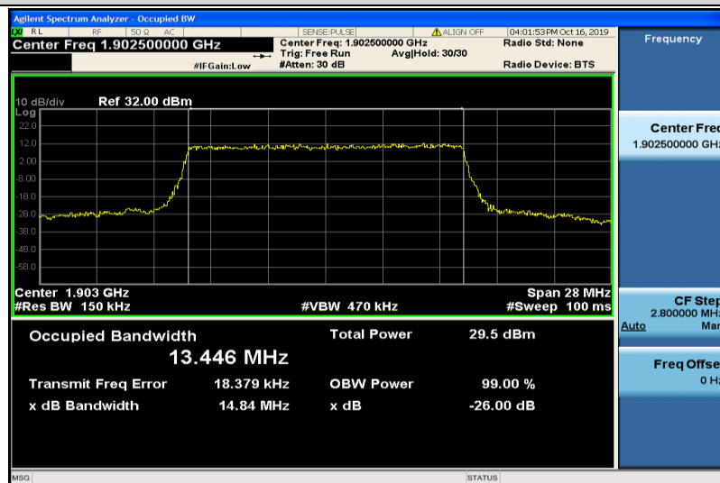
Band2-15MHz-QPSK-19125-75RB#0-13.446
