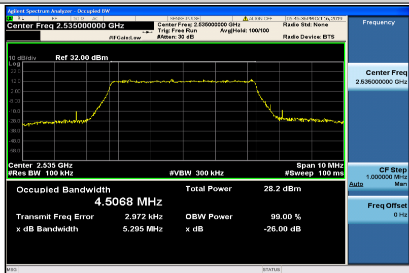
Band7-5MHz-QPSK-21100-25RB#0-4.5068
