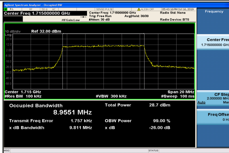
Band4-10MHz-16QAM-20000-50RB#0-8.9551
