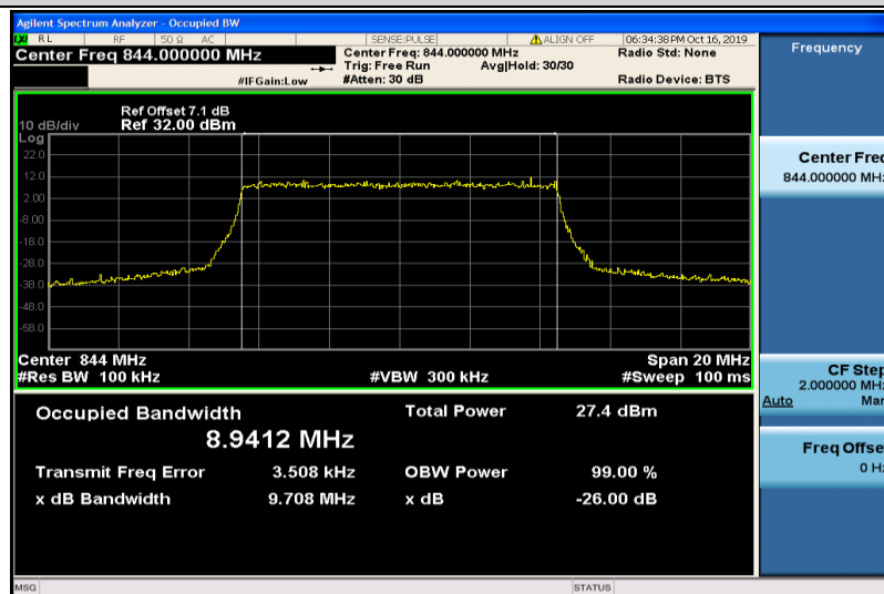
Band5-10MHz-16QAM-20600-50RB#0-8.9412
