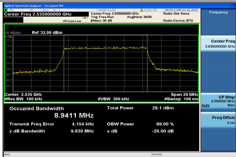
Band7-10MHz-QPSK-21100-50RB#0-8.9411
