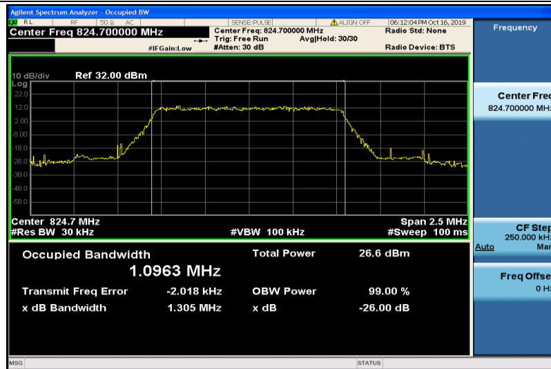
Band5-1.4MHz-16QAM-20407-6RB#0-1.0963
