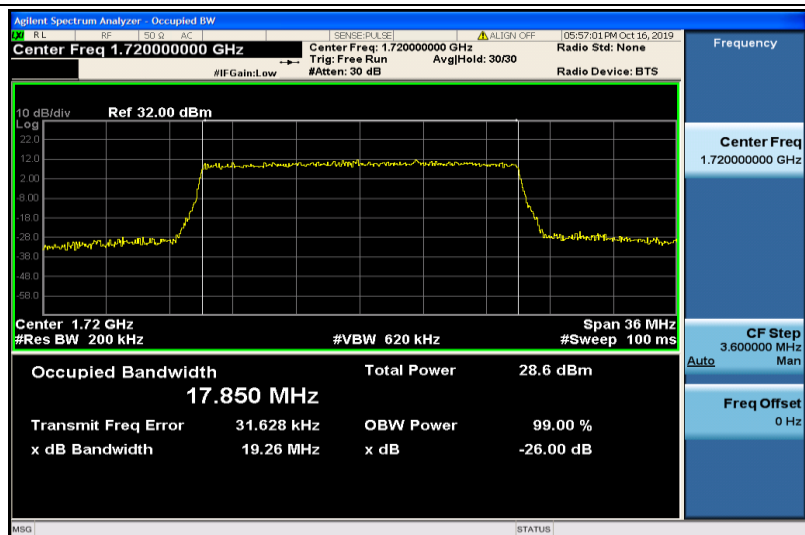
Band4-20MHz-16QAM-20050-100RB#0-17.850
