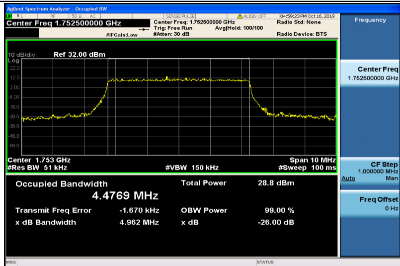
Band4-5MHz-16QAM-20375-25RB#0-4.4769
