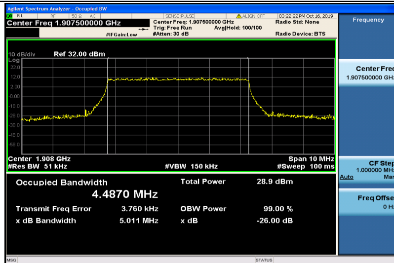
Band2-5MHz-QPSK-19175-25RB#0-4.4870
