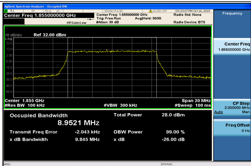
Band2-10MHz-16QAM-18650-50RB#0-8.9521
