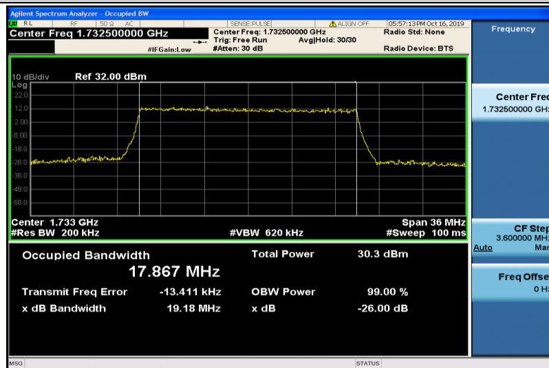
Band4-20MHz-QPSK-20175-100RB#0-17.867
