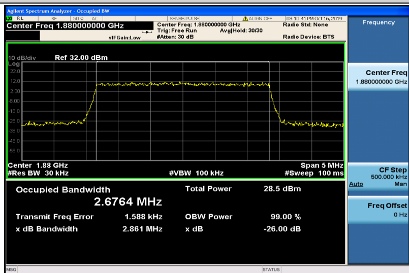
Band2-3MHz-QPSK-18900-15RB#0-2.6764
