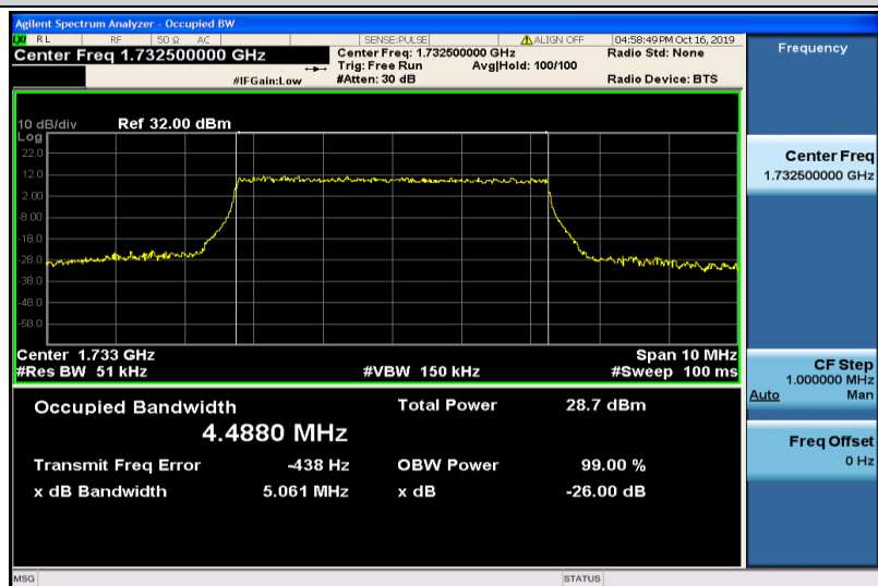
Band4-5MHz-16QAM-20175-25RB#0-4.4880
