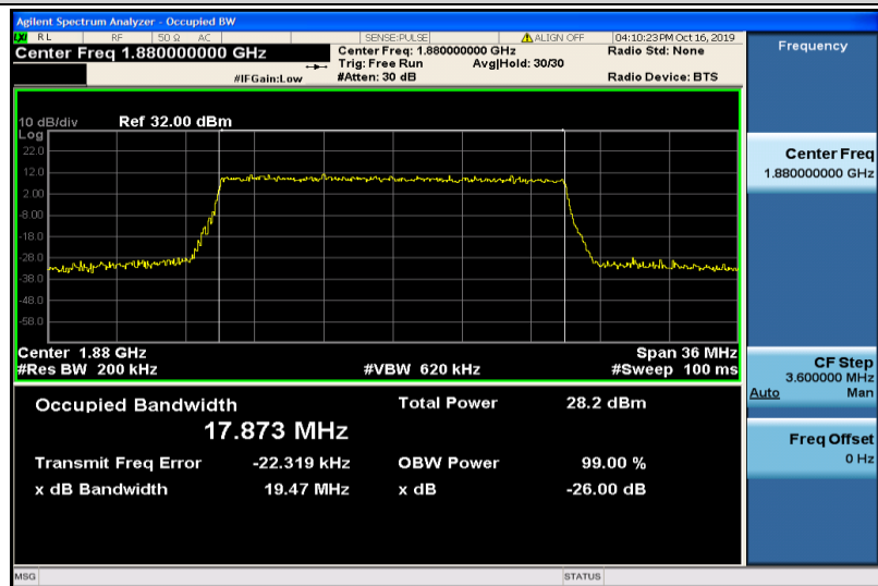
Band2-20MHz-16QAM-18900-100RB#0-17.873
