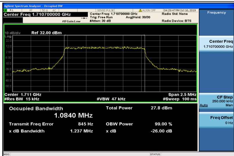
Band4-1.4MHz-QPSK-19957-6RB#0-1.0840
