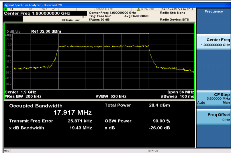
Band2-20MHz-16QAM-19100-100RB#0-17.917
