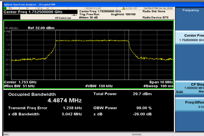
Band4-5MHz-QPSK-20375-25RB#0-4.4874
