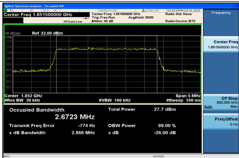
Band2-3MHz-16QAM-18615-15RB#0-2.6723
