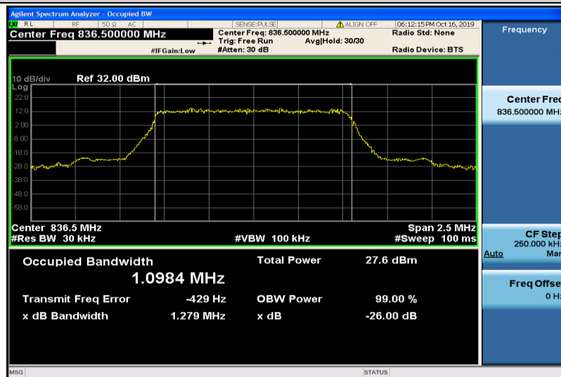
Band5-1.4MHz-QPSK-20525-6RB#0-1.0984
