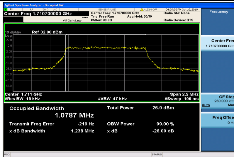
Band4-1.4MHz-16QAM-19957-6RB#0-1.0787
