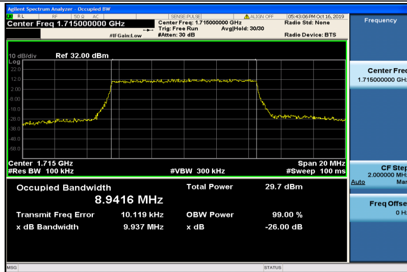
Band4-10MHz-QPSK-20000-50RB#0-8.9416
