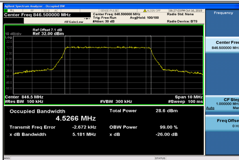
Band5-5MHz-QPSK-20625-25RB#0-4.5266
