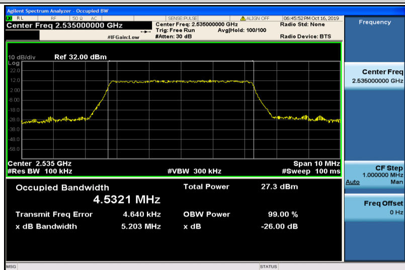
Band7-5MHz-16QAM-21100-25RB#0-4.5321
