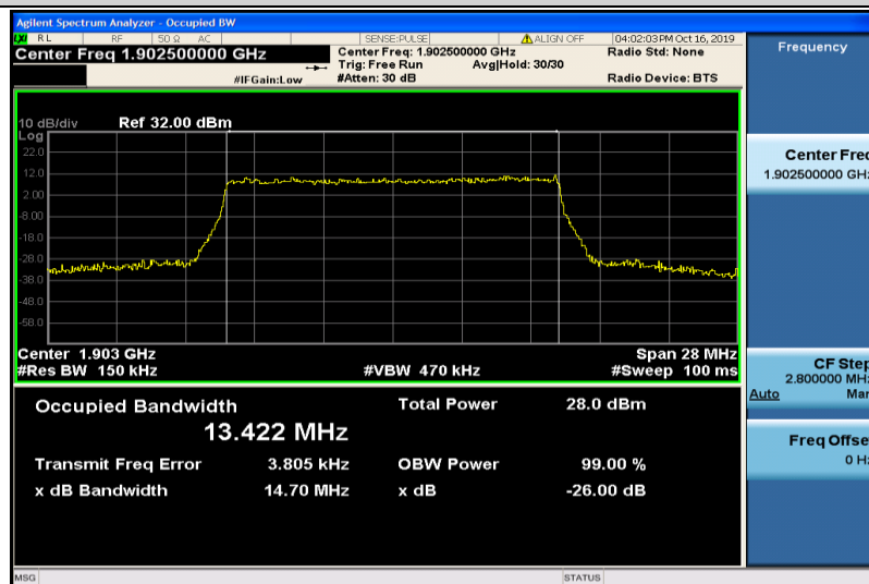
Band2-15MHz-16QAM-19125-75RB#0-13.422
