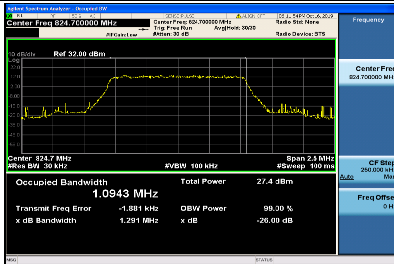
Band5-1.4MHz-QPSK-20407-6RB#0-1.0943
