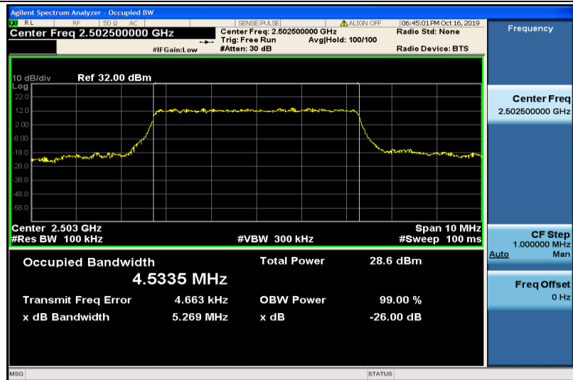
Band7-5MHz-QPSK-20775-25RB#0-4.5335
