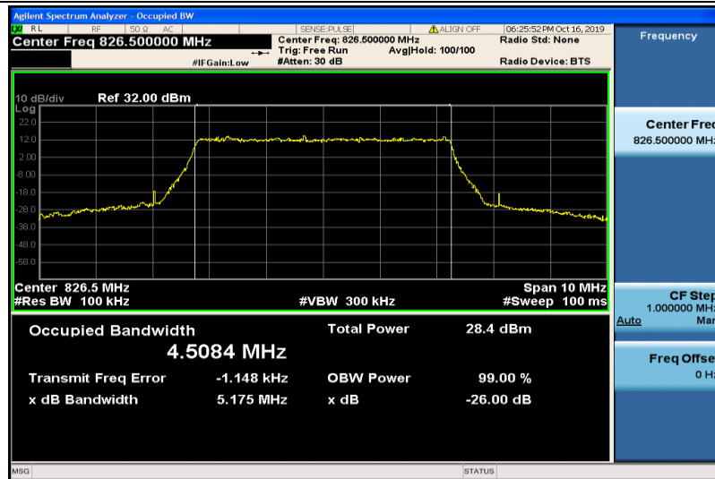
Band5-5MHz-QPSK-20425-25RB#0-4.5084
