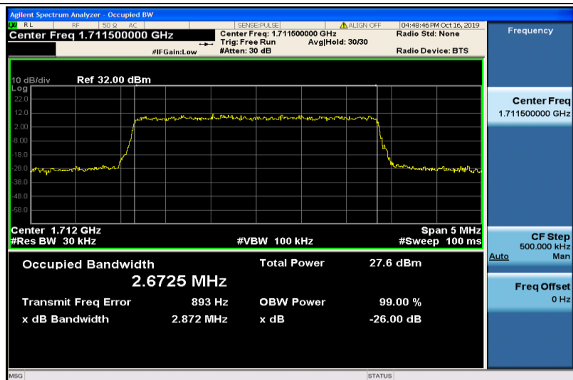
Band4-3MHz-16QAM-19965-15RB#0-2.6725
