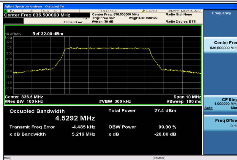
Band5-5MHz-16QAM-20525-25RB#0-4.5292
