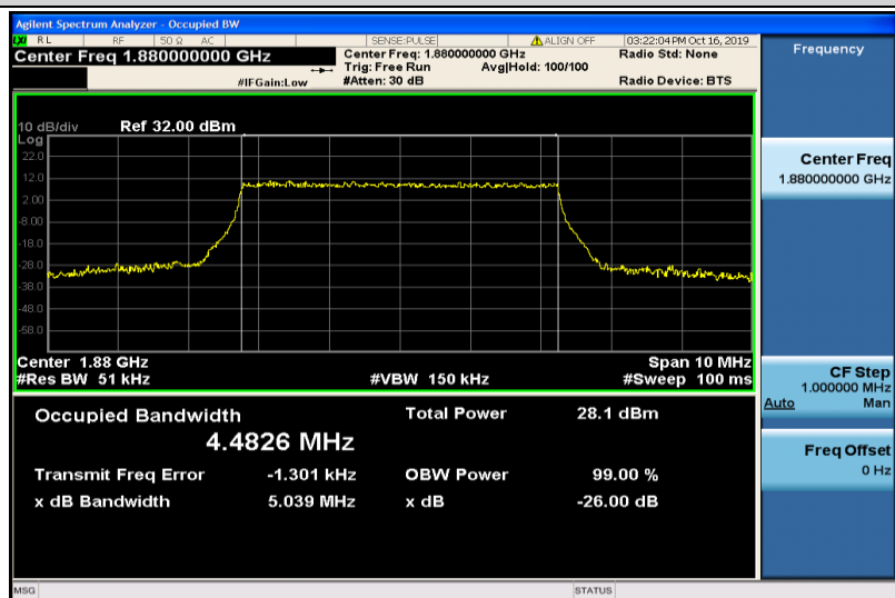
Band2-5MHz-16QAM-18900-25RB#0-4.4826
