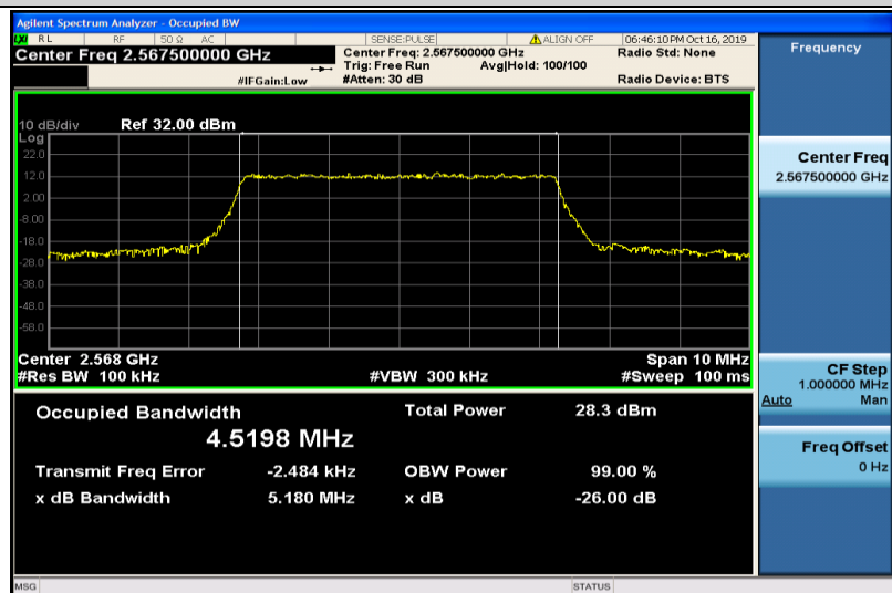
Band7-5MHz-QPSK-21425-25RB#0-4.5198
