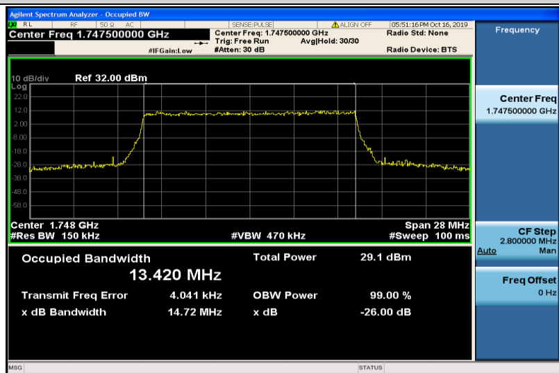
Band4-15MHz-16QAM-20325-75RB#0-13.420
