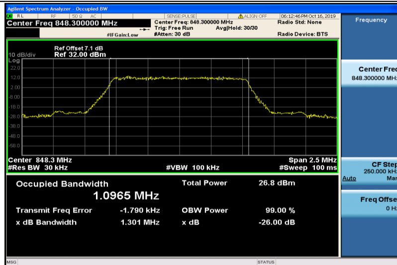
Band5-1.4MHz-16QAM-20643-6RB#0-1.0965
