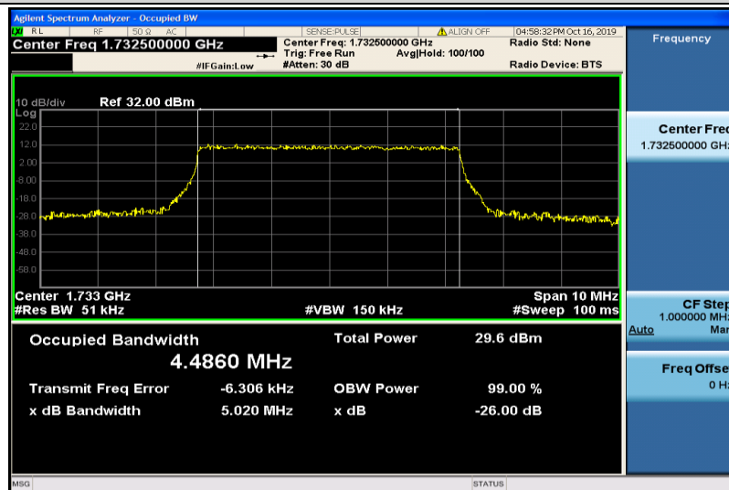
Band4-5MHz-QPSK-20175-25RB#0-4.4860
