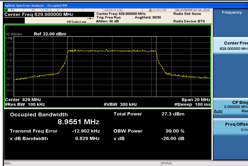
Band5-10MHz-16QAM-20450-50RB#0-8.9551
