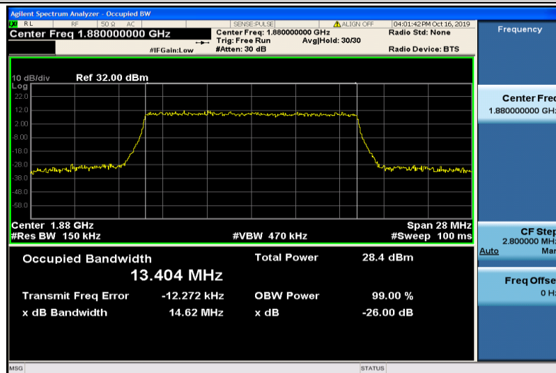
Band2-15MHz-16QAM-18900-75RB#0-13.404
