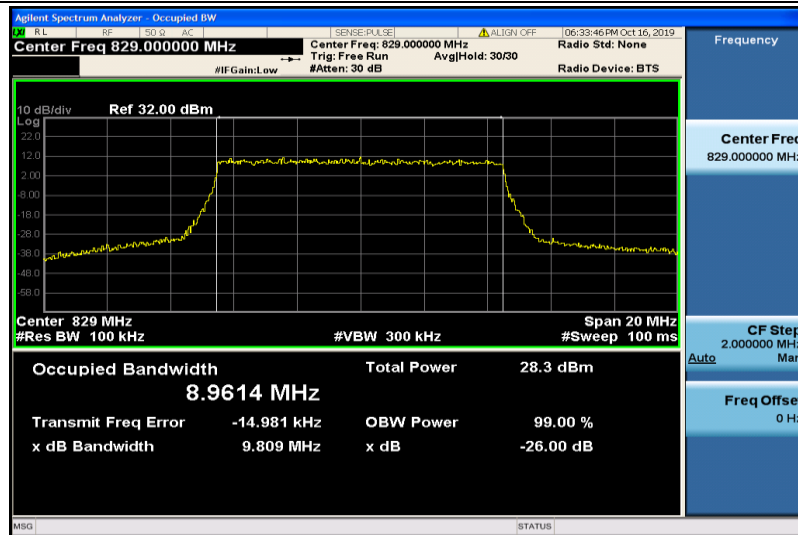
Band5-10MHz-QPSK-20450-50RB#0-8.9614
