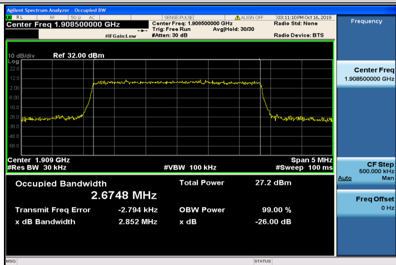
Band2-3MHz-16QAM-19185-15RB#0-2.6748
