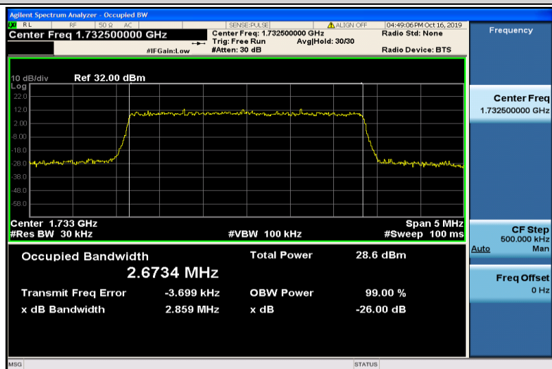
Band4-3MHz-16QAM-20175-15RB#0-2.6734
