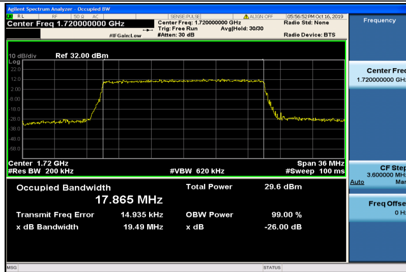
Band4-20MHz-QPSK-20050-100RB#0-17.865
