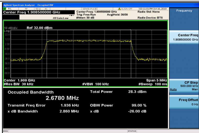
Band2-3MHz-QPSK-19185-15RB#0-2.6780
