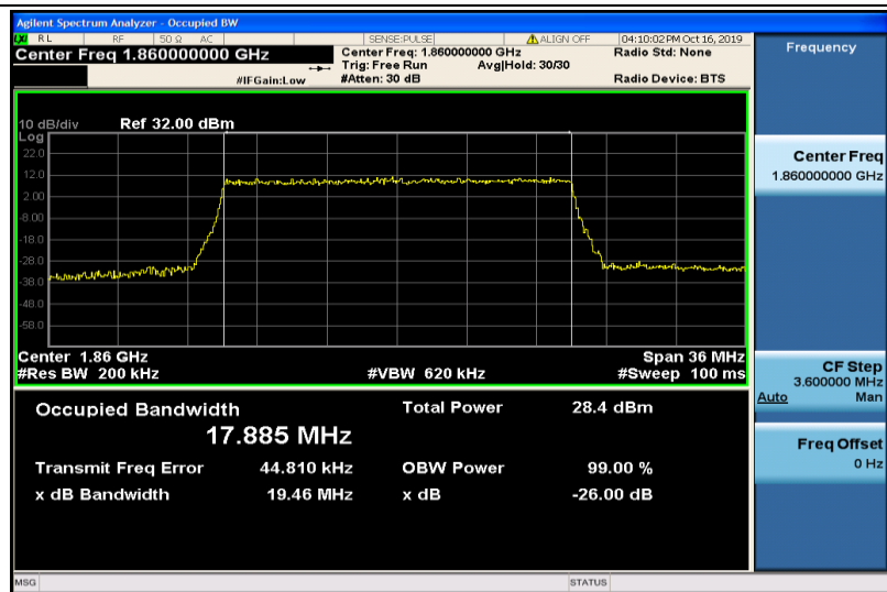
Band2-20MHz-16QAM-18700-100RB#0-17.885
