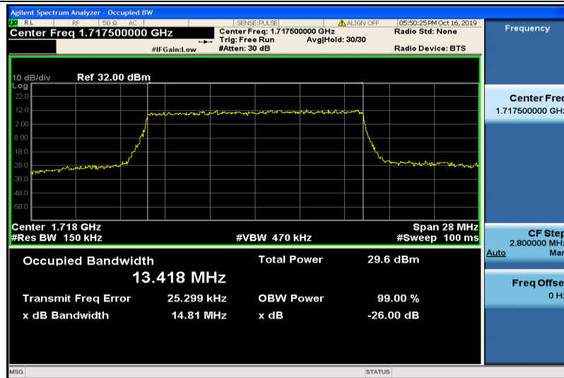
Band4-15MHz-QPSK-20025-75RB#0-13.418
