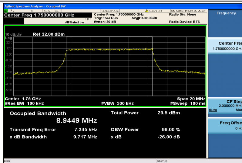
Band4-10MHz-16QAM-20350-50RB#0-8.9449
