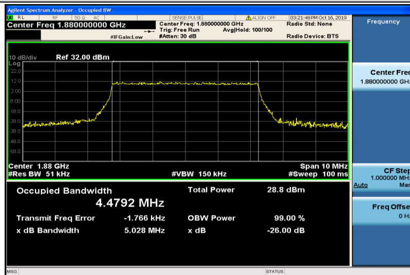
Band2-5MHz-QPSK-18900-25RB#0-4.4792
