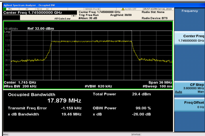
Band4-20MHz-16QAM-20300-100RB#0-17.879
