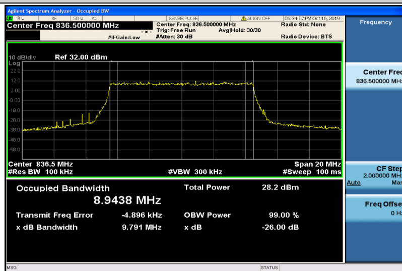
Band5-10MHz-QPSK-20525-50RB#0-8.9438
