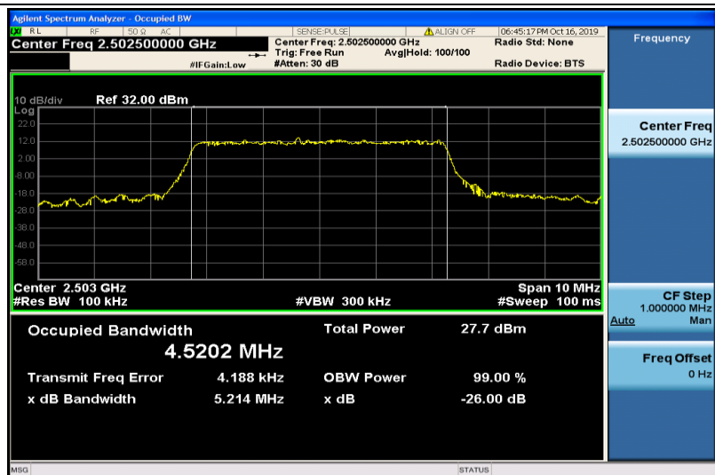
Band7-5MHz-16QAM-20775-25RB#0-4.5202
