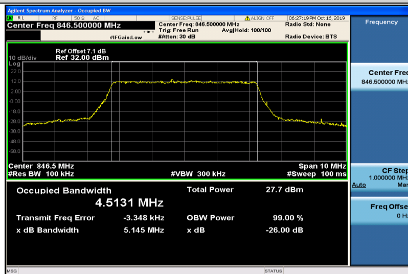
Band5-5MHz-16QAM-20625-25RB#0-4.5131
