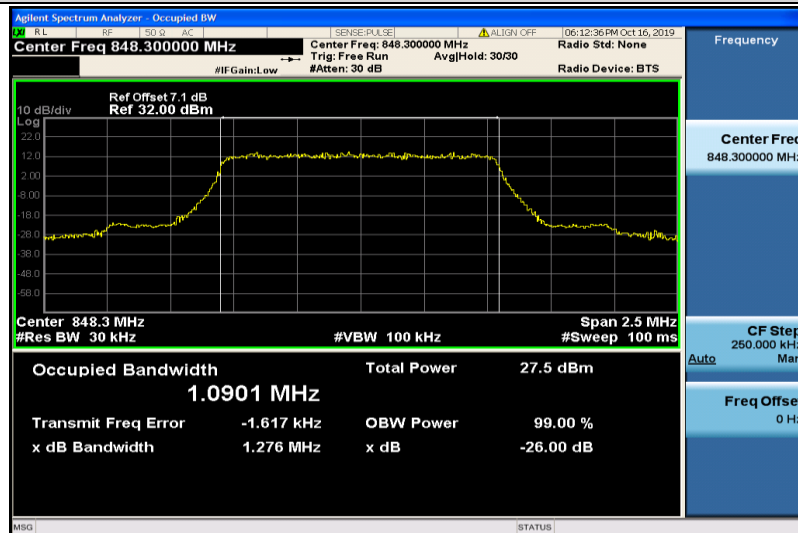
Band5-1.4MHz-QPSK-20643-6RB#0-1.0901
