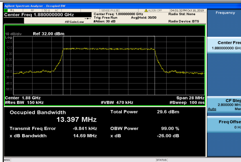
Band2-15MHz-QPSK-18900-75RB#0-13.397
