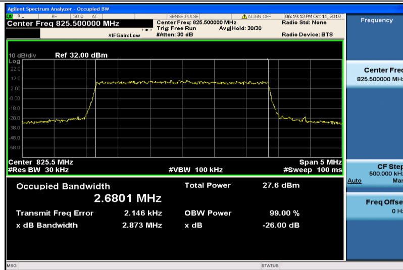
Band5-3MHz-QPSK-20415-15RB#0-2.6801
