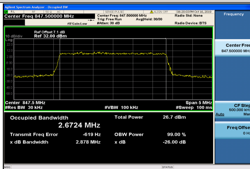
Band5-3MHz-16QAM-20635-15RB#0-2.6724
