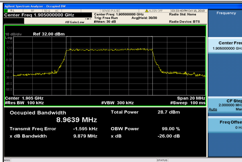
Band2-10MHz-QPSK-19150-50RB#0-8.9639
