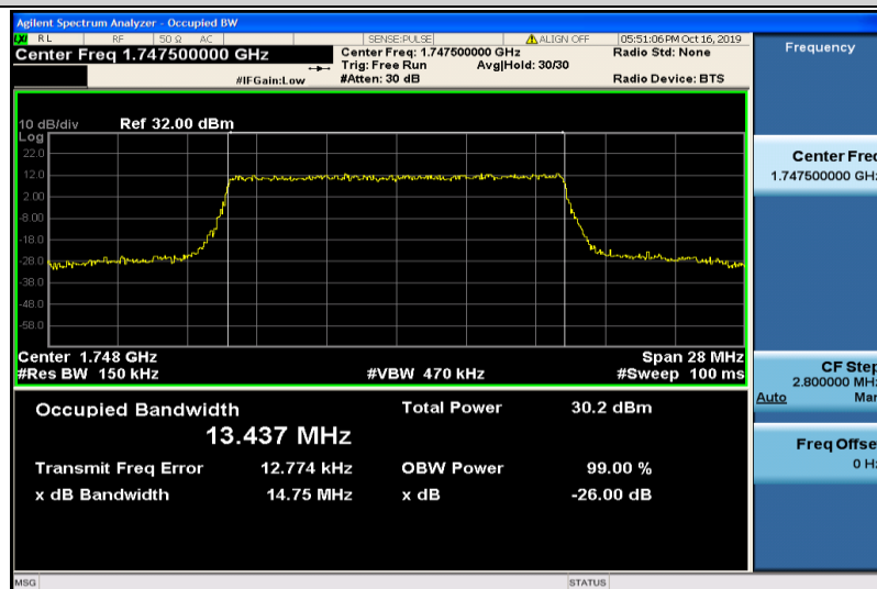
Band4-15MHz-QPSK-20325-75RB#0-13.437
