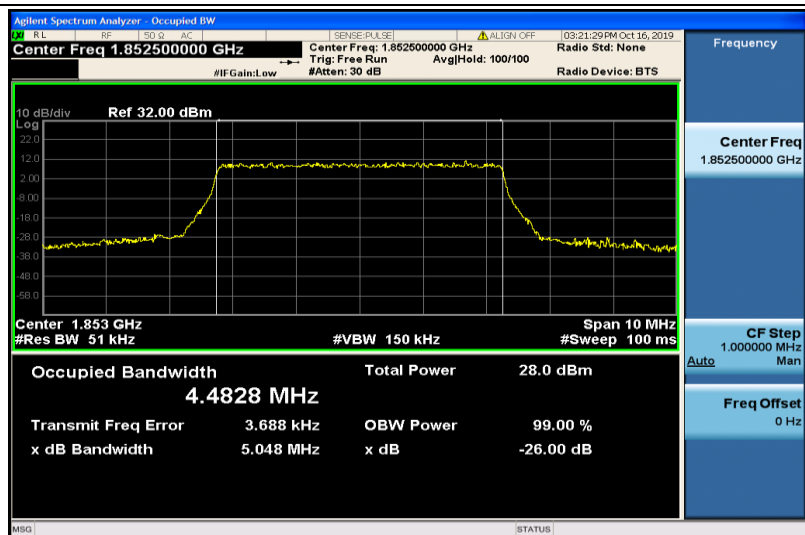
Band2-5MHz-16QAM-18625-25RB#0-4.4828
