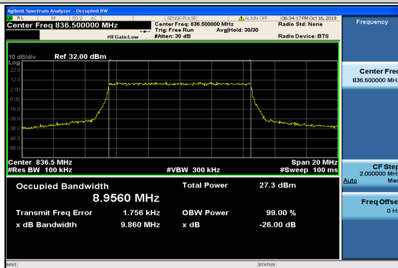
Band5-10MHz-16QAM-20525-50RB#0-8.9560
