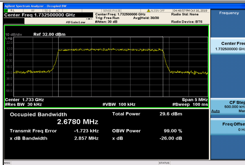
Band4-3MHz-QPSK-20175-15RB#0-2.6780
