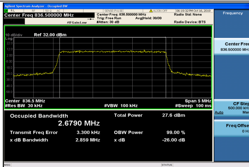
Band5-3MHz-QPSK-20525-15RB#0-2.6790
