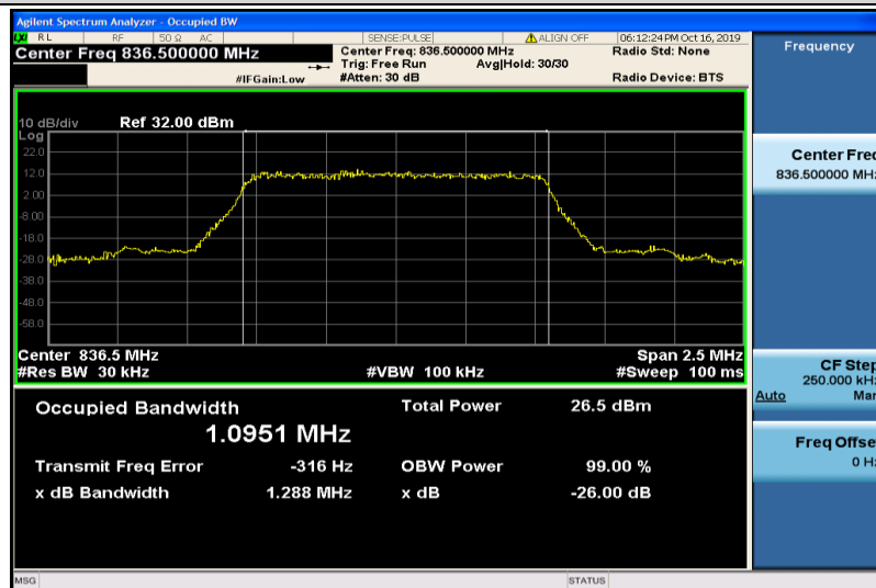
Band5-1.4MHz-16QAM-20525-6RB#0-1.0951
