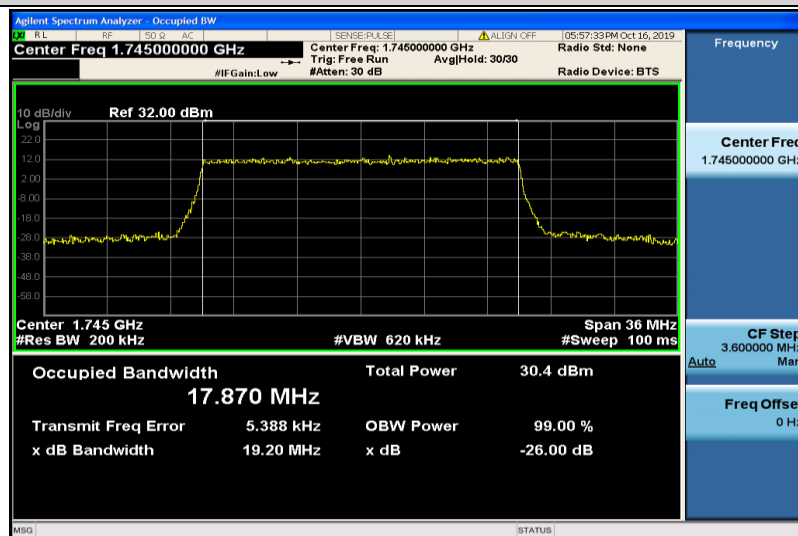
Band4-20MHz-QPSK-20300-100RB#0-17.870
