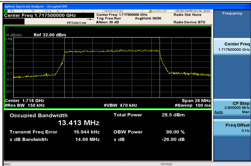
Band4-15MHz-16QAM-20025-75RB#0-13.413
