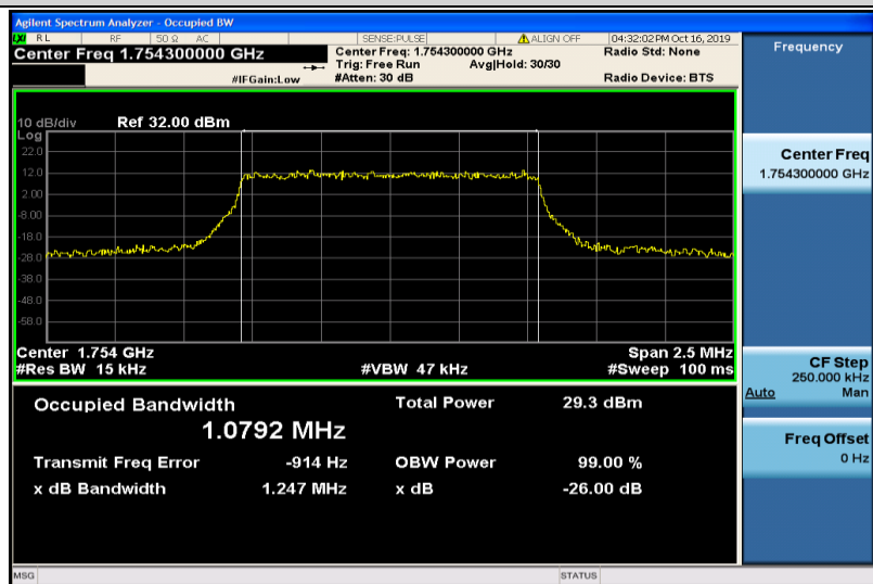
Band4-1.4MHz-QPSK-20393-6RB#0-1.0792
