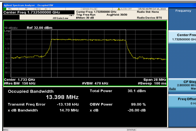
Band4-15MHz-QPSK-20175-75RB#0-13.398
