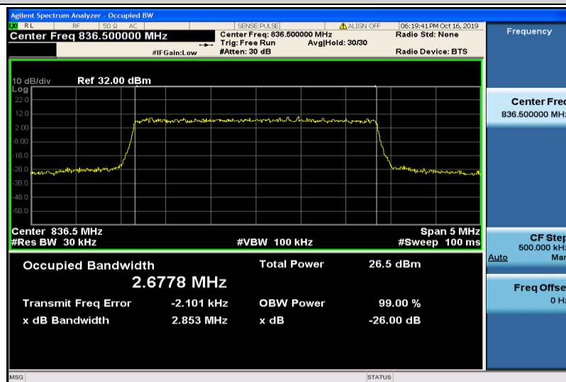
Band5-3MHz-16QAM-20525-15RB#0-2.6778
