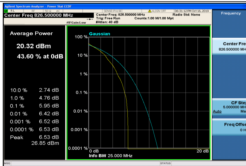
Band5-5MHz-QPSK-20425-1RB#0
