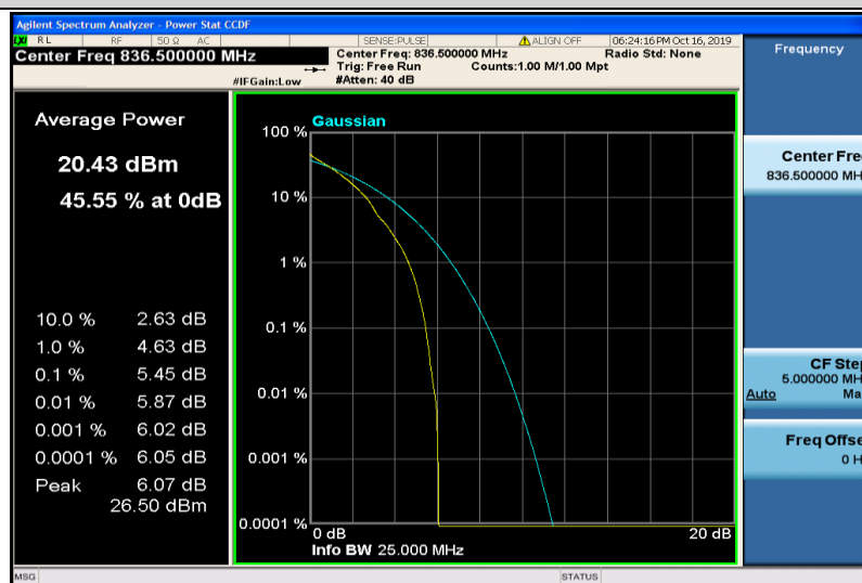
Band5-3MHz-QPSK-20525-1RB#0
