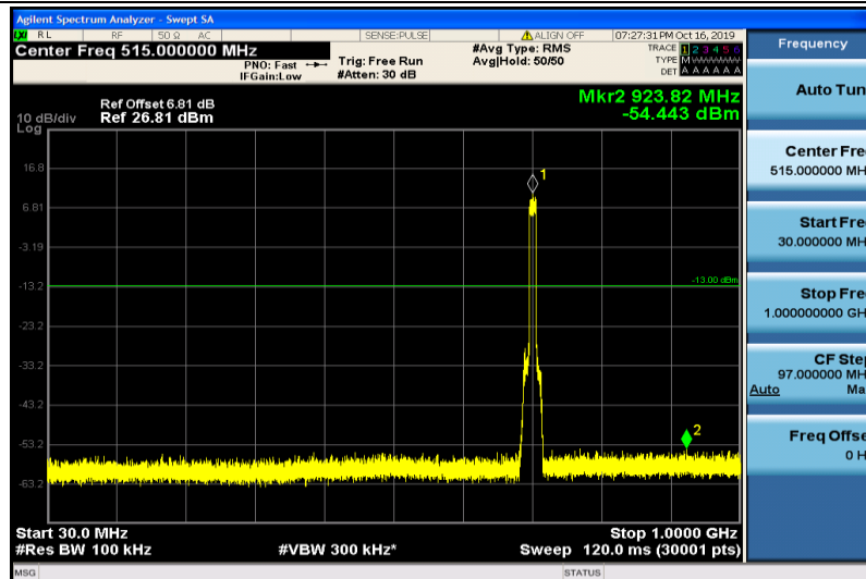
Band17-10MHz-QPSK-23780-1RB#0-30~1000MHz
