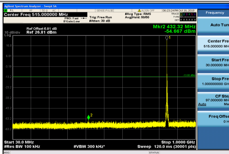
Band5-3MHz-16QAM-20635-1RB#0-30~1000MHz
