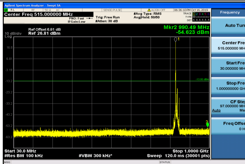
Band5-10MHz-QPSK-20525-1RB#0-30~1000MHz
