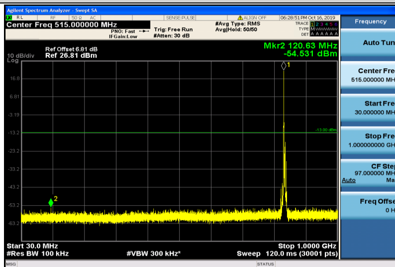
Band5-5MHz-QPSK-20525-1RB#0-30~1000MHz
