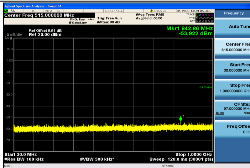
Band7-5MHz-QPSK-21425-1RB#0-30~1000MHz
