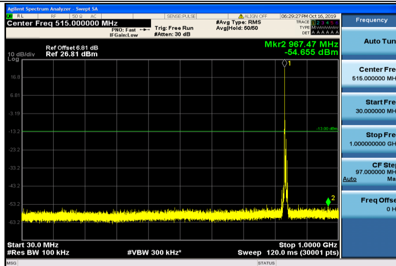
Band5-5MHz-16QAM-20525-1RB#0-30~1000MHz
