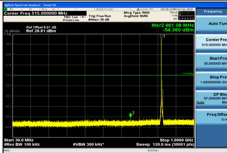
Band5-5MHz-16QAM-20425-1RB#0-30~1000MHz
