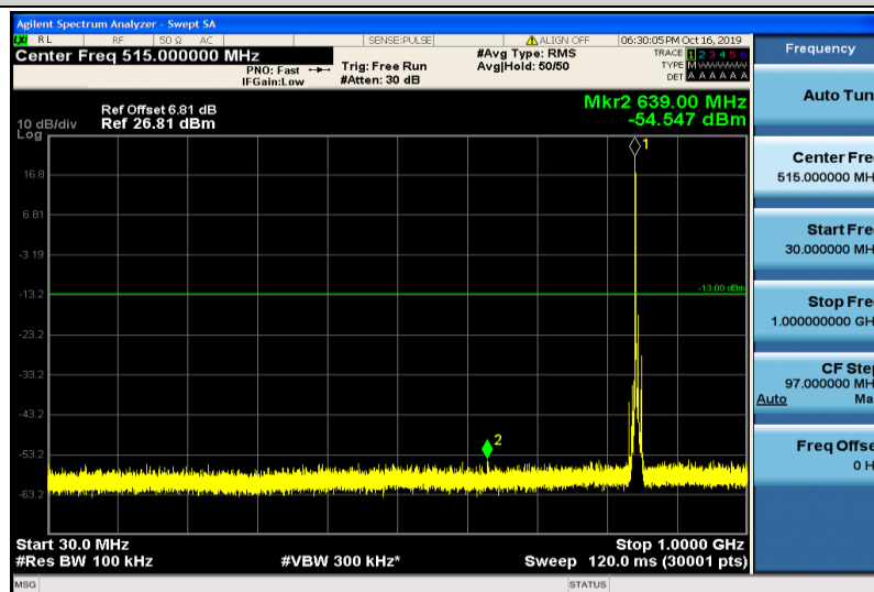
Band5-5MHz-QPSK-20625-1RB#0-30~1000MHz
