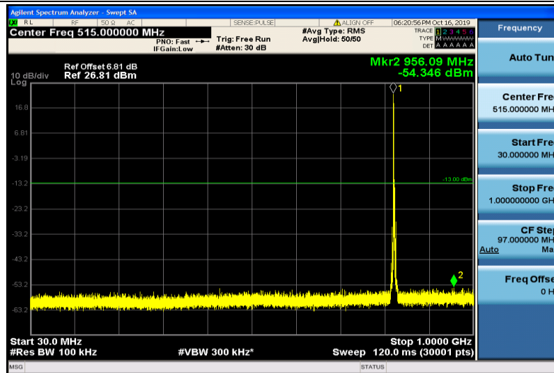
Band5-3MHz-16QAM-20415-1RB#0-30~1000MHz
