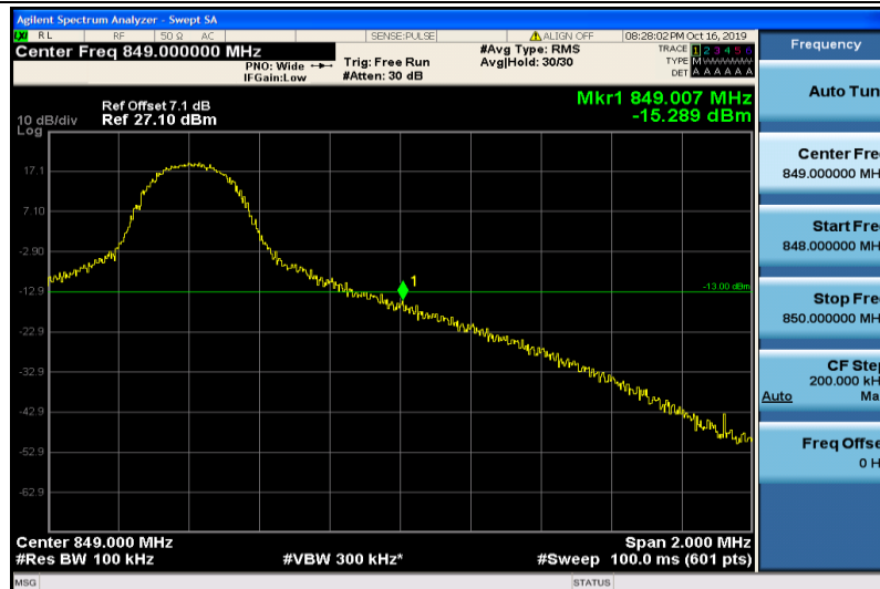
Band5-10MHz-QPSK-20600-1RB#49
