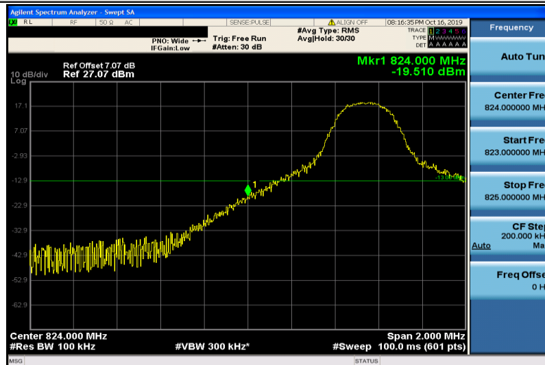
Band5-5MHz-QPSK-20425-1RB#0
