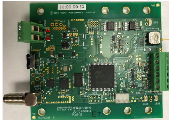
Channel selection rotary switch
