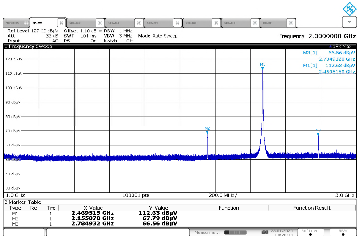
Figure A-10: 1GHz-3GHz (Conducted)
