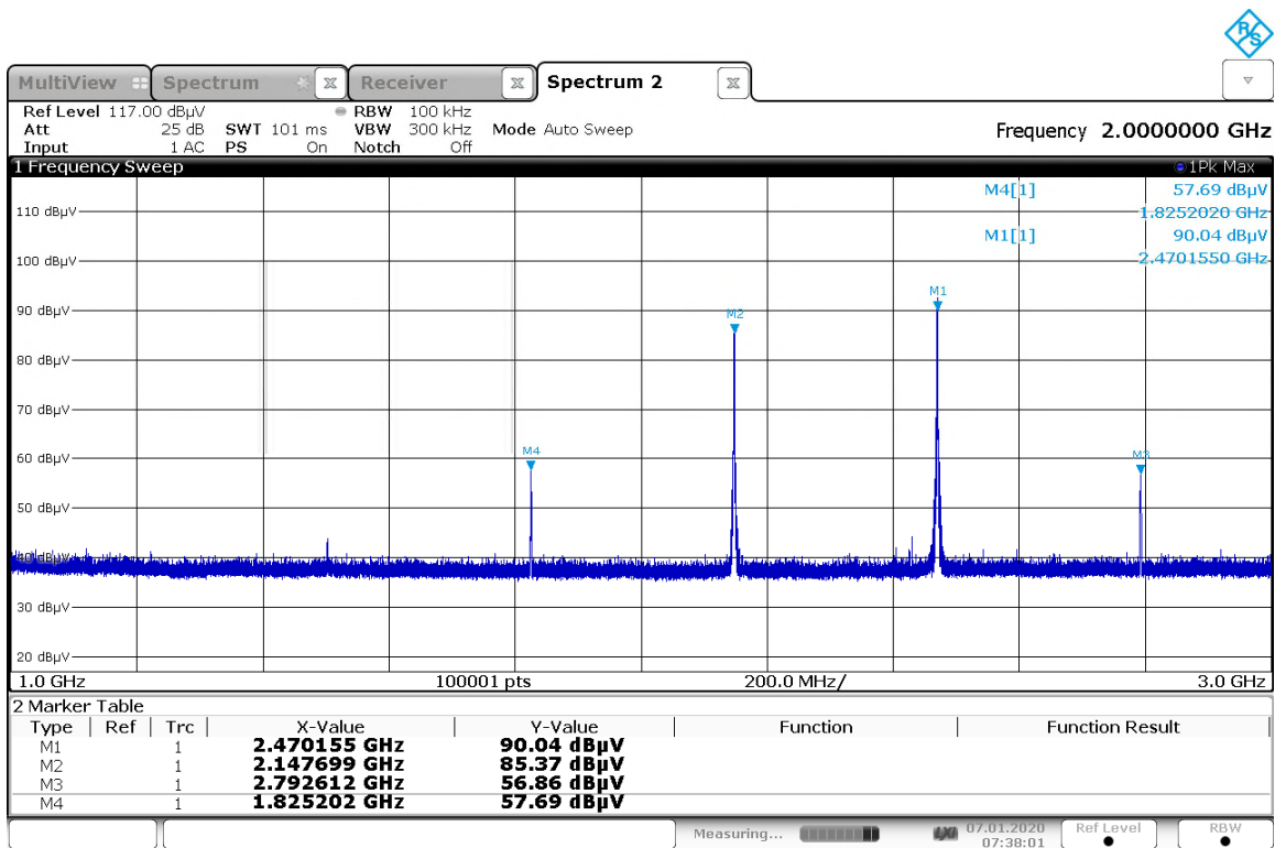
Figure A-4: 1GHz-3GHz (Radiated)
