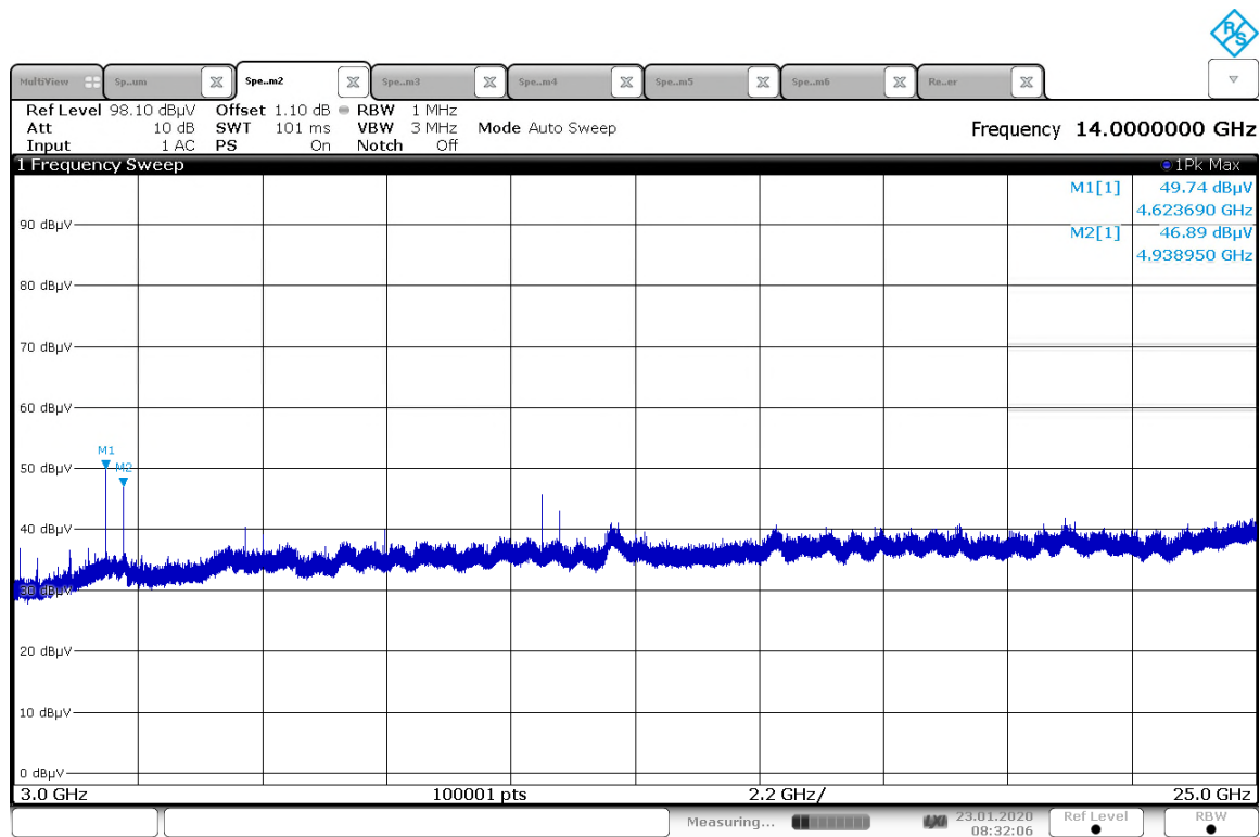
Figure A-11: 3GHz-25GHz (Conducted)
