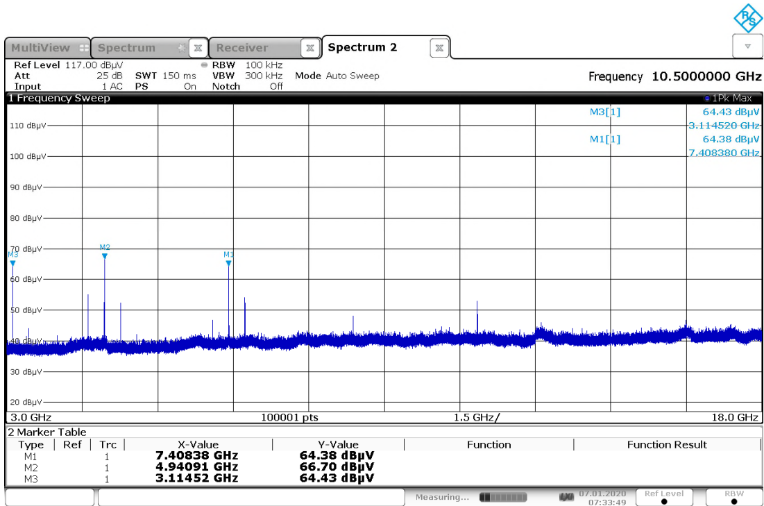
Figure A-5: 3GHz-18GHz (Radiated)
