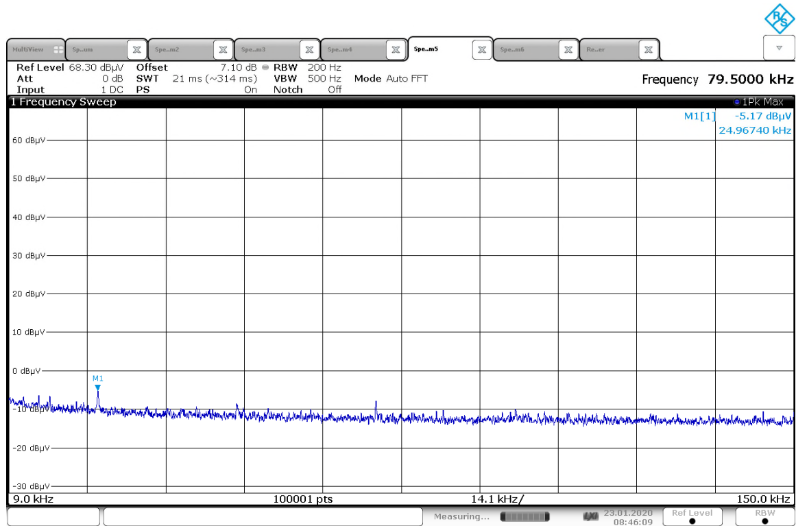
Figure A-7: 9kHz-150kHz (Conducted)
